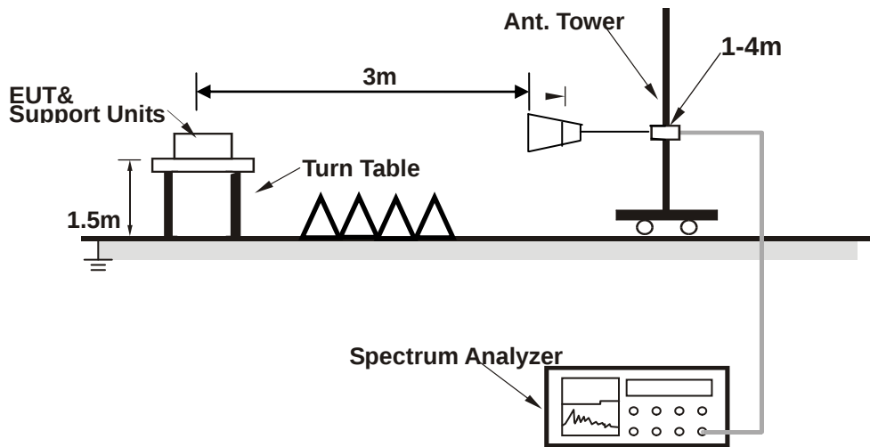
Setup diagram for Radiated (Above1G) Test
