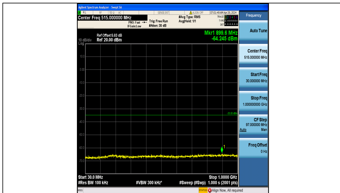
Band7_20MHz_QPSK_20850_100RB#0_30~1000_30~1000
