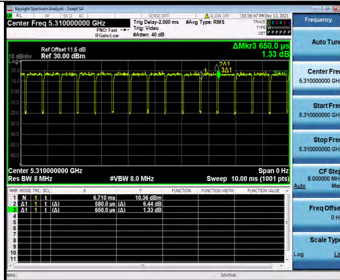
11N40SISO_Ant1_5310
