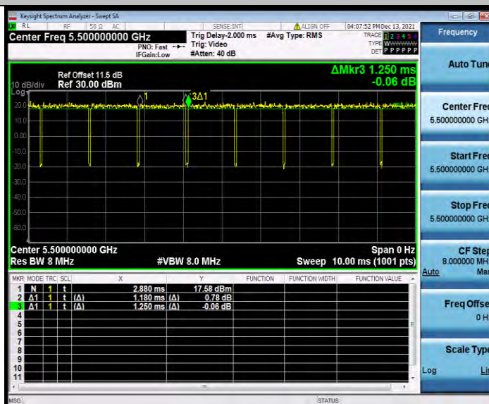
11AC20SISO_Ant1_5500
