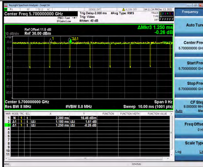
11AC20SISO_Ant1_5700
