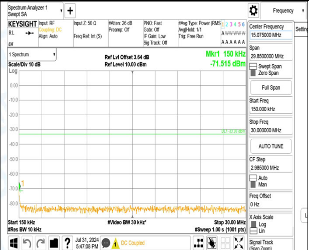
Band2_5MHz_QPSK_19175_1RB#0_1000~3000_1000~3000
