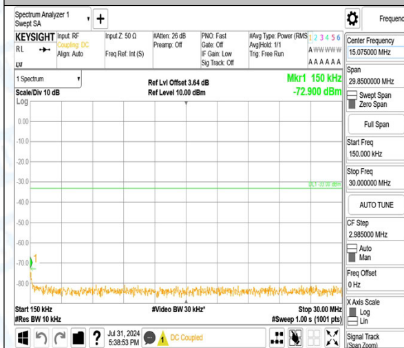
Band2_5MHz_16QAM_18625_25RB#0_0.15~30_0.15~30
