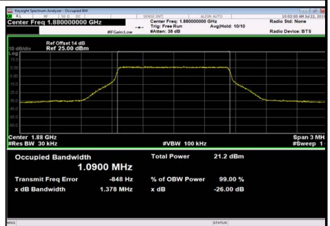
FDD02_MidRange_3_1880_Q16
