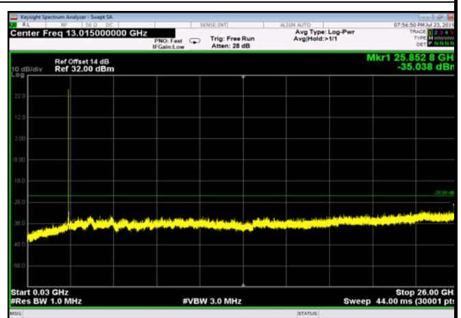
FDD07_LowRange_5MHz_30MHz~26GHz
