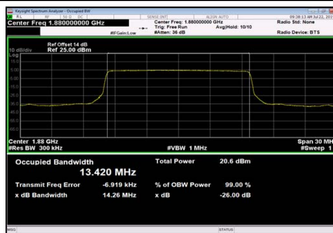
FDD02_MidRange_20MHz_1880MHz_QPSK
