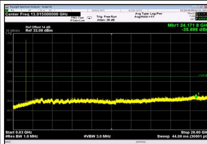
FDD05_HighRange_10MHz_30MHz~26GHz
