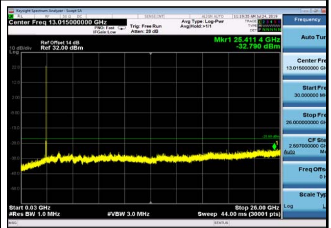
FDD07_MidRange_20MHz_30MHz~26GHz
