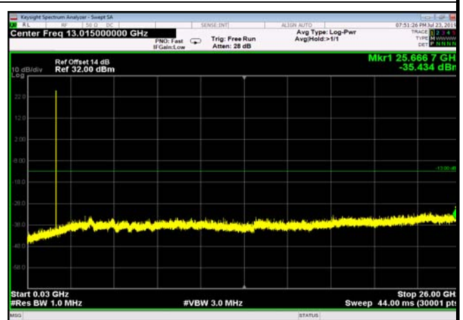
FDD04_HighRange_3MHz_30MHz~26GHz
