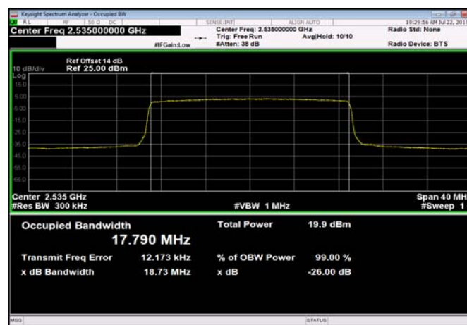
FDD07_MidRange_20_2535_QPSK
