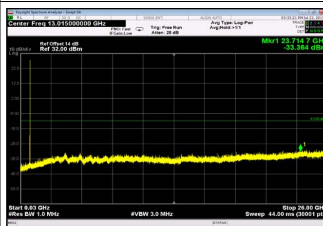
FDD05_LowRange_10MHz_30MHz~26GHz
