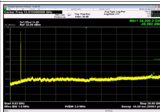
FDD02_LowRange_3MHz_30MHz~26GHz
