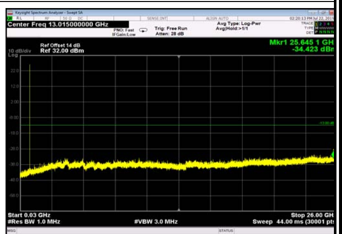
FDD05_LowRange_3MHz_30MHz~26GHz
