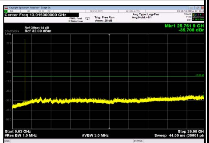
FDD05_HighRange_1.4MHz_30MHz~26GHz
