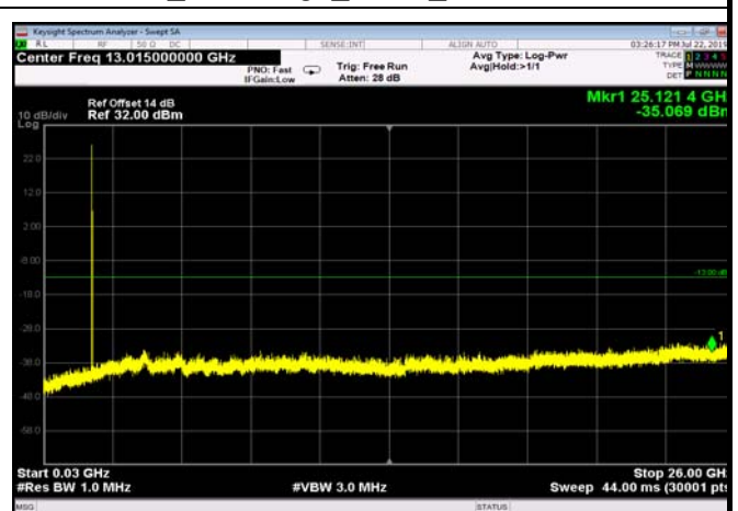
FDD02_LowRange_5MHz_30MHz~26GHz
