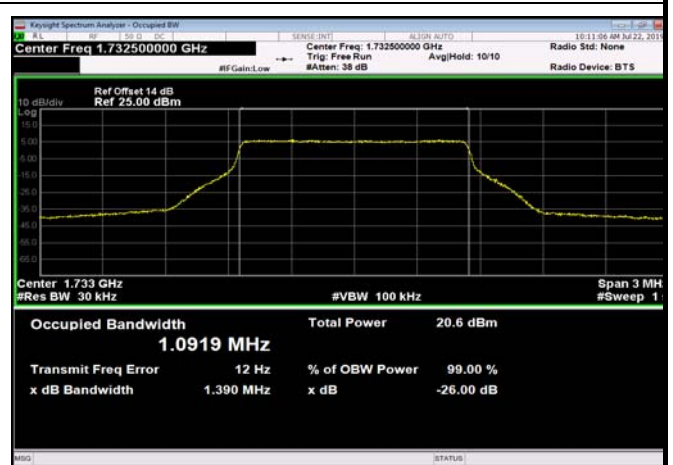
FDD04_MidRange_3_1732.5_Q16
