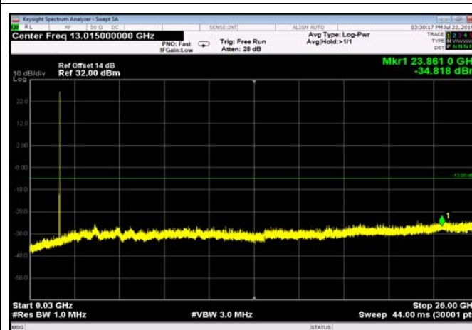
FDD04_HighRange_5MHz_30MHz~26GHz
