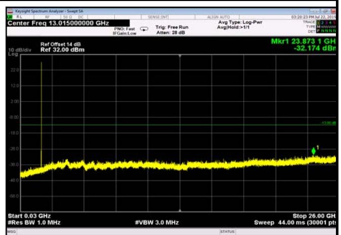
FDD04_LowRange_1.4MHz_30MHz~26GHz
