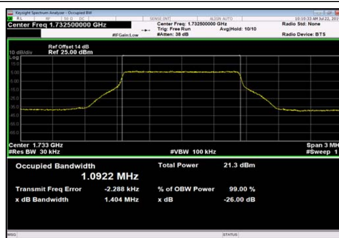
FDD04_MidRange_3_1732.5_QPSK
