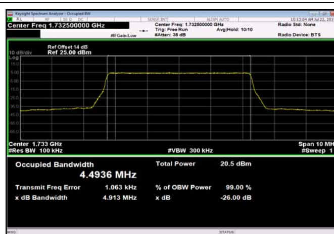
FDD04_MidRange_5_1732.5_QPSK
