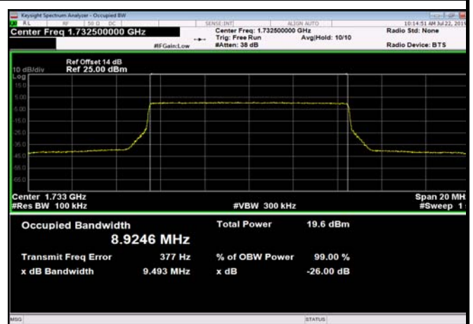
FDD04_MidRange_15_1732.5_Q16
