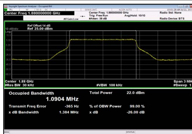
FDD02_MidRange_3_1880_QPSK
