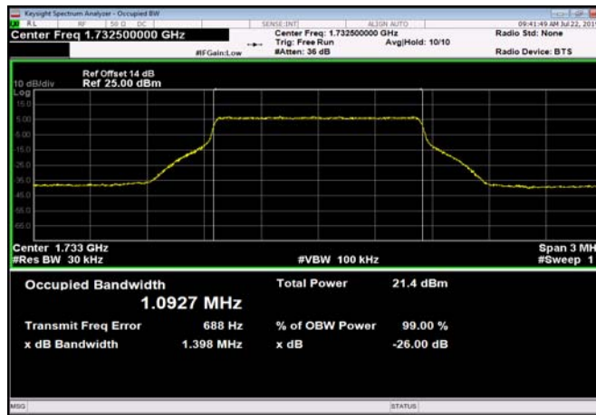
FDD04_MidRange_3MHz_1732.5MHz_QPSK
