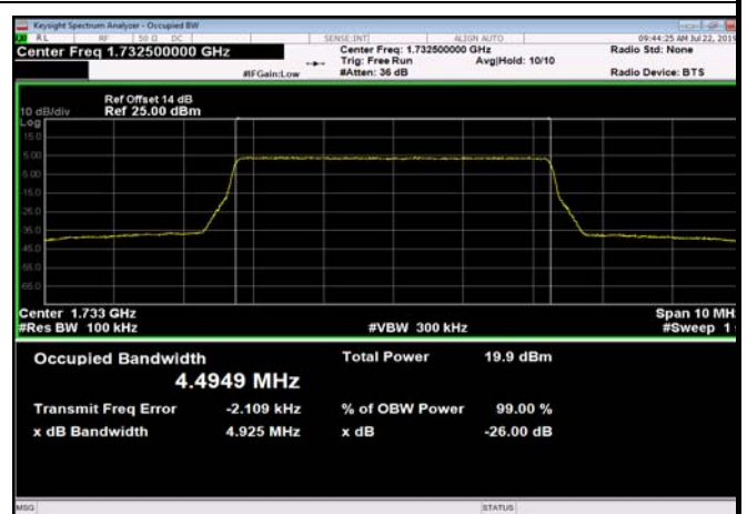
FDD04_MidRange_5MHz_1732.5MHz_Q16
