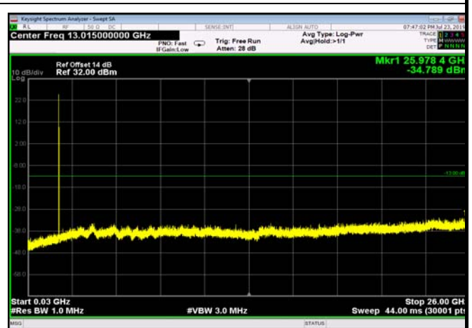
FDD02_LowRange_20MHz_30MHz~26GHz
