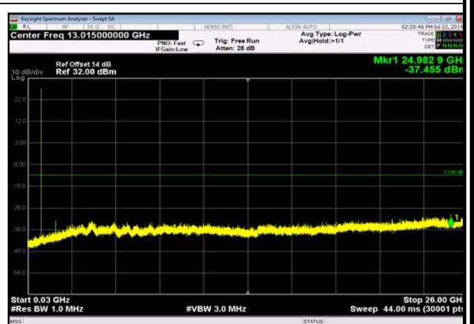
FDD05_MidRange_1.4MHz_30MHz~26GHz
