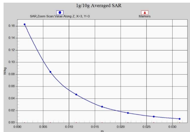
Fig. 1-31 Z-Scan at power reference point (LTE Band41PC2)
