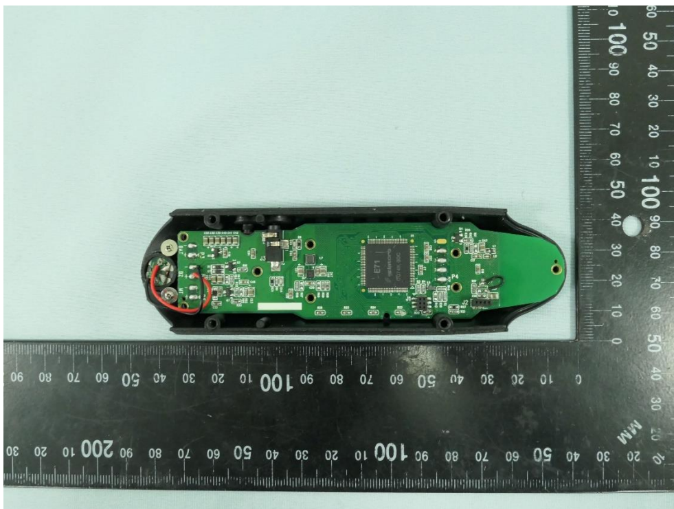
(12) EUT Photo - CP8918TC
