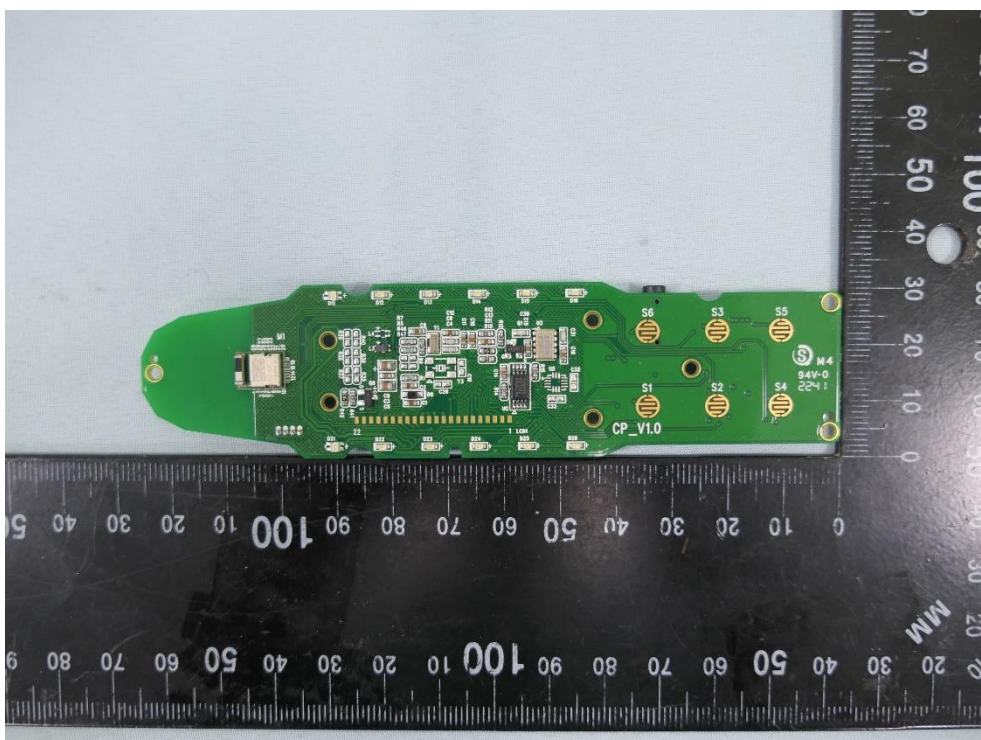
(6) EUT Photo - CP8916TC
