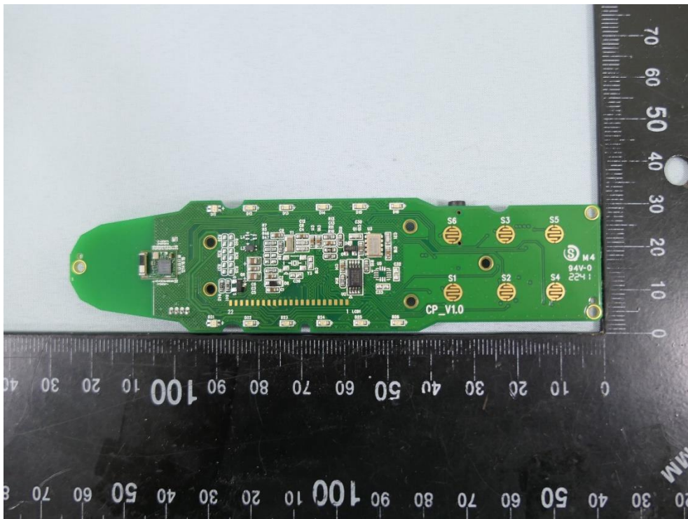
(10) EUT Photo - CP8916TC
