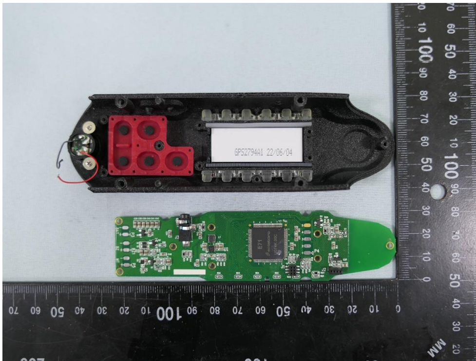
(4) EUT Photo - CP8916TC
