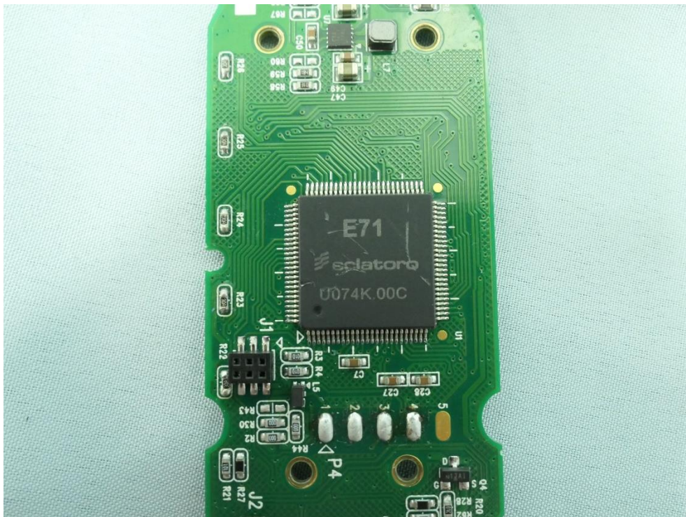
(16) EUT Photo - CP8918TC
