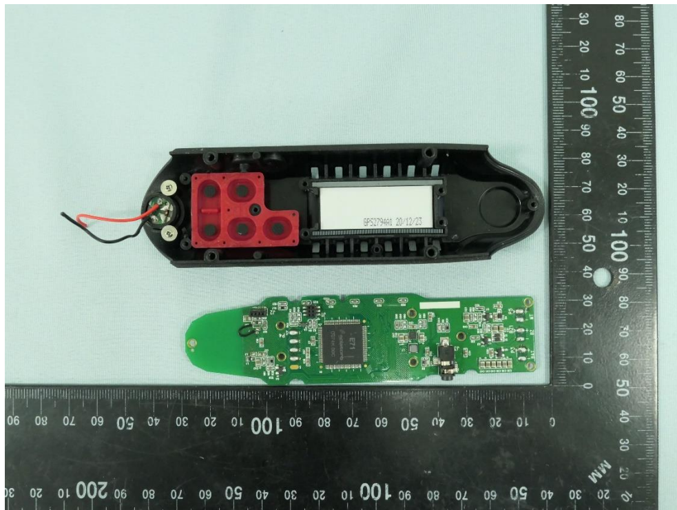
(14) EUT Photo - CP8918TC
