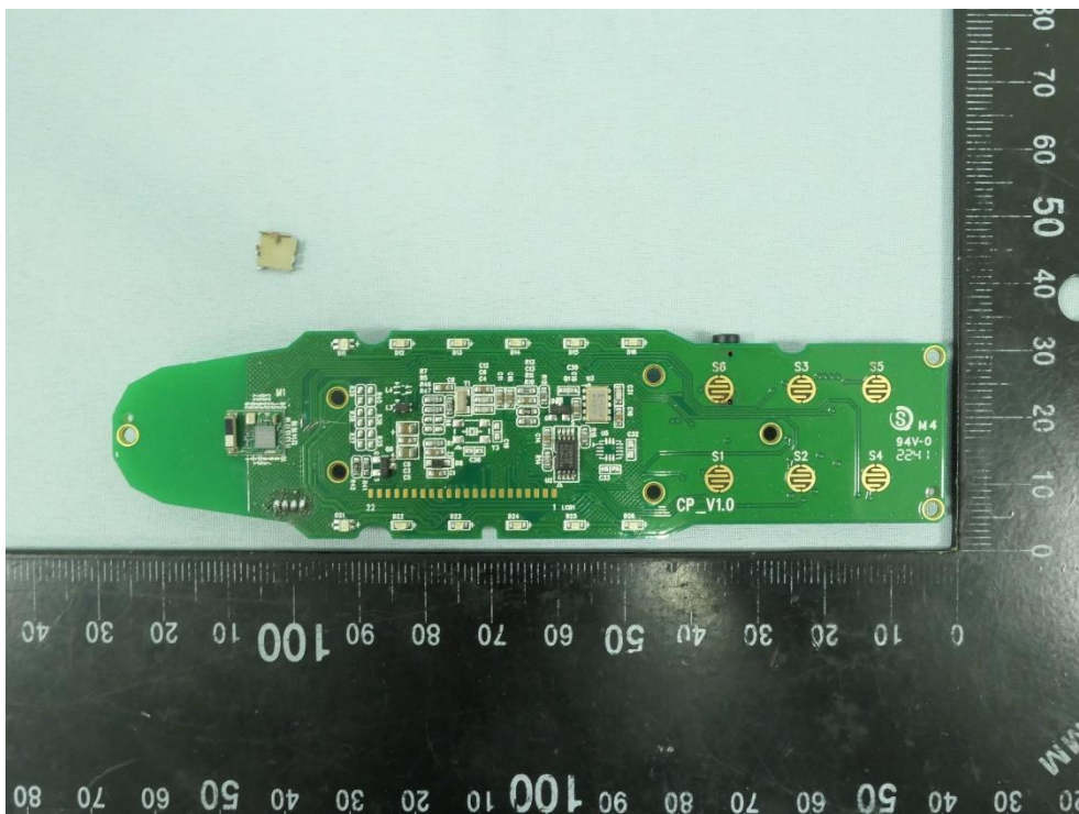
(18) EUT Photo - CP8918TC
