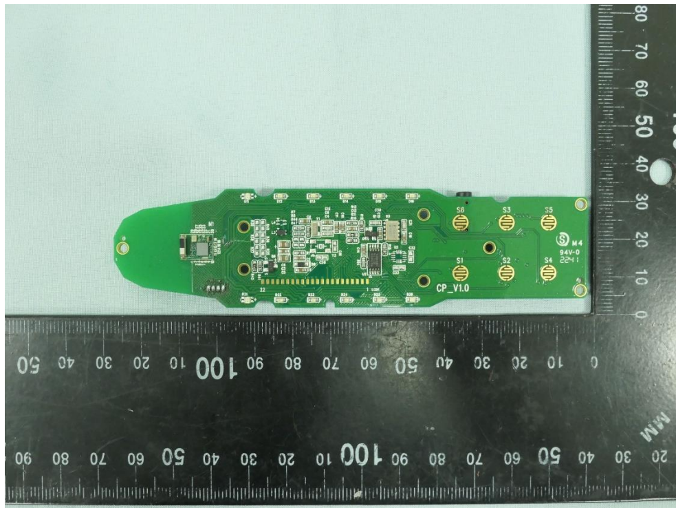
(20) EUT Photo - CP8918TC
