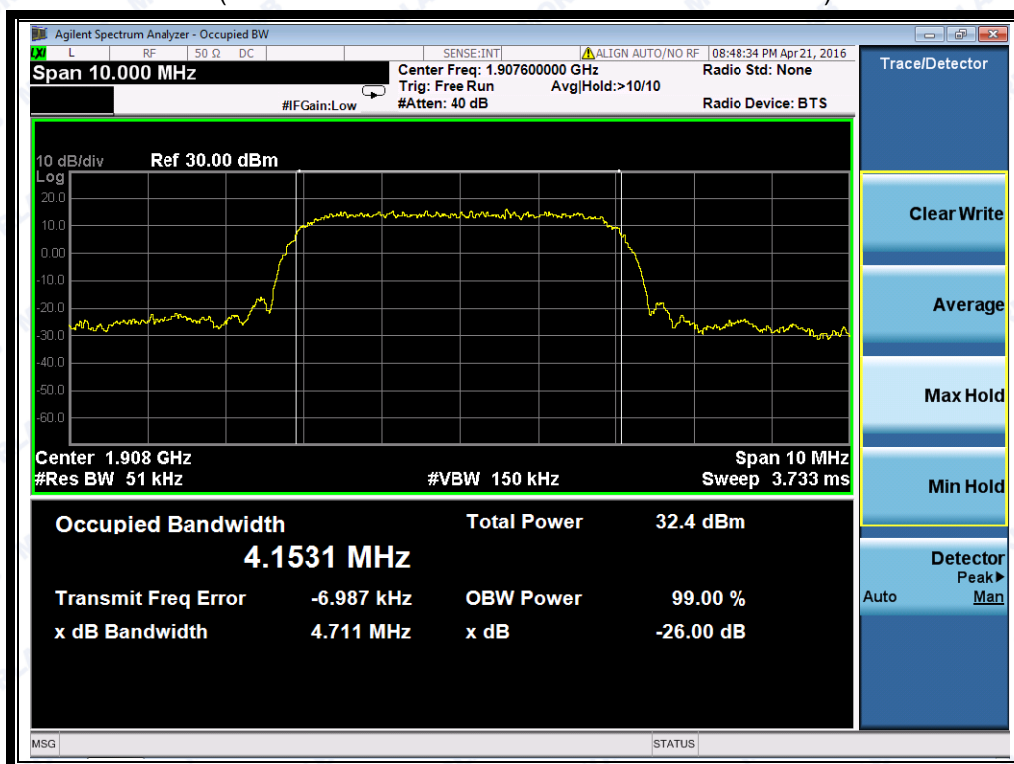
(Plot R3: HSPA+ 1900MHz Channel = 9538)
