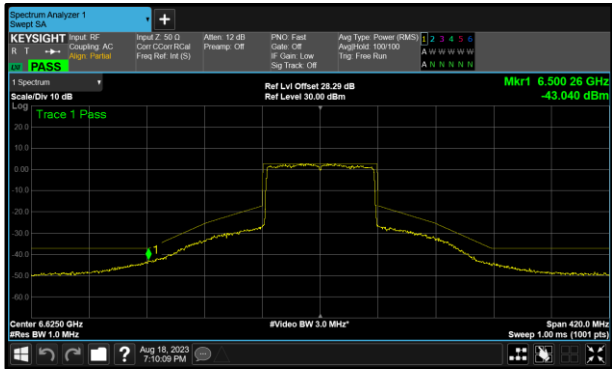
Figure 178 - A (Core 0) 802.11ax HE80 SU SP 6625 MHz (CH135)
