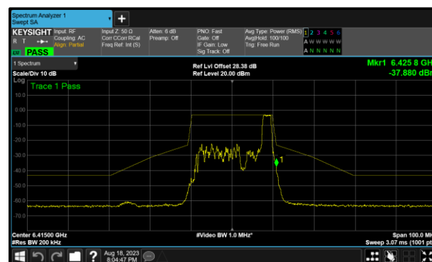
Figure 194 - A (Core 0) 802.11ax HE20 RU26 SP 6415 MHz (CH93)
