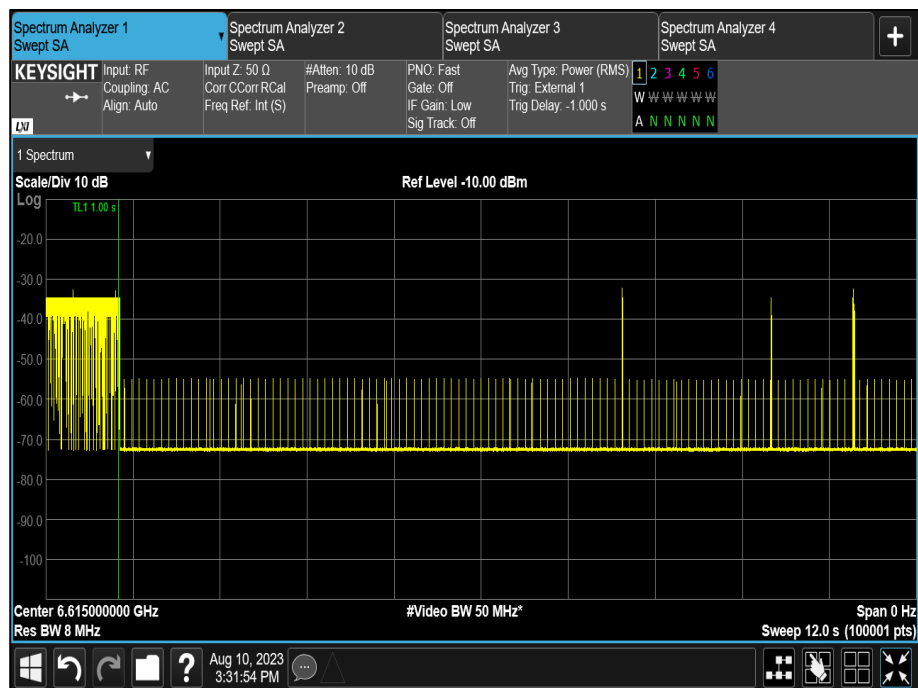
Figure 226 - U-NII-7, Minimum Bandwidth (AWGN Low)
