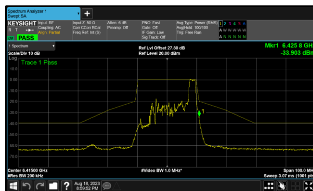
Figure 208 - B (Core 1) 802.11ax HE20 RU26 SP 6415 MHz (CH93)
