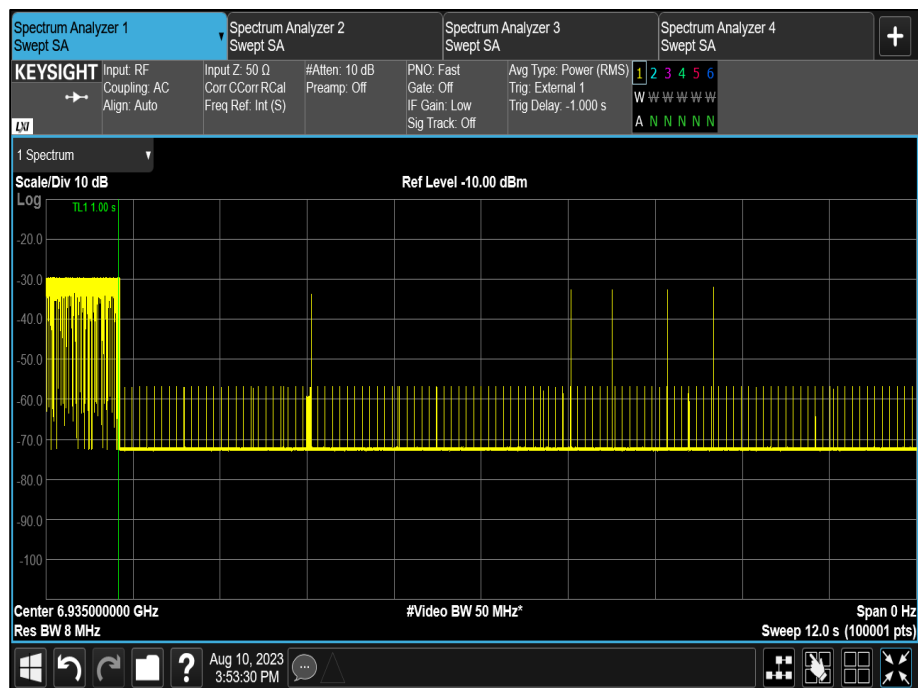
Figure 231 - U-NII-8, Minimum Bandwidth (AWGN Mid)
