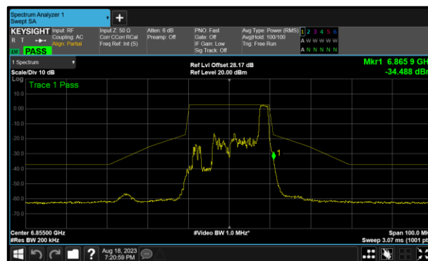
Figure 181 - A (Core 0) 802.11ax HE20 RU26 SP 6855 MHz (CH181)
