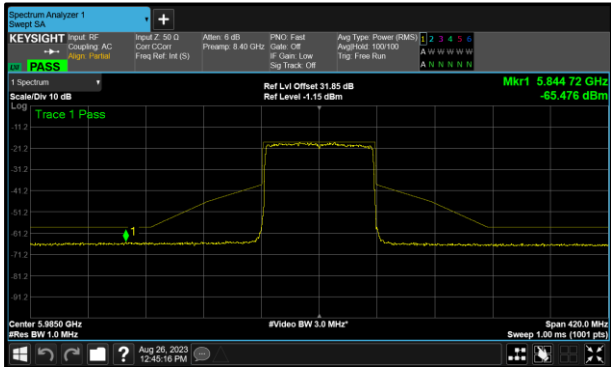
Figure 211 - A (Core 0) 802.11ax HE80 SU LPI 5985 MHz (CH7)
