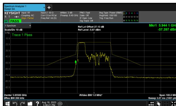
Figure 188 - B (Core 1) 802.11ax HE20 RU52 LPI 5955 MHz (CH1)
