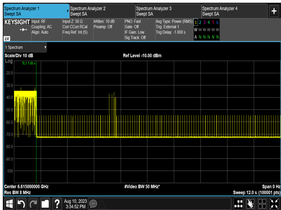
Figure 227 - U-NII-7, Minimum Bandwidth (AWGN Mid)
