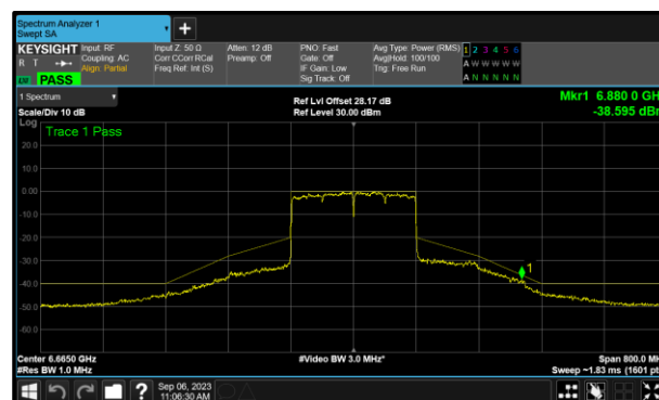
Figure 206 - B (Core 1) 802.11ax HE160 SU SP 6665 MHz (CH143)
