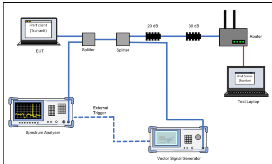
Figure 215 - Test Equipment Setup Diagram
