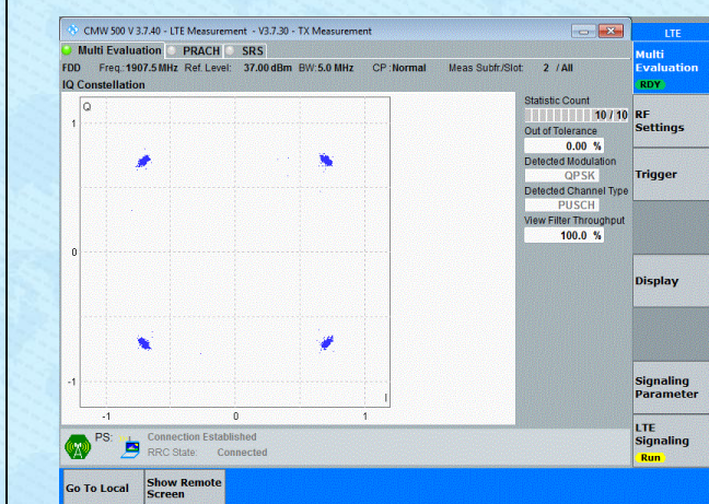
Band2-5MHz-QPSK-19175-25RB#0-PASS
