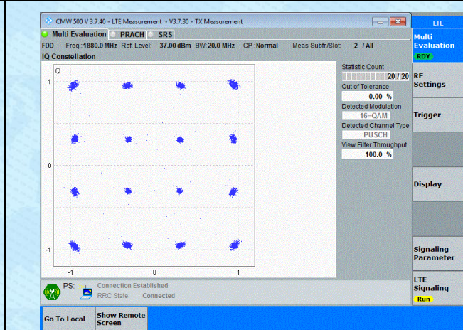
Band2-20MHz-16QAM-18900-100RB#0-PASS
