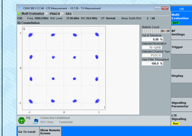
Band2-20MHz-16QAM-19100-100RB#0-PASS
