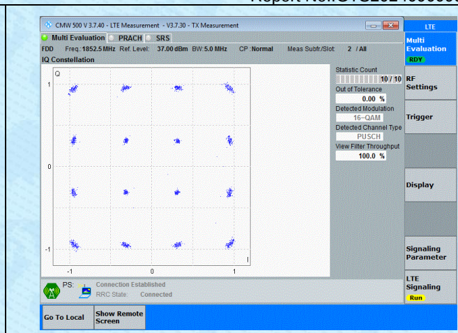
Band2-5MHz-16QAM-18625-25RB#0-PASS
