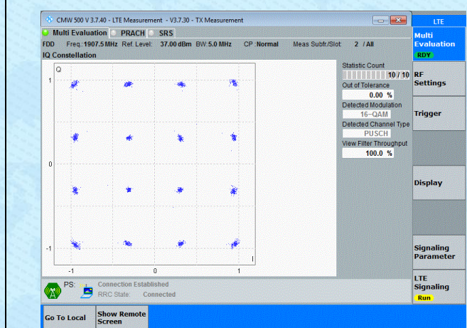
Band2-5MHz-16QAM-19175-25RB#0-PASS
