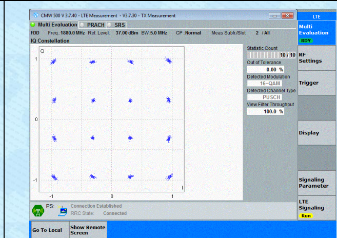
Band2-5MHz-16QAM-18900-25RB#0-PASS
