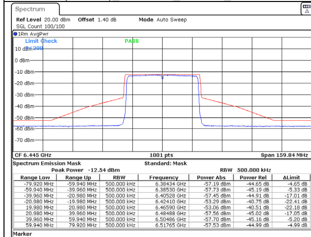
802.11ax (40MHz) 6445MHz Chain A NSS-2
