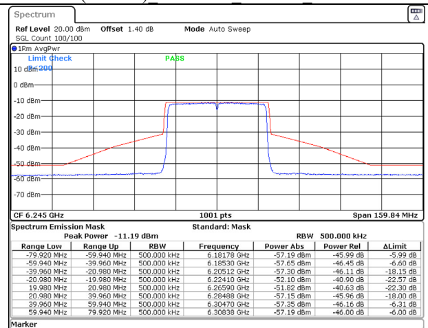
802.11ax (40MHz) 6245MHz Chain B NSS-2
