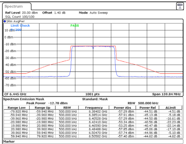
802.11ax (40MHz) 6445MHz Chain D NSS-2
