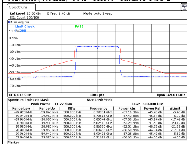
802.11ax (40MHz) 6845MHz Chain C NSS-2
