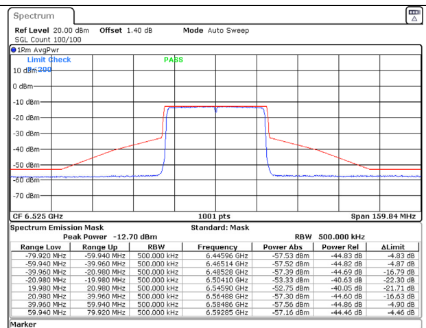
802.11ax (40MHz) 6525MHz Chain B NSS-2
