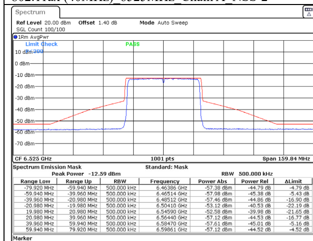
802.11ax (40MHz) 6525MHz Chain C NSS-2
