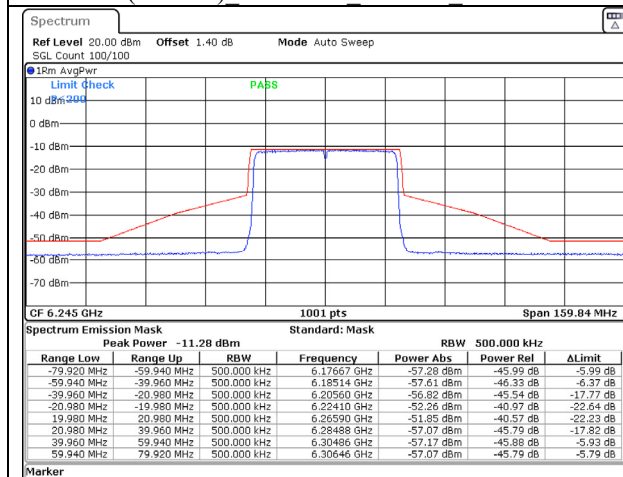
802.11ax (40MHz) 6245MHz Chain A NSS-2
