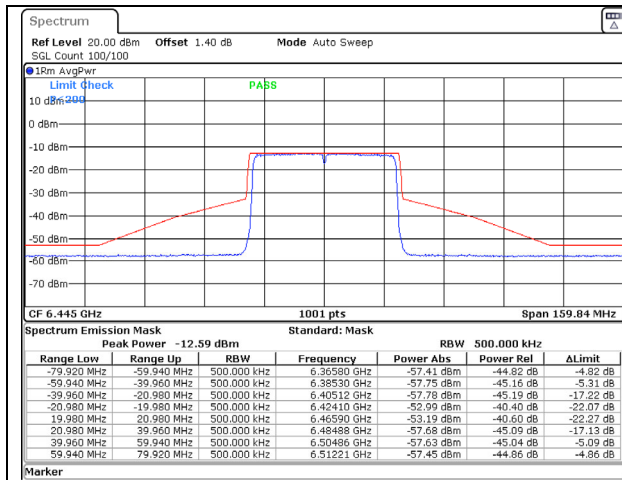
802.11ax (40MHz) 6445MHz Chain C NSS-2
