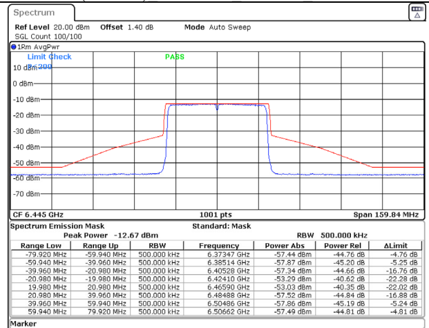
802.11ax (40MHz) 6445MHz Chain B NSS-2
