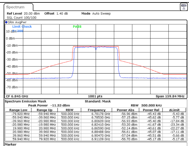
802.11ax (40MHz) 6845MHz Chain B NSS-2
