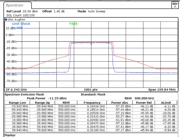
802.11ax (40MHz) 6245MHz Chain D NSS-2
