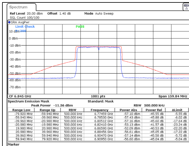
802.11ax (40MHz) 6845 CH179 Chain A NSS-2
