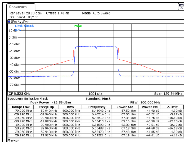
802.11ax (40MHz) 6525MHz Chain A NSS-2
