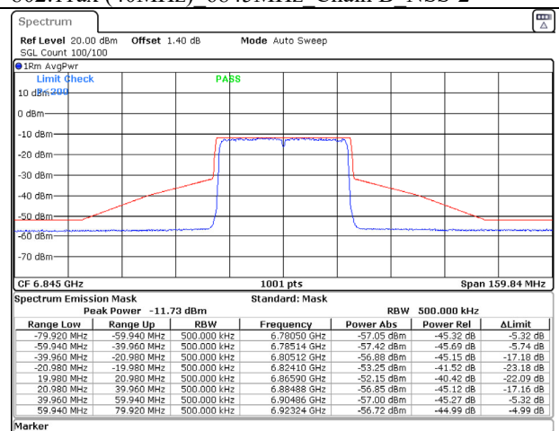
802.11ax (40MHz) 6845MHz Chain D NSS-2
