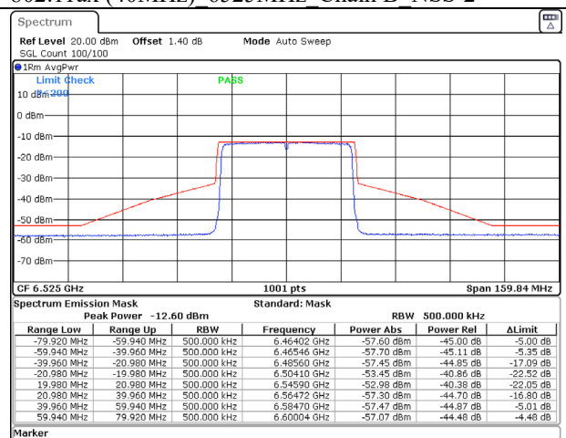
802.11ax (40MHz) 6525MHz Chain D NSS-2
