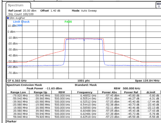
802.11ax (40MHz) 6565MHz Chain A NSS-2
