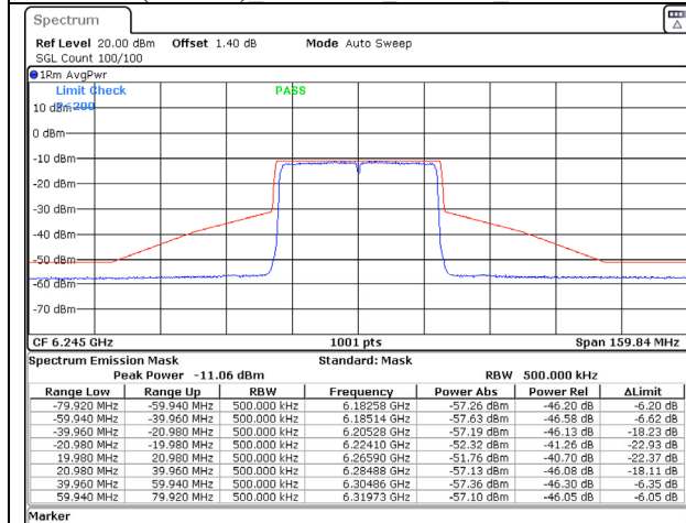
802.11ax (40MHz) 6245MHz Chain C NSS-2
