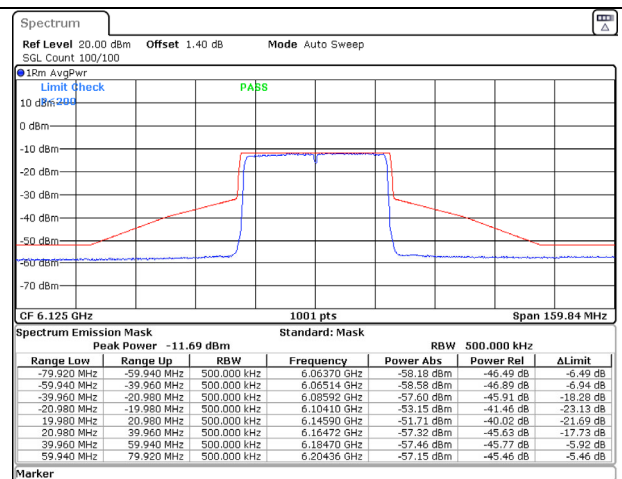
802.11ax (40MHz) 6125MHz Chain D NSS-2
