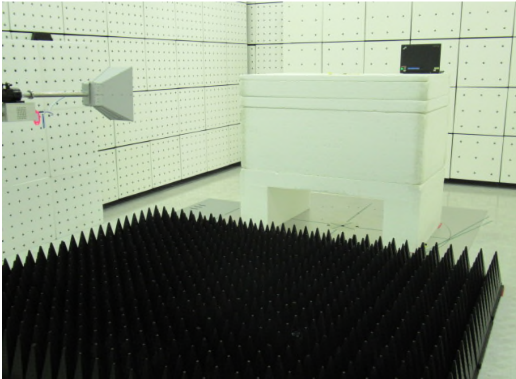
Front View of Set up Photos
