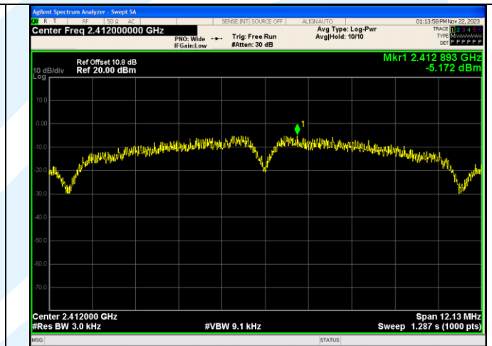
IEEE 802.11b Channel 1 20MHz Antenna 1
