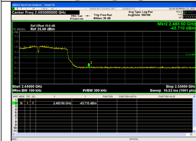
Out Of Band Emission IEEE 802.11n Channel 9 40MHz Antenna 1
