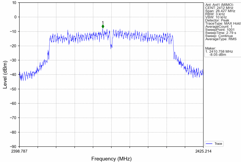
802.11ax(HEW20)_LCH_2412MHz_SU_MIMO_NTNV
