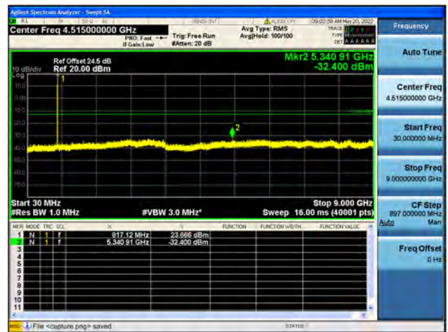
Band26Part90 / 5MHz / Mid CH / 64QAM
