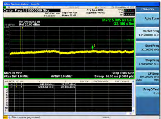
Band26Part90 / 1.4MHz / Mid CH / 64QAM
