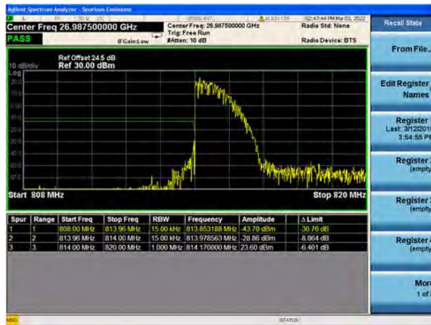
Band26 / 3MHz / Low CH / QPSK / 1 RB
