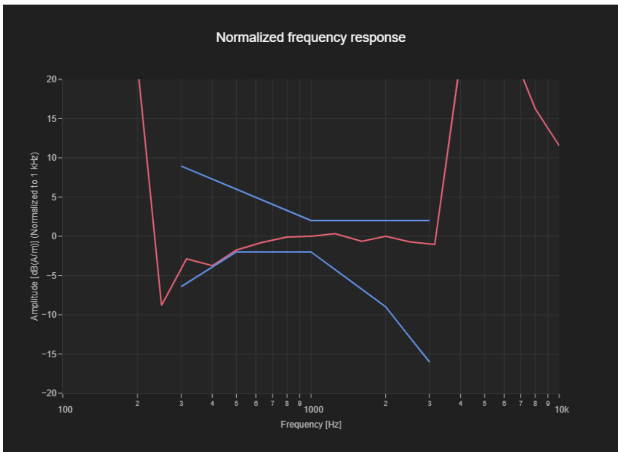
Figure C.4 Frequency Response of NR B48-N5 -OTT
