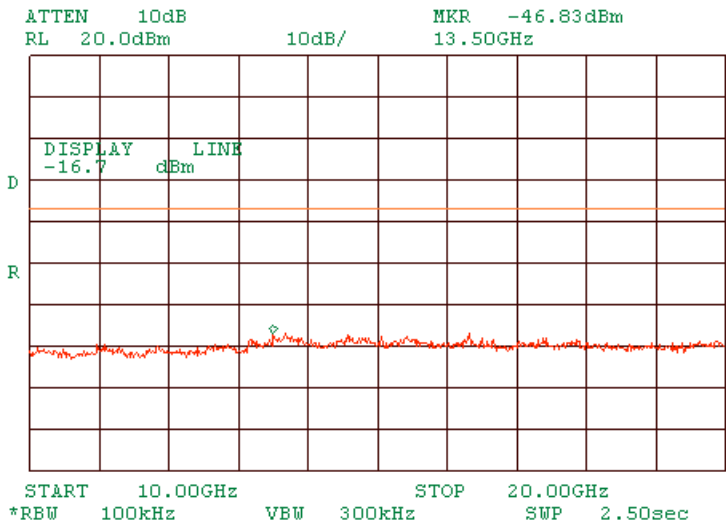
Plot 1.9.55 Spurious emission measurements in 10000 - 20000 MHz range at mid carrier frequency OFDM
