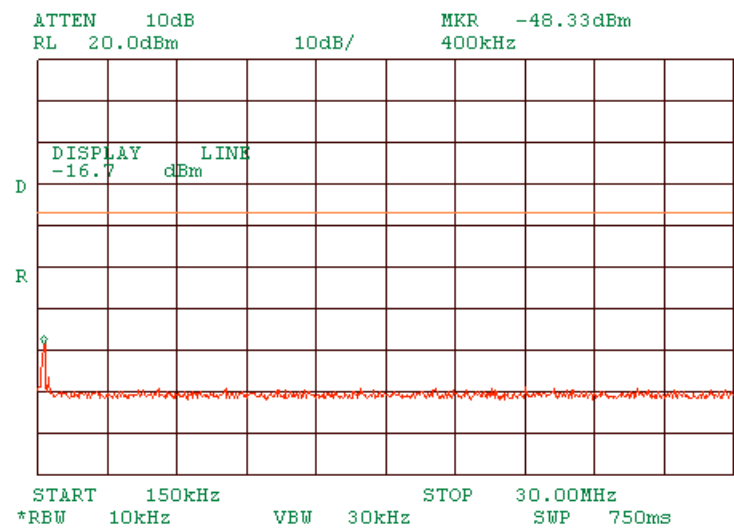
Plot 1.9.36 Spurious emission measurements in 0.15 - 30 MHz range at low carrier frequency OFDM
