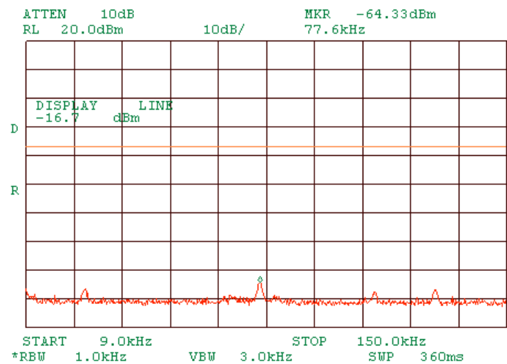
Plot 1.9.35 Spurious emission measurements in 9 - 150 kHz range at high carrier frequency OFDM
