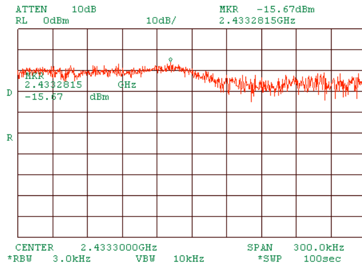
Plot 1.11.26 Peak spectral power density at mid frequency within 6 dB band zoomed at 36 Mbps OFDM
