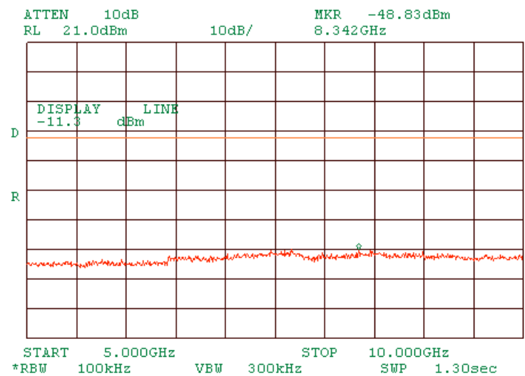
Plot 1.9.22 Spurious emission measurements in 5000 - 10000 MHz range at low carrier frequency DSSS
