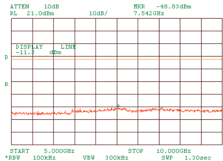
Plot 1.9.23 Spurious emission measurements in 5000 - 10000 MHz range at mid carrier frequency DSSS
