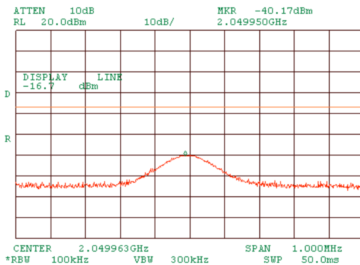
Plot 1.9.46 Zoomed at spurious emission at low carrier frequency OFDM
