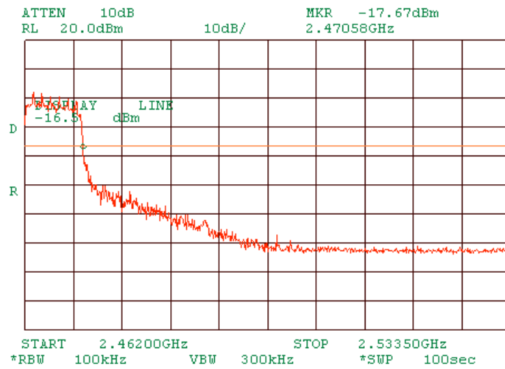
Plot 1.9.61 Band edge measurements at high carrier frequency DSSS
