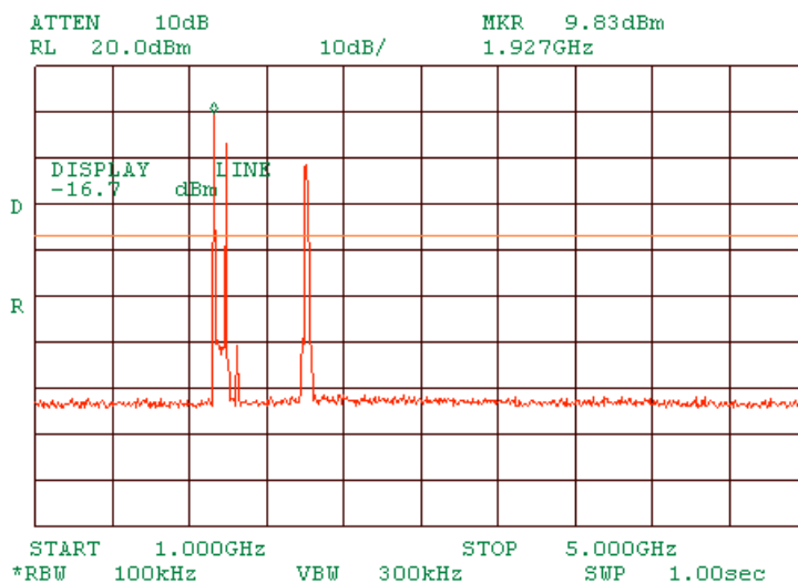
Plot 1.9.45 Spurious emission measurements in 1000 - 5000 MHz range at low carrier frequency OFDM
