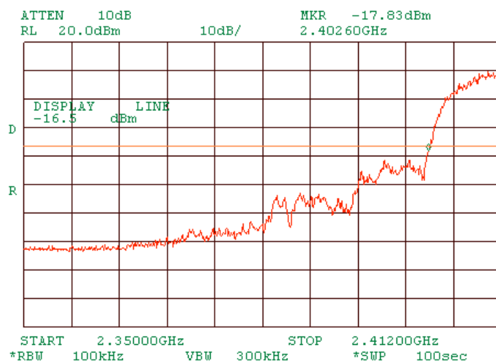
Plot 1.9.28 Band edge measurements at low carrier frequency DSSS
