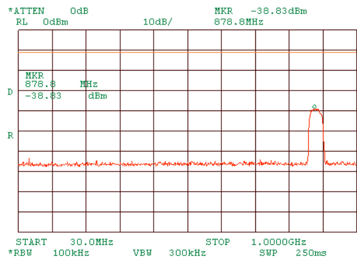
Plot 1.9.12 Spurious emission measurements in 30 - 1000 MHz range at mid carrier frequency DSSS
