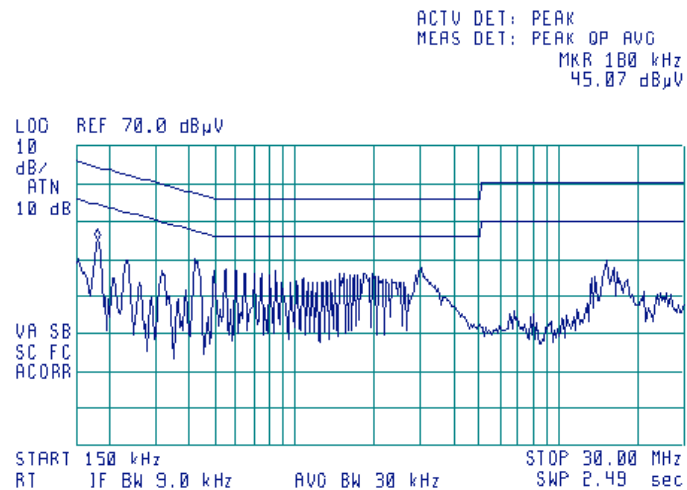
Plot 1.14.4 Conducted emission measurements at MA 1000 port
