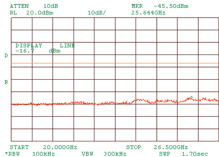
Plot 1.9.59 Spurious emission measurements in 20000 - 26500 MHz range at high carrier frequency OFDM
