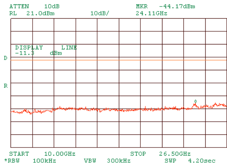
Plot 1.9.26 Spurious emission measurements in 10000 - 26500 MHz range at mid carrier frequency DSSS
