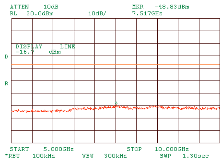
Plot 1.9.53 Spurious emission measurements in 5000 - 10000 MHz range at high carrier frequency OFDM
