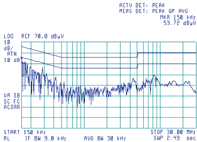
Plot 1.14.8 Conducted emission measurements at Laptop port
