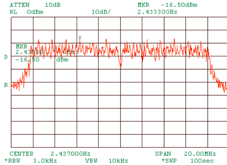
Plot 1.11.25 Peak spectral power density at mid frequency within 6 dB band at 36 Mbps OFDM
