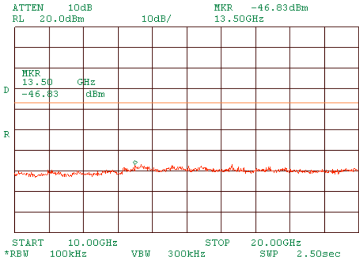
Plot 1.9.56 Spurious emission measurements in 10000 - 20000 MHz range at high carrier frequency OFDM
