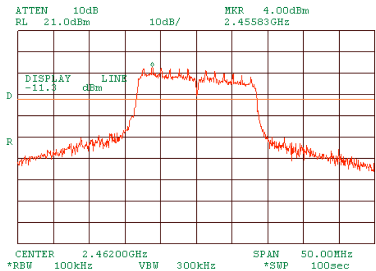
Plot 1.9.32 The highest emission level within the assigned band at high carrier frequency OFDM
