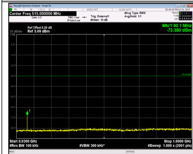
41-41-20MHz-20MHz-64QAM-64QAM-41292-41490-1RB #0-1RB#99-30~1000MHz-PASS
