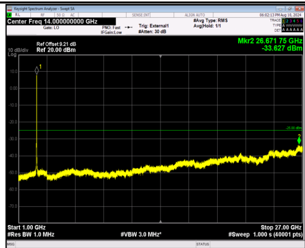
41-41-20MHz-20MHz-16QAM-16QAM-41292-41490-100RB #0-100RB#0-1000~27000MHz-PASS
