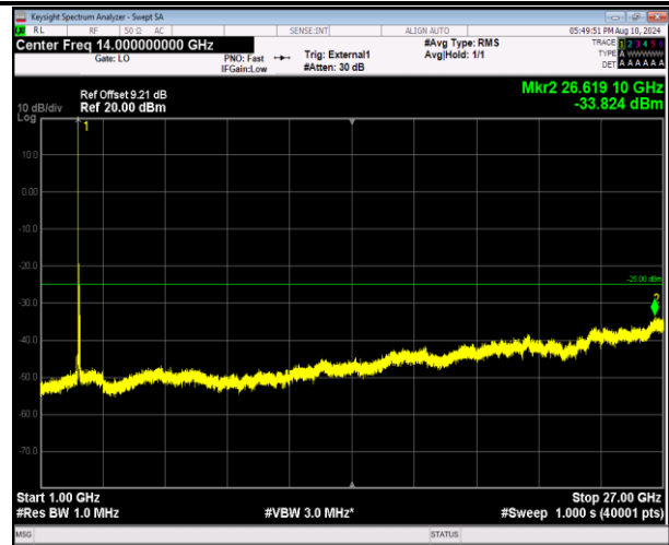
41-41-20MHz-20MHz-16QAM-16QAM-40521-40719-1RB#0 -ORB#0-1000~27000MHz-PASS
