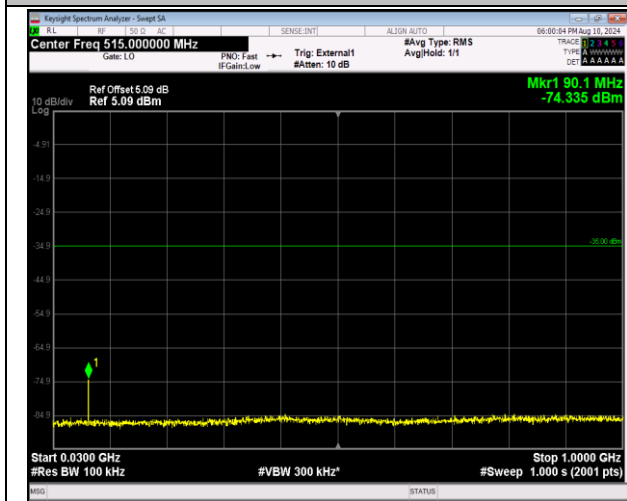
41-41-20MHz-20MHz-16QAM-16QAM-41292-41490-1RB #0-1RB#99-30~1000MHz-PASS
