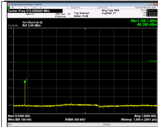
41-41-20MHz-20MHz-64QAM-64QAM-41292-41490-1RB #99-0RB#0-30~1000MHz-PASS
