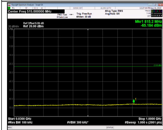
66-66-5MHz-20MHz-64QAM-64QAM-132005-132122-1R B#0-0RB#0-30~1000MHz-PASS
