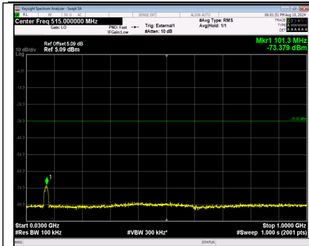
41-41-20MHz-20MHz-16QAM-16QAM-41292-41490-100 RB#0-100RB#0-30~1000MHz-PASS
