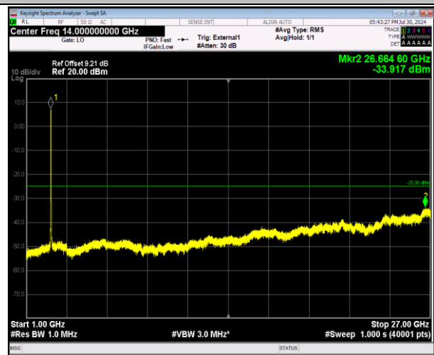
41-41-20MHz-20MHz-64QAM-64QAM-40521-40719-100RB #0-100RB#0-1000~27000MHz-PASS
