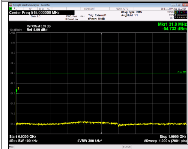
41-41-20MHz-20MHz-16QAM-16QAM-40521-40719-1RB #99-ORB#0-30~1000MHz-PASS
