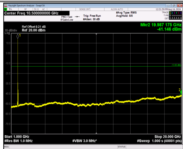
66-66-5MHz-20MHz-64QAM-64QAM-132330-132447-1RB# 0-1RB#99-1000~20000MHz-PASS
