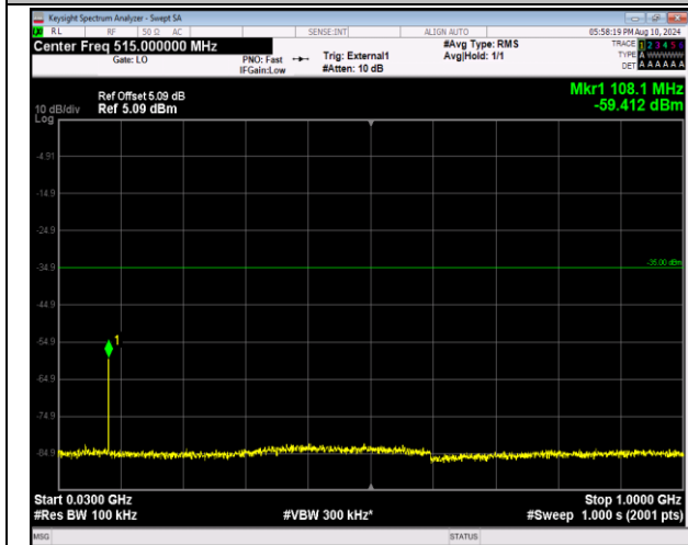
41-41-20MHz-20MHz-16QAM-16QAM-41292-41490-1RB #99-ORB#0-30~1000MHz-PASS
