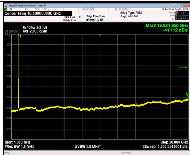
66-66-5MHz-20MHz-16QAM-16QAM-132330-132447-1RB# 0-0RB#0-1000~20000MHz-PASS
