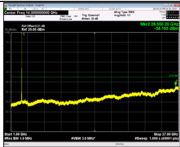
41-41-20MHz-20MHz-64QAM-64QAM-41292-41490-1RB#9 9-0RB#0-1000~27000MHz-PASS
