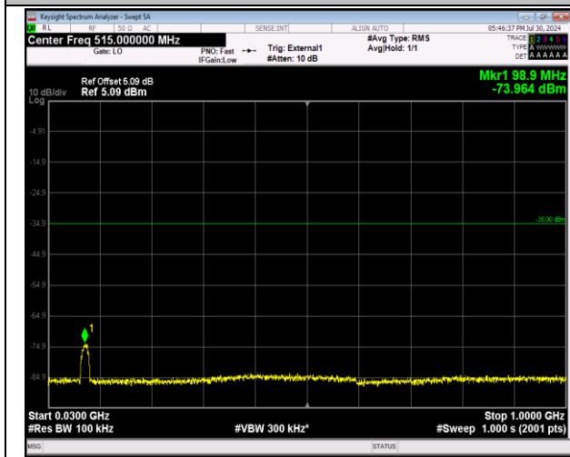
41-41-20MHz-20MHz-64QAM-64QAM-41292-41490-100 RB#0-100RB#0-30~1000MHz-PASS
