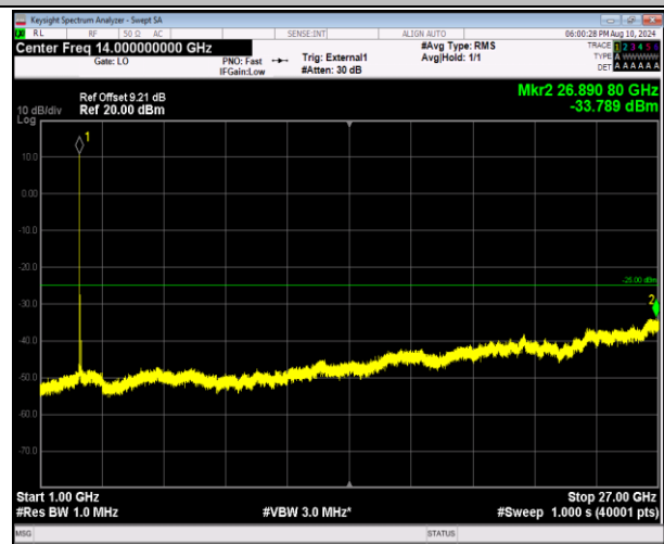
41-41-20MHz-20MHz-16QAM-16QAM-41292-41490-1RB#0 -1RB#99-1000~27000MHz-PASS
