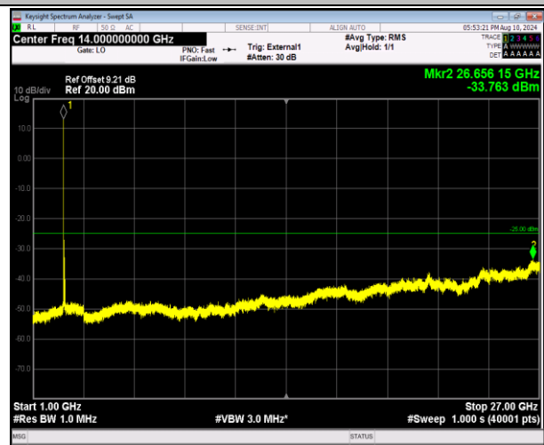
41-41-20MHz-20MHz-16QAM-16QAM-40521-40719-1RB#0 -1RB#99-1000~27000MHz-PASS
