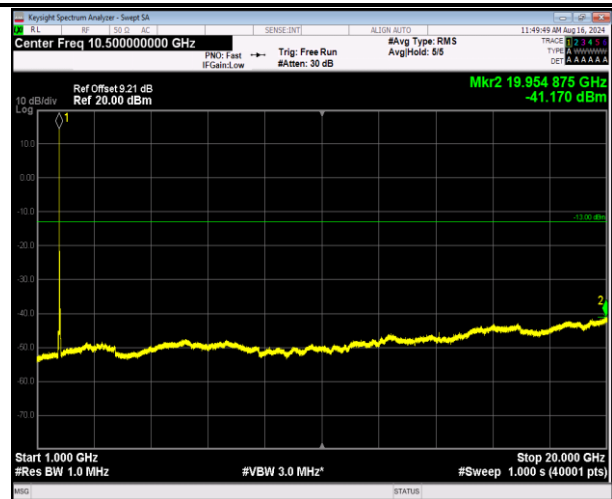
66-66-5MHz-20MHz-16QAM-16QAM-132330-132447-25RB #0-100RB#0-1000~20000MHz-PASS
