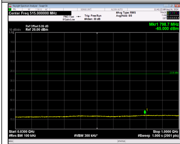
66-66-5MHz-20MHz-QPSK-QPSK-132005-132122-1RB# 24-0RB#0-30~1000MHz-PASS
