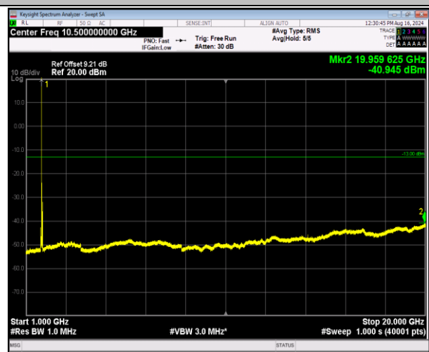
66-66-5MHz-20MHz-64QAM-64QAM-132330-132447-1RB# 0-0RB#0-1000~20000MHz-PASS
