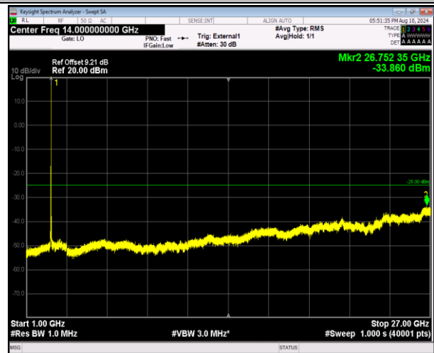
41-41-20MHz-20MHz-16QAM-16QAM-40521-40719-1RB#9 9-ORB#0-1000~27000MHz-PASS
