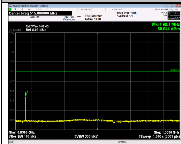
41-41-20MHz-20MHz-64QAM-64QAM-41292-41490-1RB #0-0RB#0-30~1000MHz-PASS
