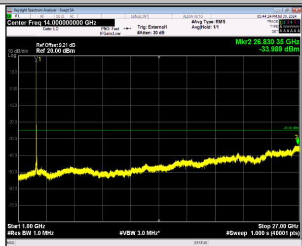
41-41-20MHz-20MHz-64QAM-64QAM-41292-41490-1RB#0 -0RB#0-1000~27000MHz-PASS
