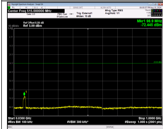
41-41-20MHz-20MHz-QPSK-QPSK-41292-41490-100RB #0-100RB#0-30~1000MHz-PASS
