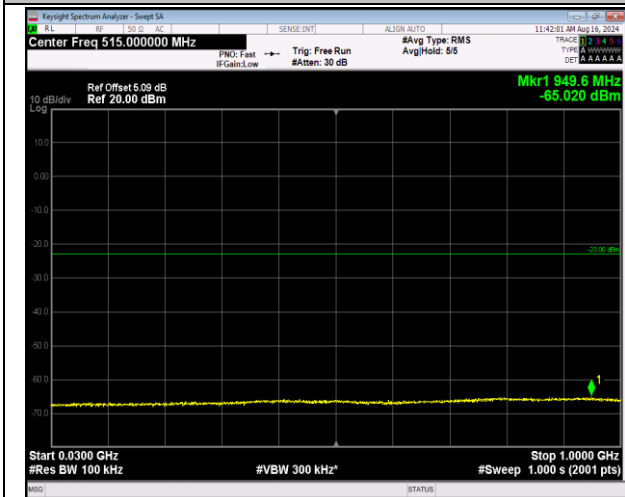
66-66-5MHz-20MHz-16QAM-16QAM-132005-132122-1R B#24-ORB#0-30~1000MHz-PASS
