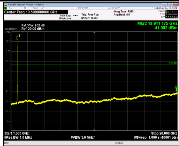
66-66-5MHz-20MHz-16QAM-16QAM-132005-132122-25RB #0-100RB#0-1000~20000MHz-PASS
