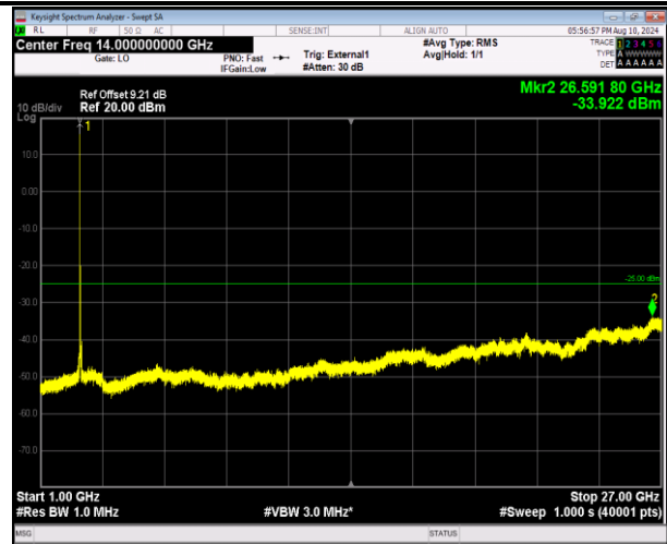
41-41-20MHz-20MHz-16QAM-16QAM-41292-41490-1RB#0 -ORB#0-1000~27000MHz-PASS
