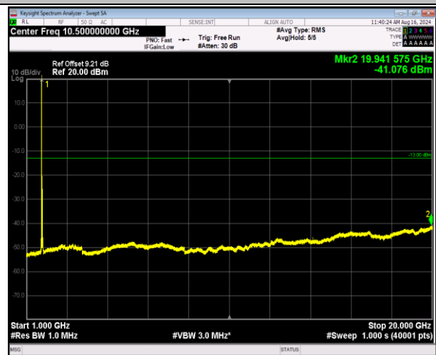
66-66-5MHz-20MHz-QPSK-QPSK-132005-132122-1RB#0- ORB#0-1000~20000MHz-PASS
