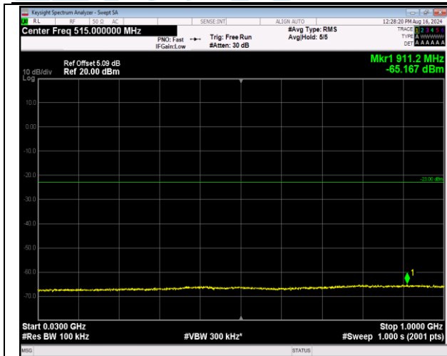
66-66-5MHz-20MHz-64QAM-64QAM-132005-132122-1R B#24-ORB#0-30~1000MHz-PASS
