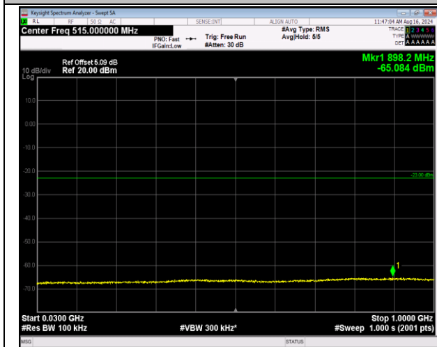
66-66-5MHz-20MHz-16QAM-16QAM-132330-132447-1R B#24-0RB#0-30~1000MHz-PASS
