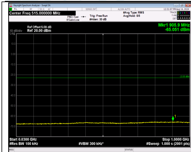
66-66-5MHz-20MHz-64QAM-64QAM-132330-132447-1R B#24-ORB#0-30~1000MHz-PASS
