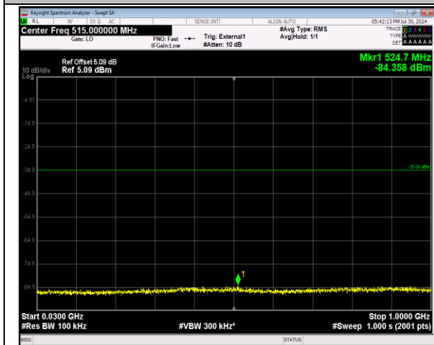
41-41-20MHz-20MHz-64QAM-64QAM-40521-40719-1RB #0-1RB#99-30~1000MHz-PASS
