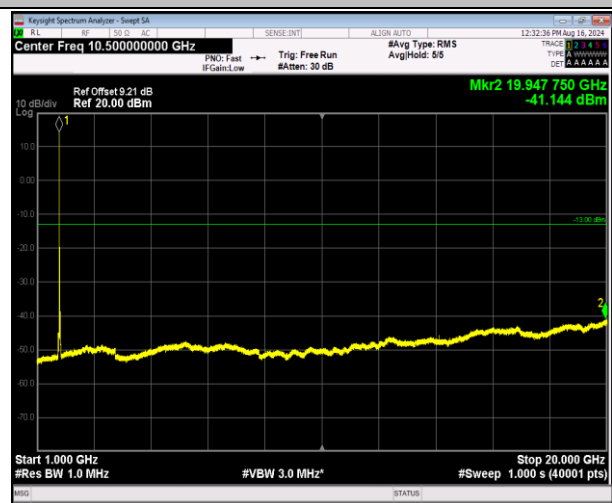
66-66-5MHz-20MHz-64QAM-64QAM-132330-132447-25RB #0-100RB#0-1000~20000MHz-PASS
