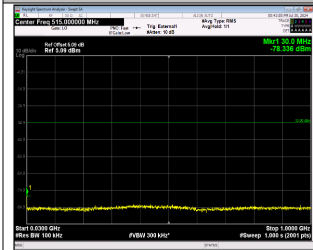
41-41-20MHz-20MHz-64QAM-64QAM-40521-40719-100 RB#0-100RB#0-30~1000MHz-PASS
