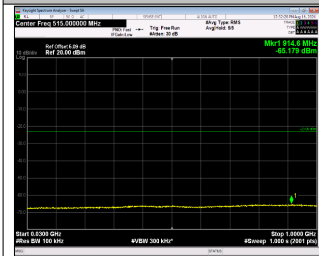
66-66-5MHz-20MHz-64QAM-64QAM-132330-132447-25 RB#0-100RB#0-30~1000MHz-PASS
