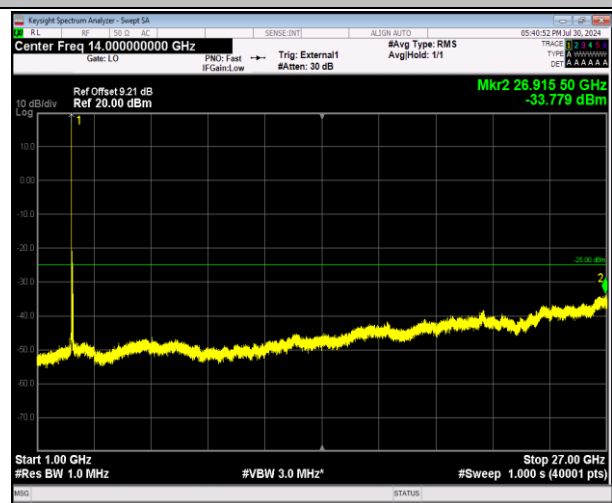
41-41-20MHz-20MHz-64QAM-64QAM-40521-40719-1RB#0 -0RB#0-1000~27000MHz-PASS
