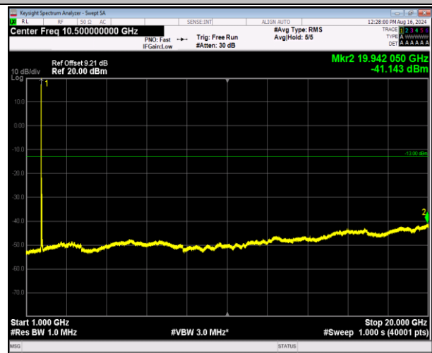
66-66-5MHz-20MHz-64QAM-64QAM-132005-132122-1RB# 0-0RB#0-1000~20000MHz-PASS
