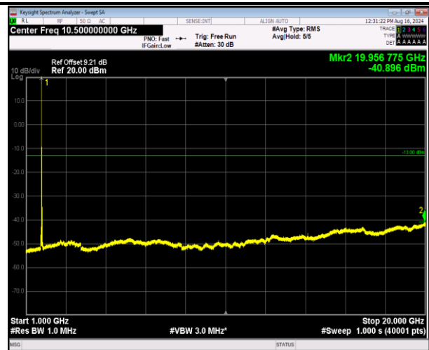
66-66-5MHz-20MHz-64QAM-64QAM-132330-132447-1RB# 24-ORB#0-1000~20000MHz-PASS
