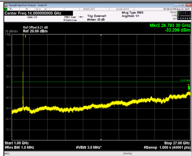
41-41-20MHz-20MHz-16QAM-16QAM-41292-41490-1RB#9 9-ORB#0-1000~27000MHz-PASS
