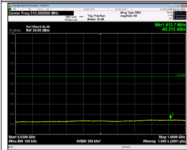
66-66-5MHz-20MHz-16QAM-16QAM-132005-132122-1R B#0-1RB#99-30~1000MHz-PASS
