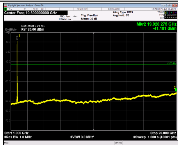
66-66-5MHz-20MHz-64QAM-64QAM-132005-132122-1RB# 0-1RB#99-1000~20000MHz-PASS
