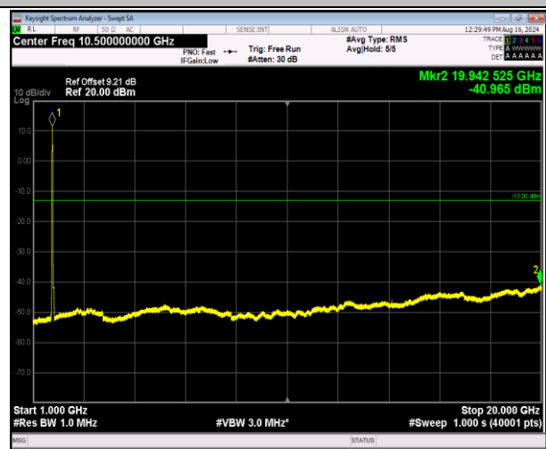
66-66-5MHz-20MHz-64QAM-64QAM-132005-132122-25RB #0-100RB#0-1000~20000MHz-PASS
