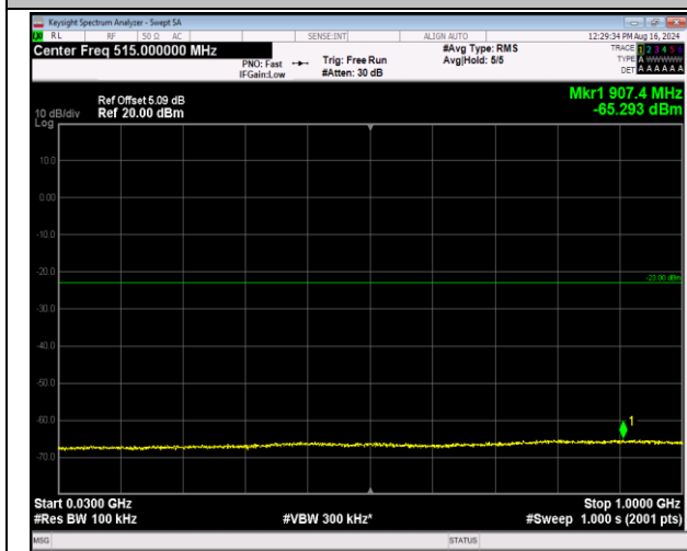
66-66-5MHz-20MHz-64QAM-64QAM-132005-132122-25 RB#0-100RB#0-30~1000MHz-PASS
