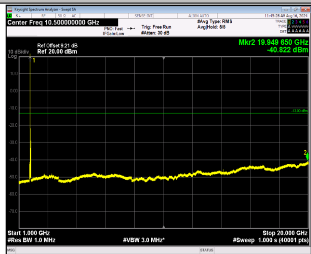
66-66-5MHz-20MHz-QPSK-QPSK-132330-132447-1RB#0- ORB#0-1000~20000MHz-PASS
