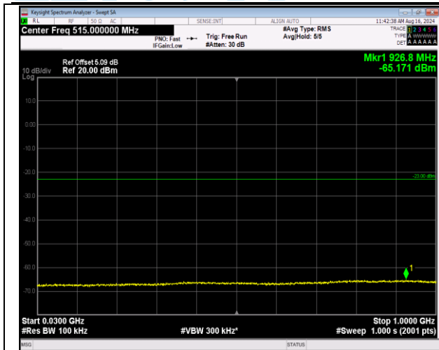
66-66-5MHz-20MHz-QPSK-QPSK-132005-132122-1RB# 0-1RB#99-30~1000MHz-PASS
