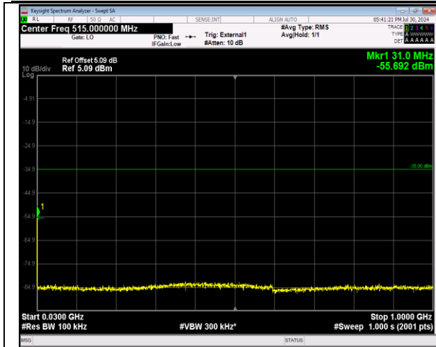
41-41-20MHz-20MHz-64QAM-64QAM-40521-40719-1RB #99-0RB#0-30~1000MHz-PASS
