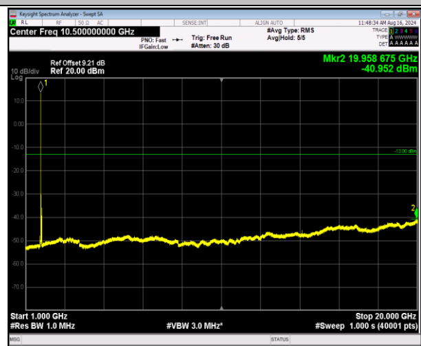
66-66-5MHz-20MHz-16QAM-16QAM-132330-132447-1RB# 0-1RB#99-1000~20000MHz-PASS
