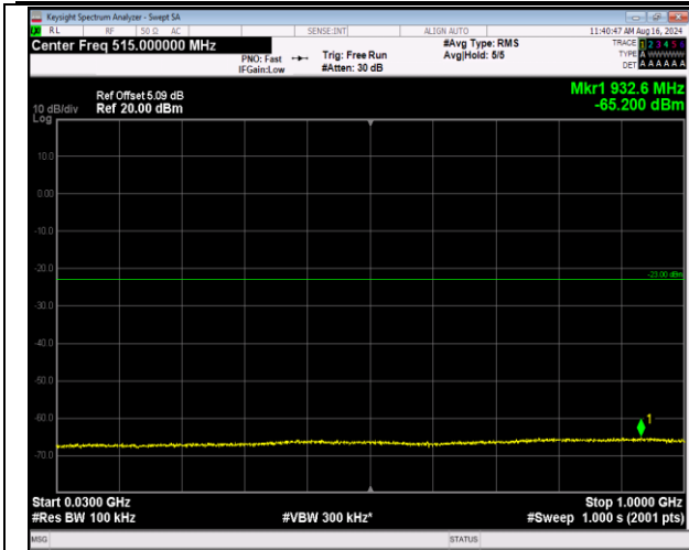
66-66-5MHz-20MHz-16QAM-16QAM-132005-132122-1R B#0-ORB#0-30~1000MHz-PASS
