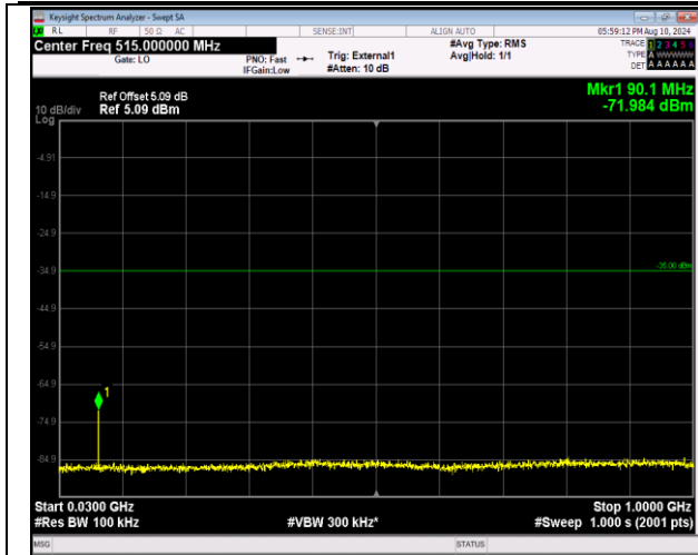
41-41-20MHz-20MHz-QPSK-QPSK-41292-41490-1RB#0 -1RB#99-30~1000MHz-PASS
