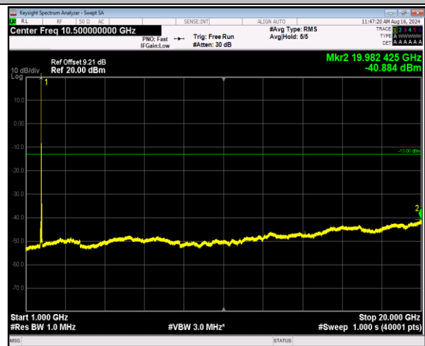
66-66-5MHz-20MHz-16QAM-16QAM-132330-132447-1RB# 24-0RB#0-1000~20000MHz-PASS
