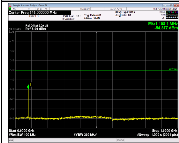
41-41-20MHz-20MHz-QPSK-QPSK-41292-41490-1RB#9 9-0RB#0-30~1000MHz-PASS
