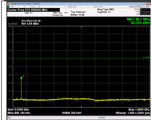
41-41-20MHz-20MHz-16QAM-16QAM-41292-41490-1RB #0-ORB#0-30~1000MHz-PASS
