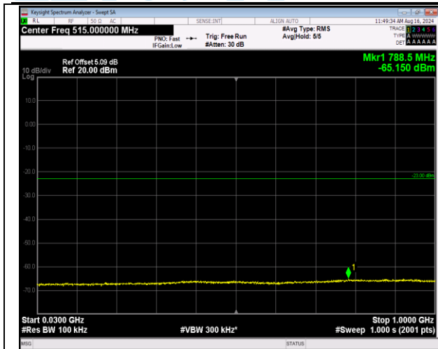
66-66-5MHz-20MHz-16QAM-16QAM-132330-132447-25 RB#0-100RB#0-30~1000MHz-PASS
