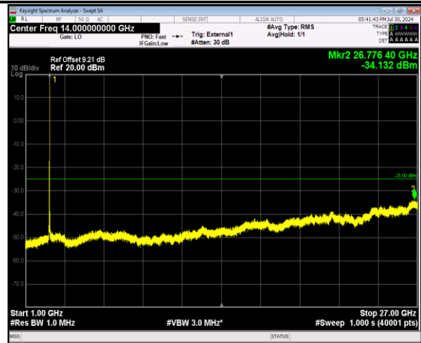
41-41-20MHz-20MHz-64QAM-64QAM-40521-40719-1RB#9 9-0RB#0-1000~27000MHz-PASS
