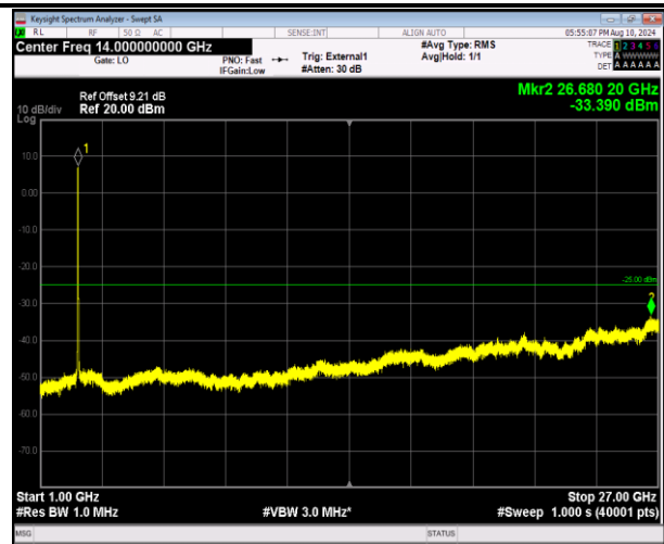
41-41-20MHz-20MHz-16QAM-16QAM-40521-40719-100RB #0-100RB#0-1000~27000MHz-PASS
