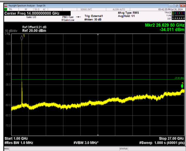
41-41-20MHz-20MHz-64QAM-64QAM-40521-40719-1RB#0 -1RB#99-1000~27000MHz-PASS
