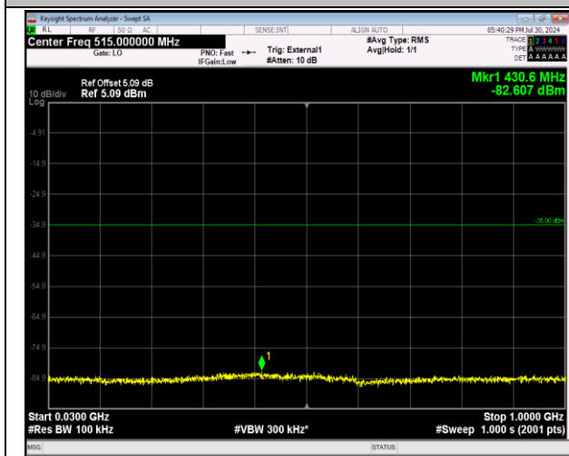
41-41-20MHz-20MHz-64QAM-64QAM-40521-40719-1RB #0-0RB#0-30~1000MHz-PASS
