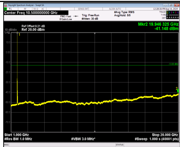
66-66-5MHz-20MHz-64QAM-64QAM-132005-132122-1RB# 24-ORB#0-1000~20000MHz-PASS
