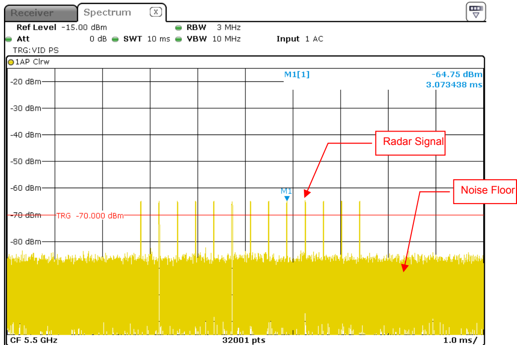
Radar Signal 4
