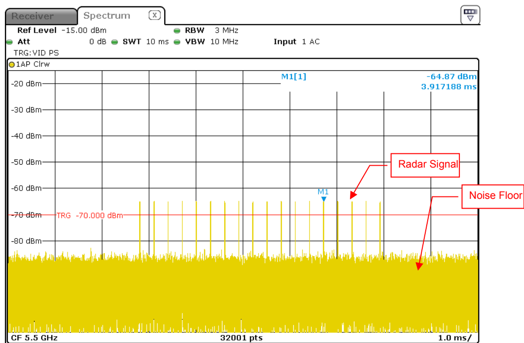
Radar Signal 3
