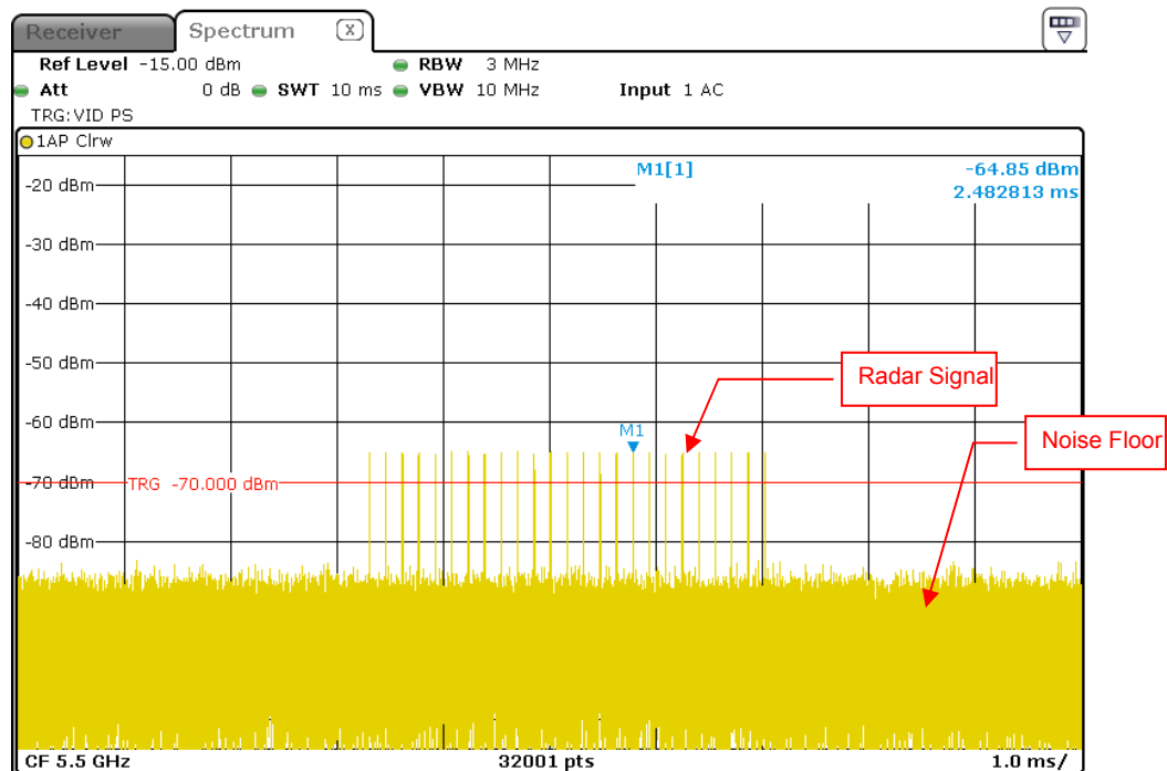
Radar Signal 2
