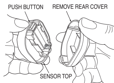
Figure 2. Removing Rear Cover of Mini 4in1 Sensor
