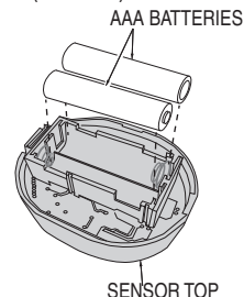
Figure 3. Install Batteries into Sensor Top
