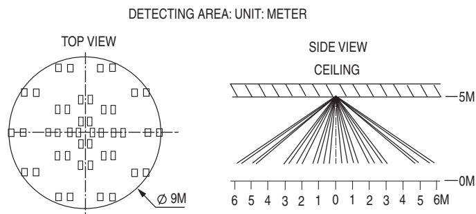
Figure 4. Detecting Area
