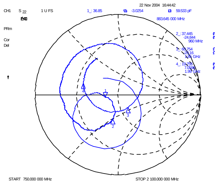
Impedance Smith Chart Antenna Extended Flip Closed
