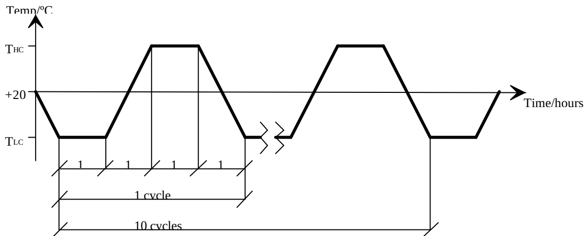
Figure 4-1: Temperature Cycling
