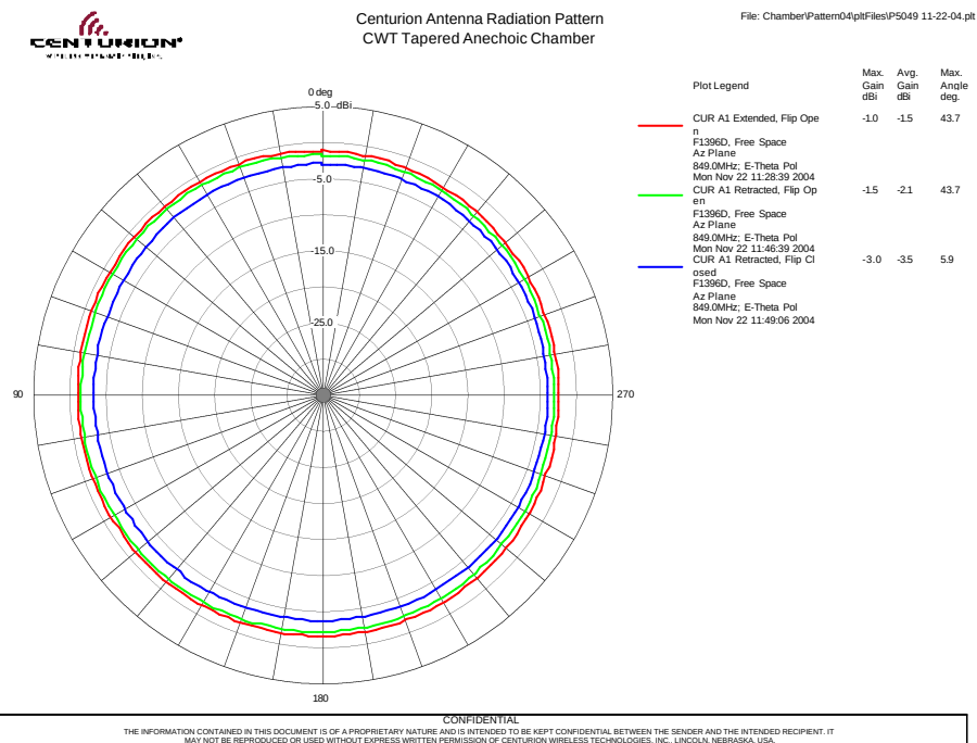
Figure 2-7: OPEN EXTENDED /OPEN & CLOSE RETRACTED CDMA (849 MHz) – Az
