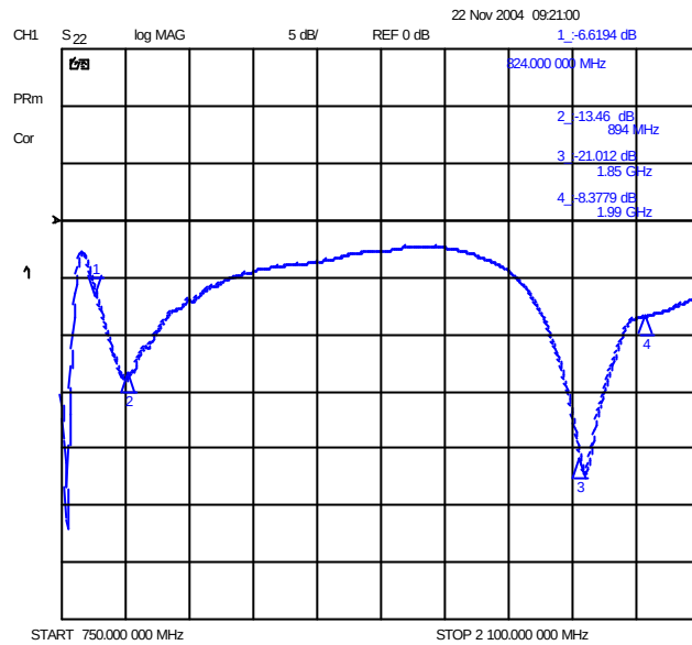
Return Loss Antenna Extended Flip Open
