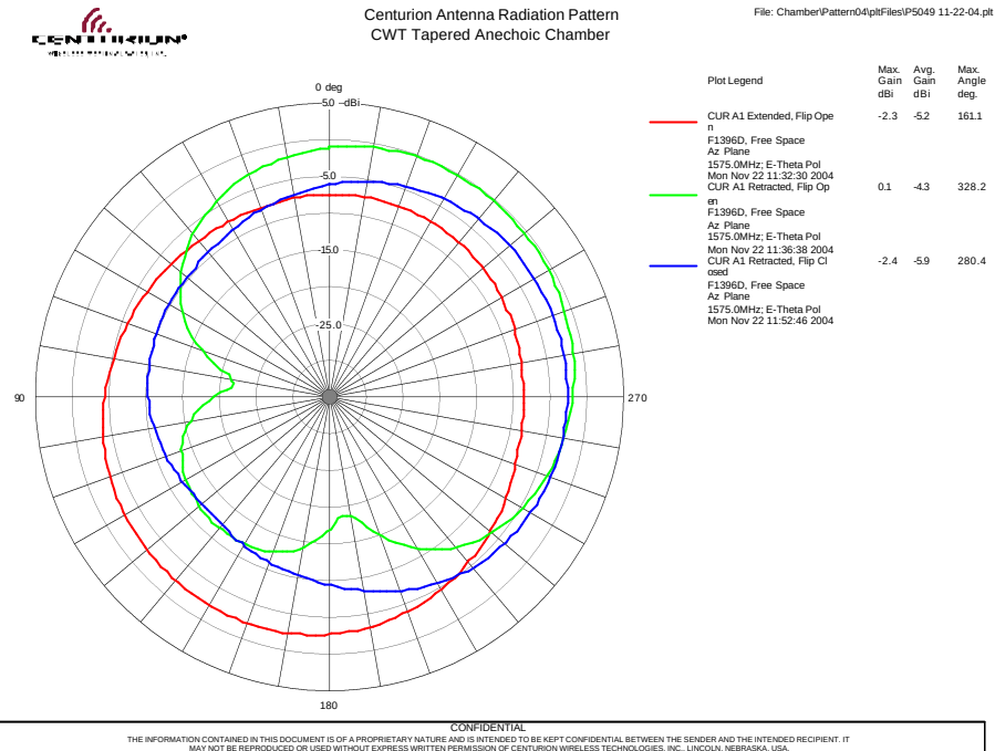
Figure 2-10: OPEN EXTENDED /OPEN & CLOSE RETRACTED GPS (1575 MHz) – Az
