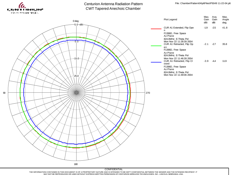
Figure 2-6: OPEN EXTENDED /OPEN & CLOSE RETRACTED CDMA (824 MHz) – Az
