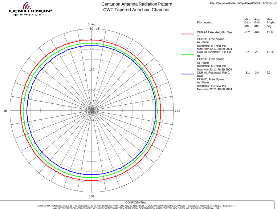
Figure 2-8: OPEN EXTENDED /OPEN & CLOSE RETRACTED CDMA (869 MHz) – Az
