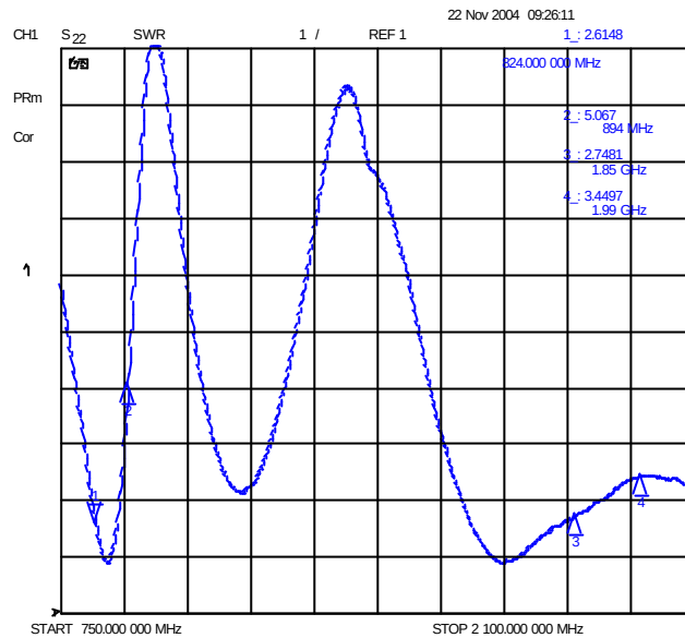
VSWR Antenna Retracted Flip Closed
