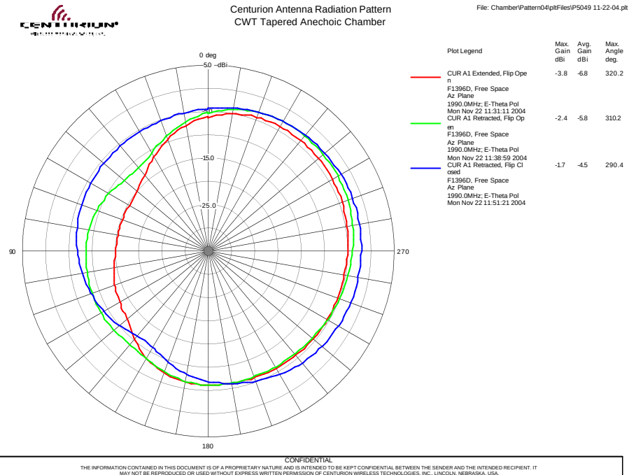
Figure 2-12: OPEN EXTENDED /OPEN & CLOSE RETRACTED PCS (1990 MHz) – Az
