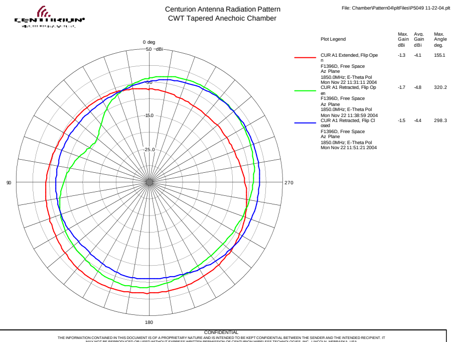
Figure 2-11: OPEN EXTENDED /OPEN & CLOSE RETRACTED PCS (1850 MHz) – Az
