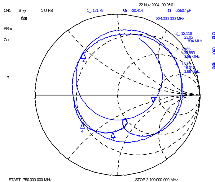
Impedance Smith Chart Antenna Retracted Flip Closed
