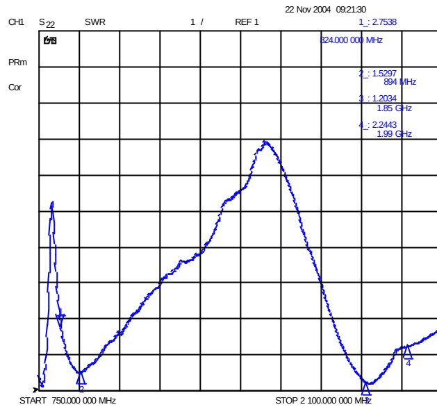
VSWR Antenna Extended Flip Open
