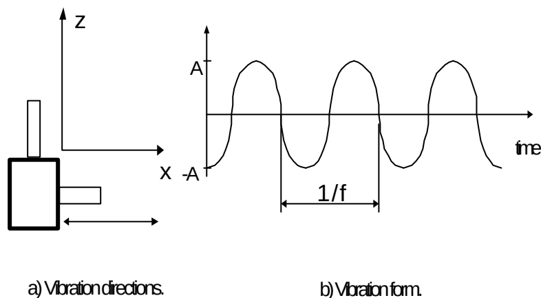
Figure 4-2: Sinusoidal Vibration
