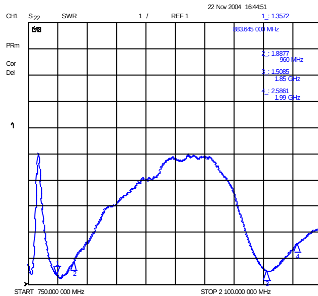
VSWR Antenna Extended Flip Closed
