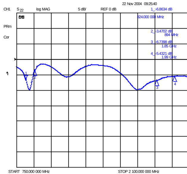
Return Loss Antenna Retracted Flip Closed
