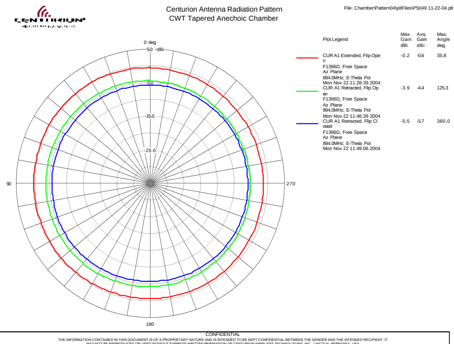
Figure 2-9: OPEN EXTENDED /OPEN & CLOSE RETRACTED CDMA (894 MHz) – Az
