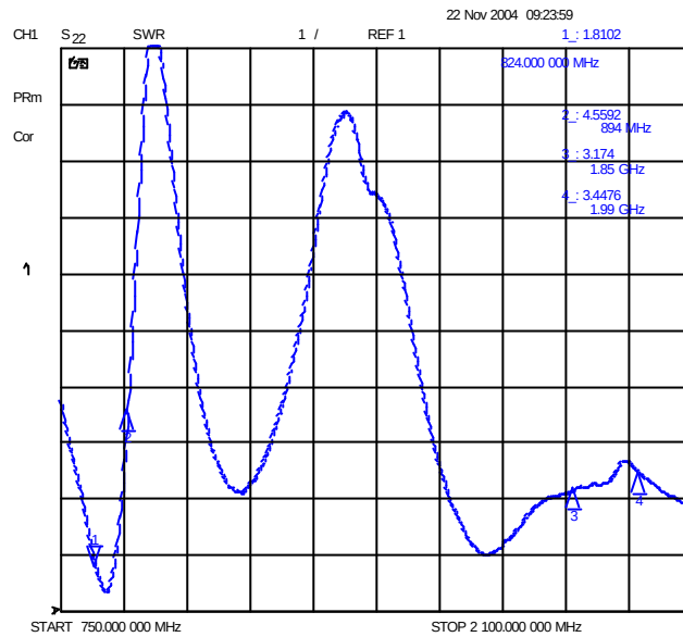
VSWR Antenna Retracted Flip Open
