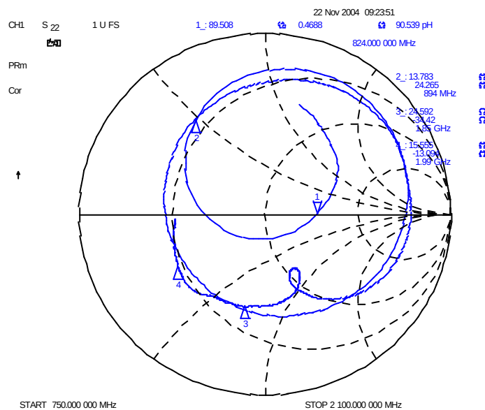
Impedance Smith Chart Antenna Retracted Flip Open
