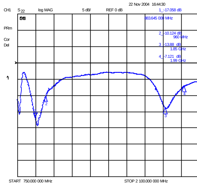
Return Loss Antenna Extended Flip Closed
