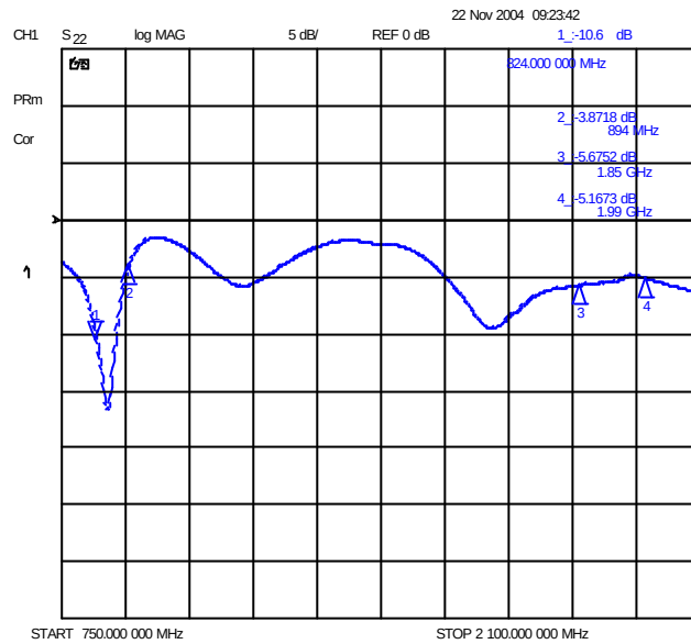
Return Loss Antenna Retracted Flip Open
