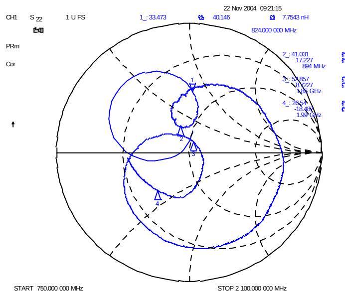
Impedance Smith Chart Antenna Extended Flip Open
