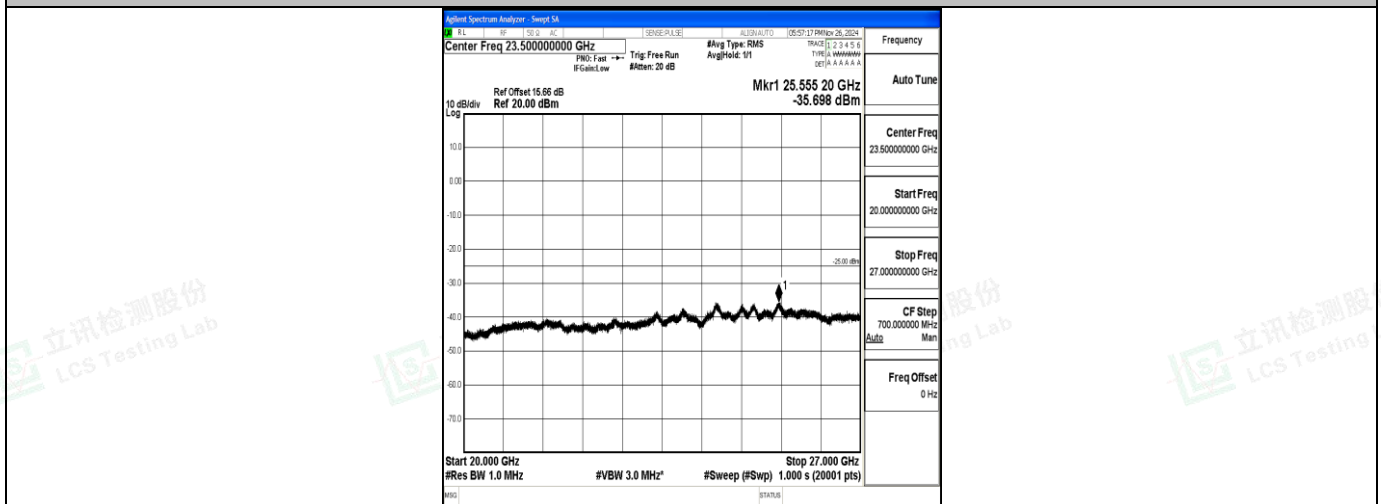
Band7_10MHz_QPSK_21400_1RB#0_20000~27000_20000~27000
