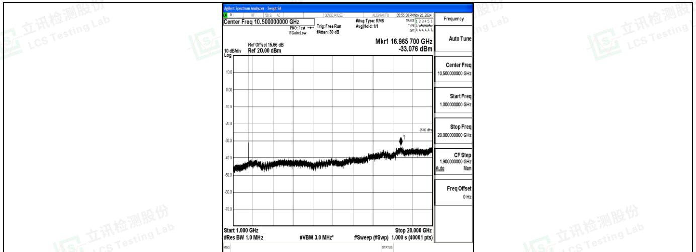
Band7_10MHz_16QAM_20800_1RB#0_1000~20000_1000~20000
