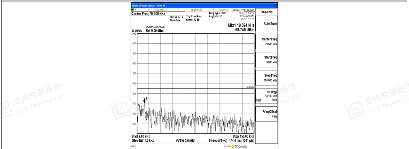
Band7_10MHz_16QAM_21100_1RB#0_0.009~0.15_0.009~0.15
