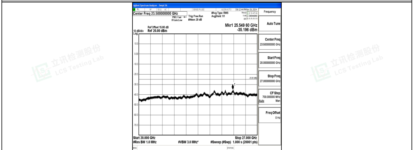
Band7_15MHz_QPSK_20825_1RB#0_20000~27000_20000~27000
