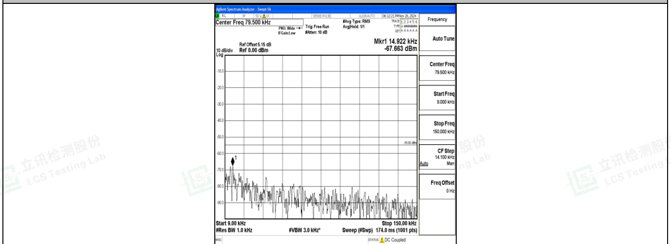
Band7_15MHz_QPSK_20825_1RB#0_0.009~0.15_0.009~0.15
