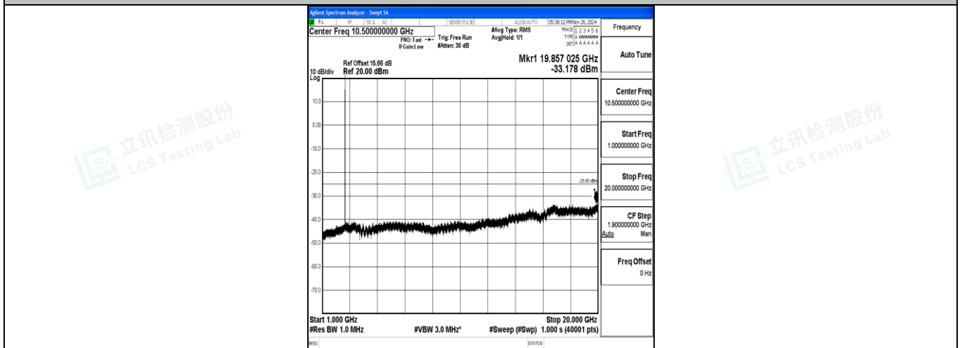
Band7_5MHz_16QAM_21425_1RB#0_1000~20000_1000~20000
