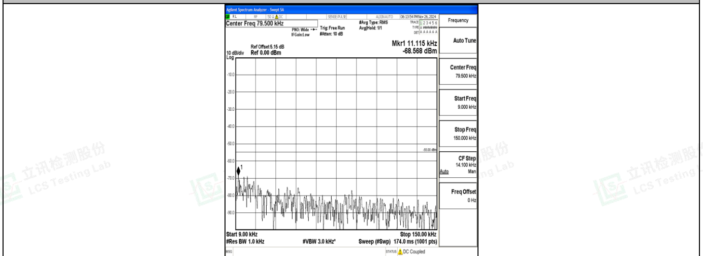
Band7_15MHz_16QAM_21100_1RB#0_0.009~0.15_0.009~0.15
