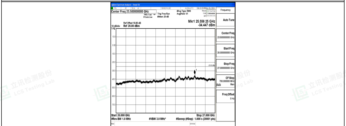
Band7_15MHz_16QAM_20825_1RB#0_20000~27000_20000~27000
