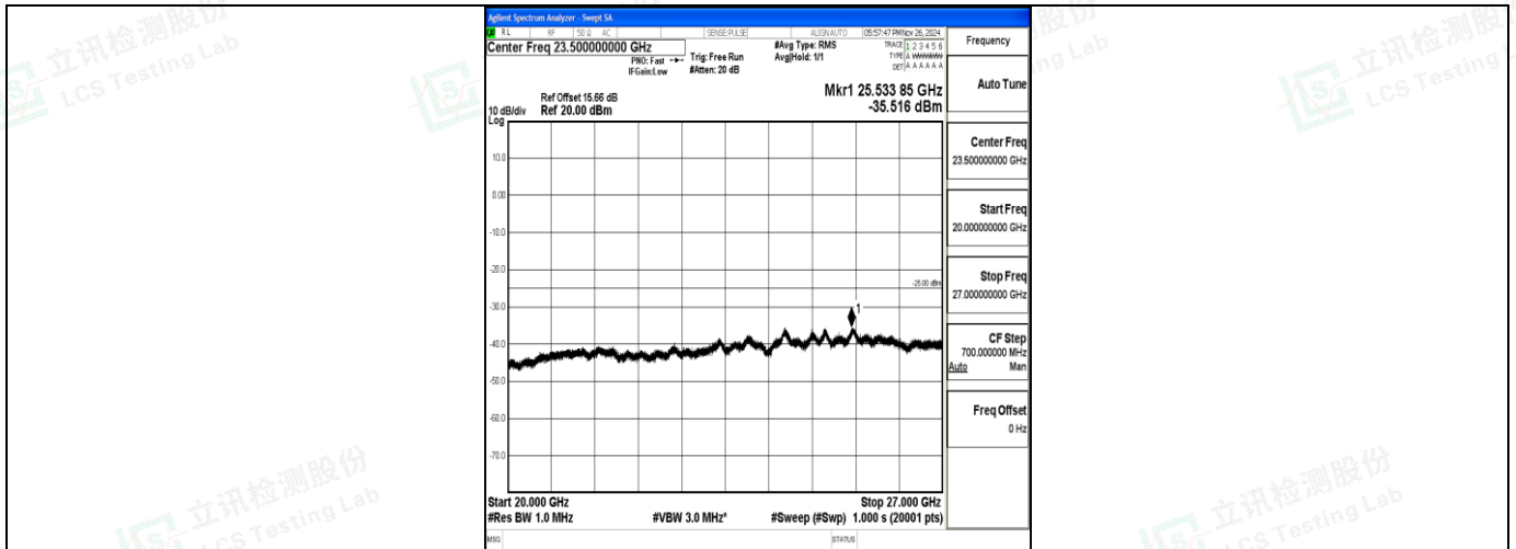
Band7_10MHz_16QAM_21400_1RB#0_20000~27000_20000~27000
