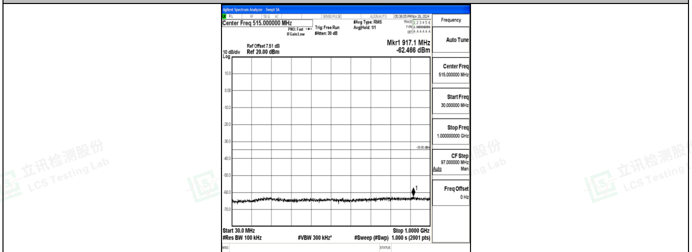
Band7_5MHz_16QAM_21425_1RB#0_30~1000_30~1000
