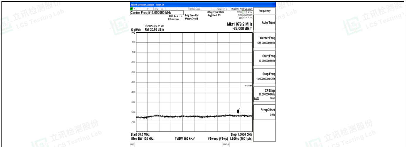
Band7_10MHz_QPSK_20800_1RB#0_30~1000_30~1000
