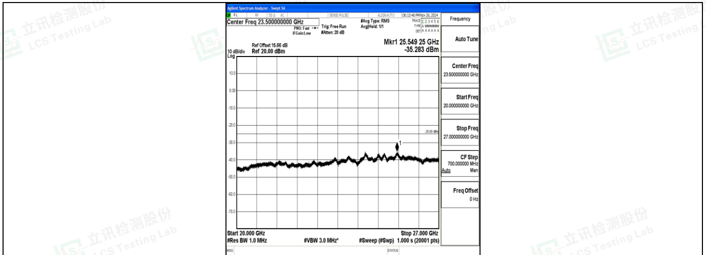
Band7_15MHz_QPSK_21100_1RB#0_20000~27000_20000~27000
