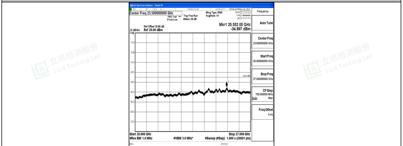
Band7_10MHz_16QAM_21100_1RB#0_20000~27000_20000~27000
