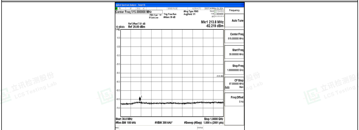
Band7_10MHz_16QAM_21400_1RB#0_30~1000_30~1000
