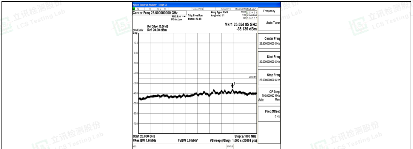
Band7_5MHz_16QAM_21425_1RB#0_20000~27000_20000~27000
