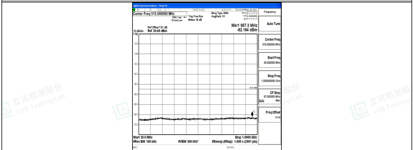
Band7_15MHz_QPSK_21100_1RB#0_30~1000_30~1000
