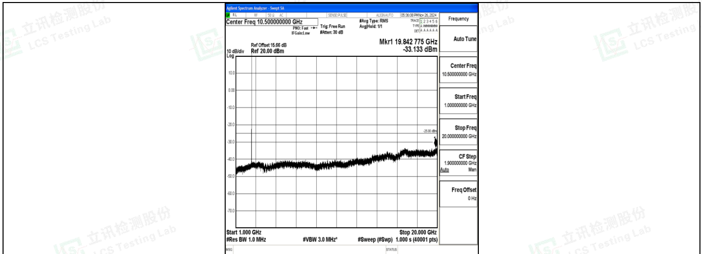
Band7_5MHz_16QAM_20775_1RB#0_1000~20000_1000~20000
