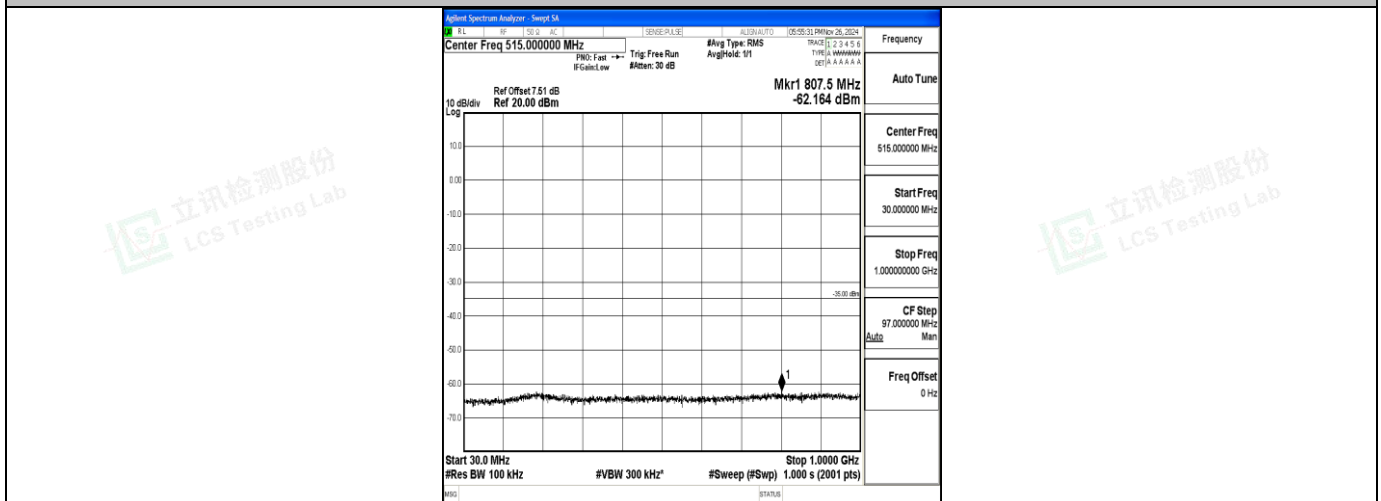
Band7_10MHz_16QAM_20800_1RB#0_30~1000_30~1000
