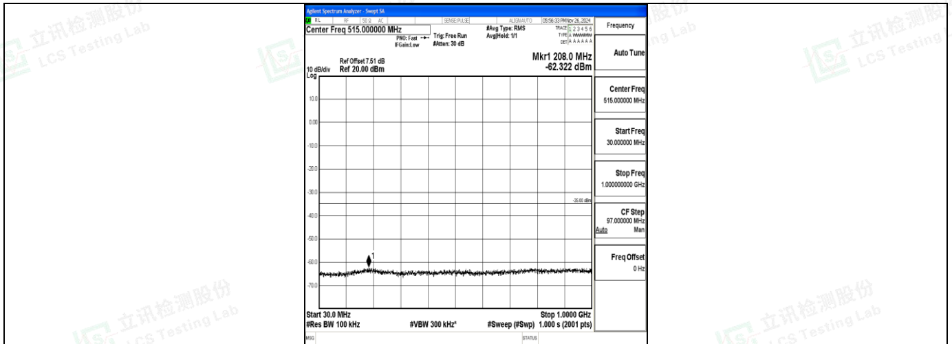
Band7_10MHz_16QAM_21100_1RB#0_30~1000_30~1000
