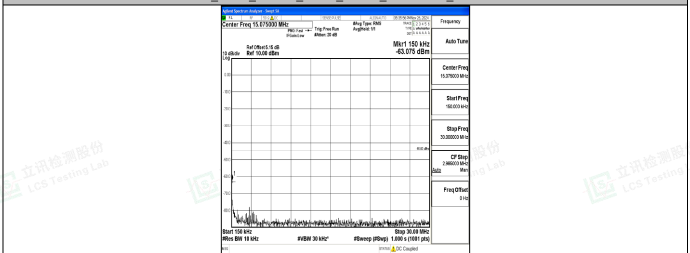
Band7_5MHz_16QAM_20775_1RB#0_0.15~30_0.15~30
