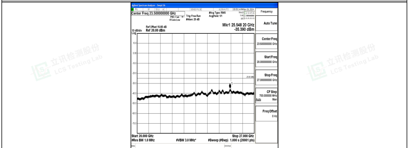
Band7_10MHz_QPSK_20800_1RB#0_20000~27000_20000~27000
