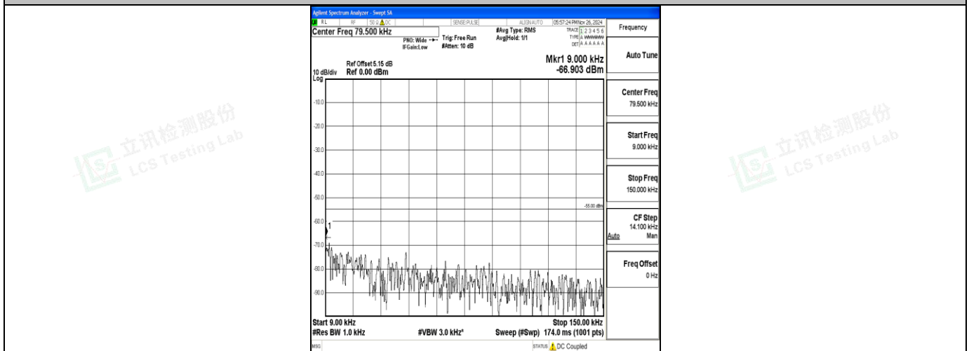
Band7_10MHz_16QAM_21400_1RB#0_0.009~0.15_0.009~0.15
