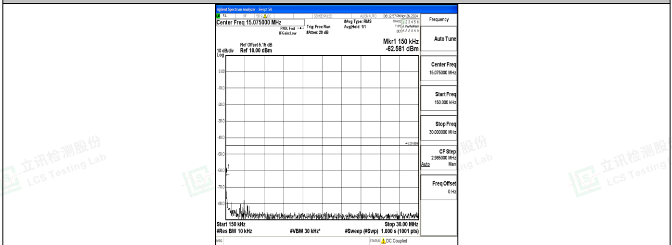
Band7_15MHz_16QAM_20825_1RB#0_0.15~30_0.15~30
