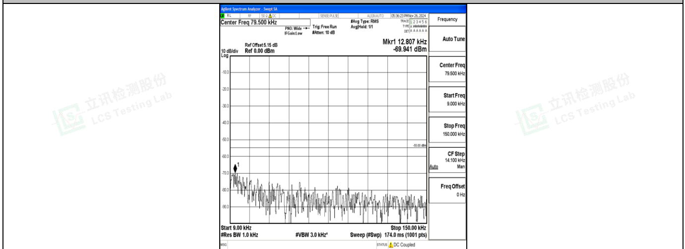
Band7_5MHz_QPSK_21100_1RB#0_0.009~0.15_0.009~0.15
