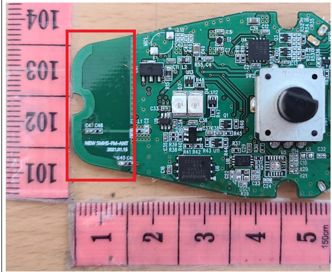
BT Antenna
