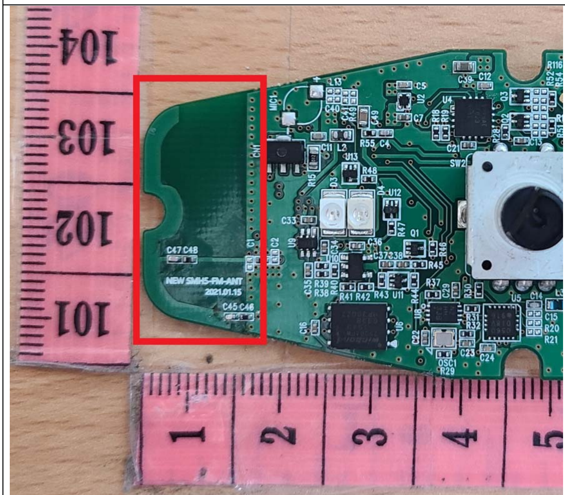
BT Antenna
