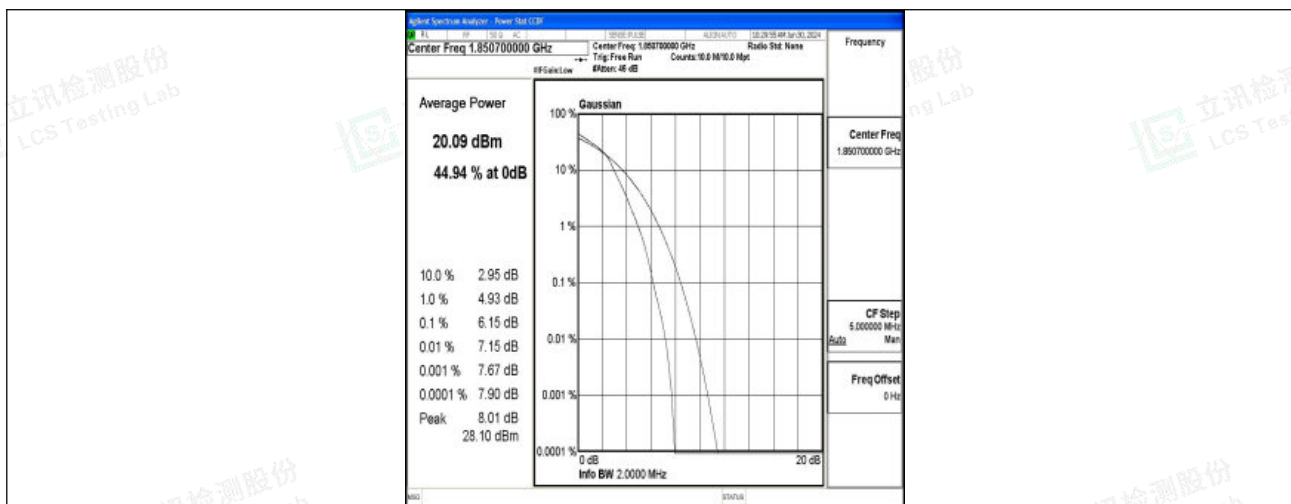
Band2-1.4MHz-16QAM-18607-6RB#0-PASS
