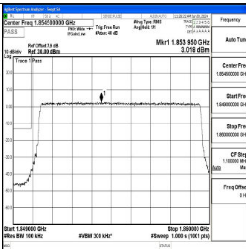
Band2_10MHz_QPSK_18650_50RB#0
