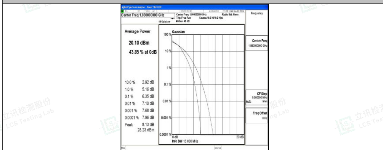
Band2-15MHz-16QAM-18900-75RB#0-PASS
