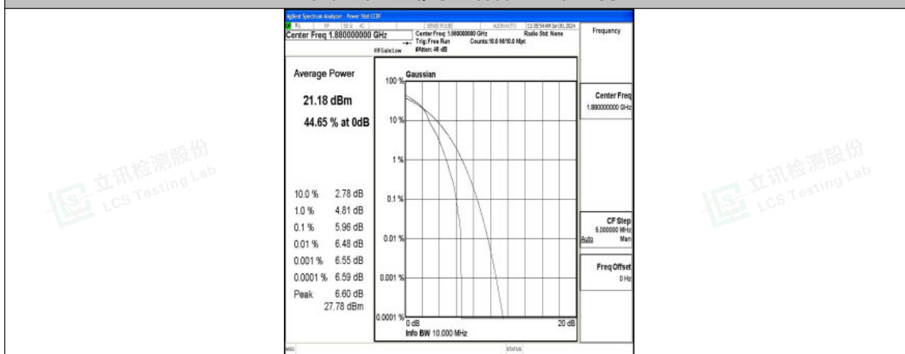
Band2-10MHz-16QAM-18900-1RB#0-PASS
