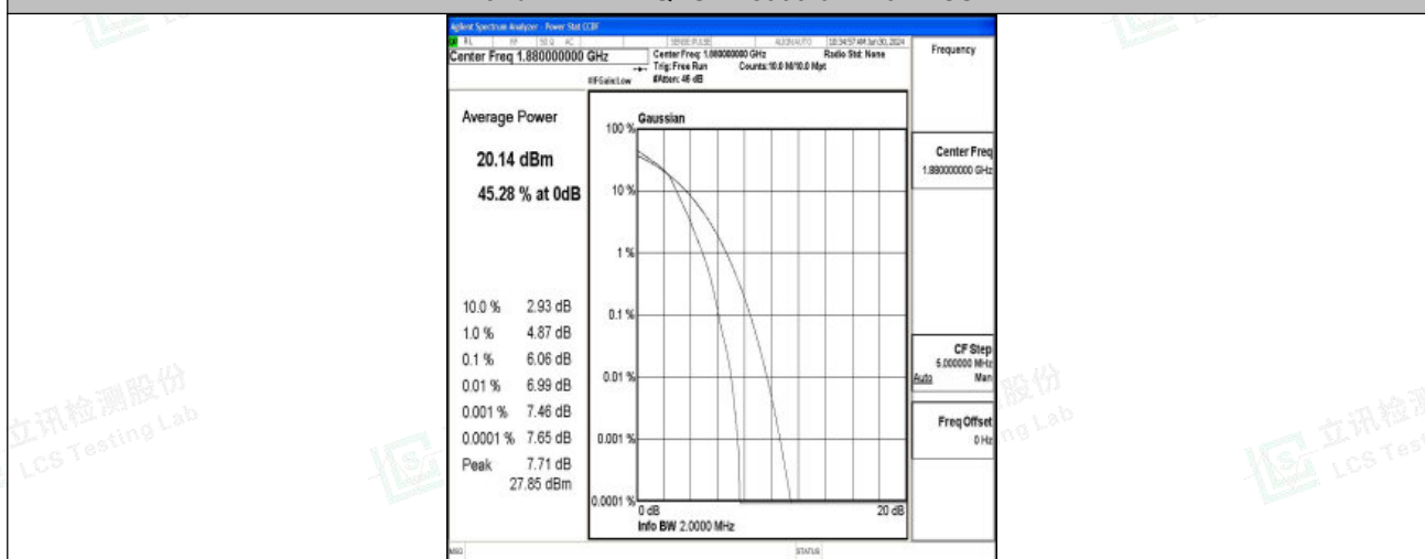
Band2-1.4MHz-16QAM-18900-6RB#0-PASS
