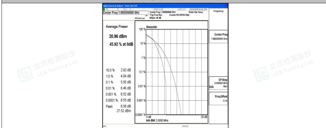
Band2-1.4MHz-16QAM-18900-1RB#0-PASS
