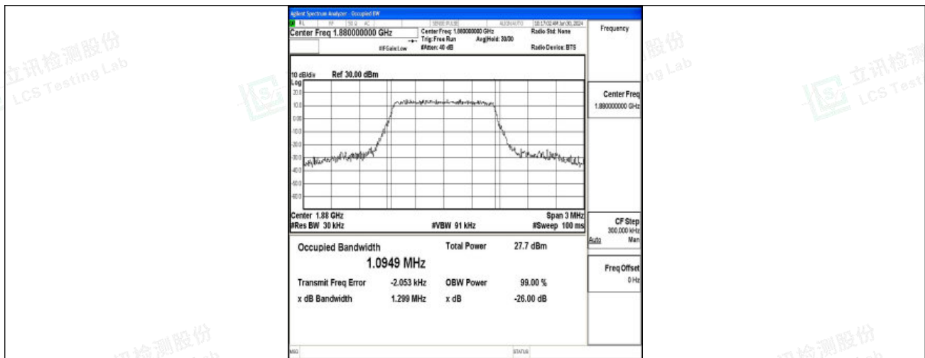
Band2-1.4MHz-16QAM-18900-6RB#0-PASS
