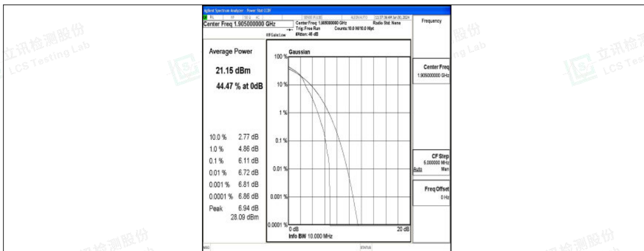
Band2-10MHz-16QAM-19150-1RB#0-PASS
