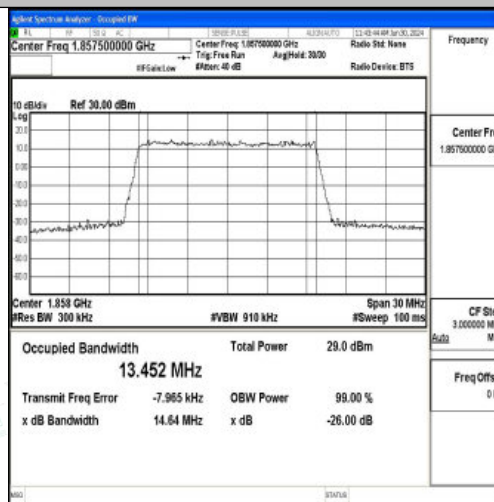
Band2-15MHz-16QAM-18675-75RB#0-PASS
