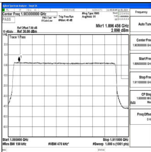
Band2_15MHz_QPSK_19125_75RB#0
