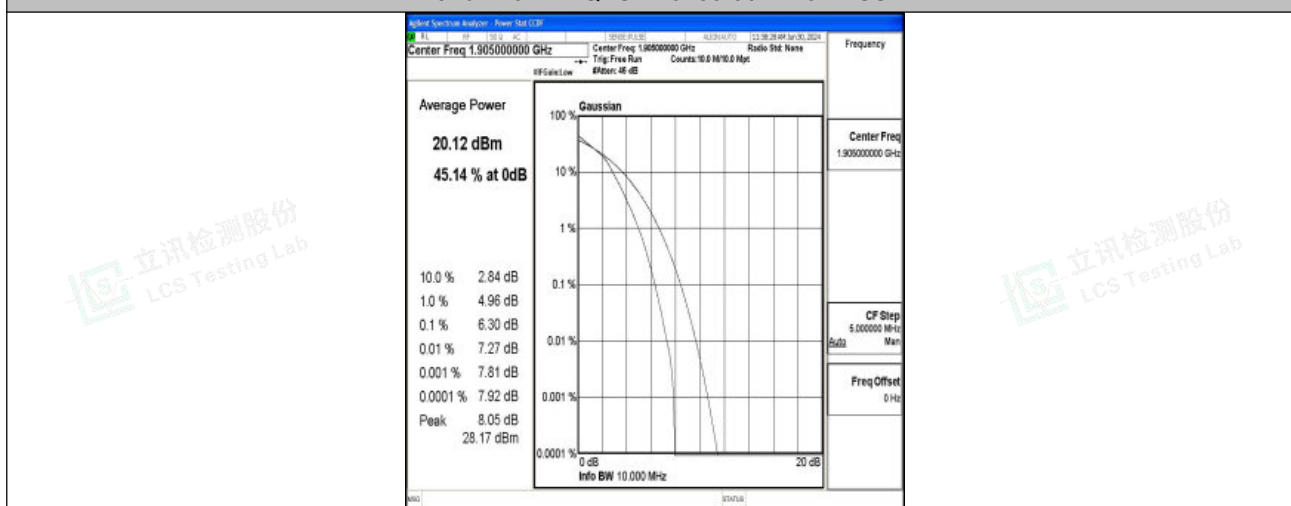
Band2-10MHz-16QAM-19150-50RB#0-PASS
