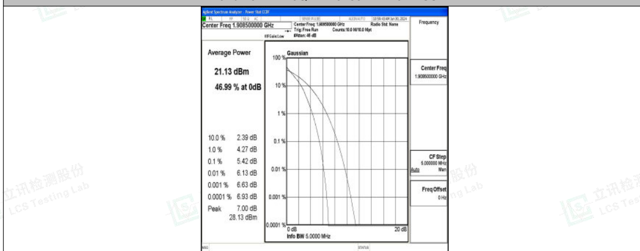
Band2-3MHz-QPSK-19185-15RB#0-PASS
