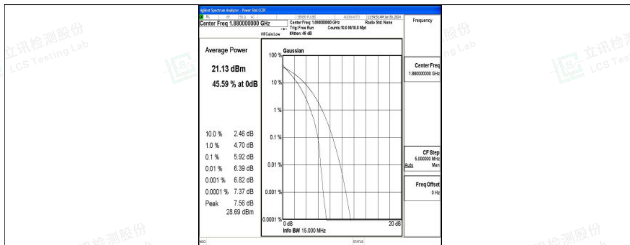
Band2-15MHz-QPSK-18900-75RB#0-PASS
