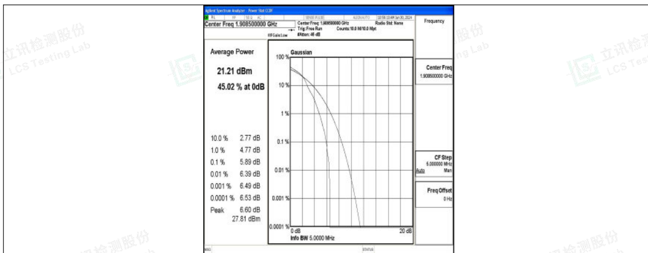
Band2-3MHz-16QAM-19185-1RB#0-PASS
