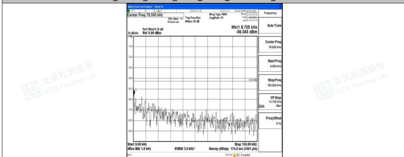
Band2_1.4MHz_QPSK_18900_1RB#0_0.009~0.15_0.009~0.15
