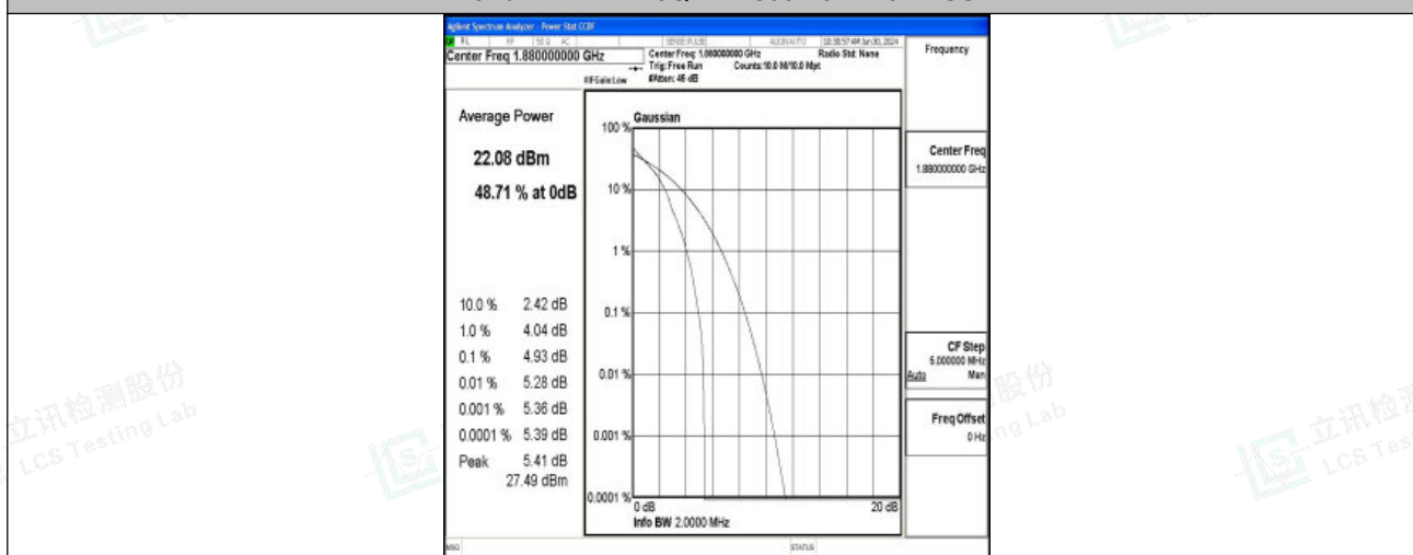
Band2-1.4MHz-QPSK-18900-1RB#0-PASS
