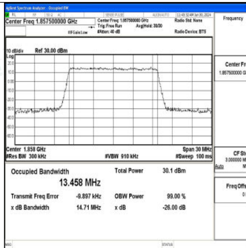
Band2-15MHz-QPSK-18675-75RB#0-PASS
