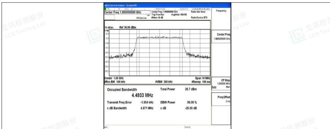
Band2-5MHz-16QAM-18900-25RB#0-PASS
