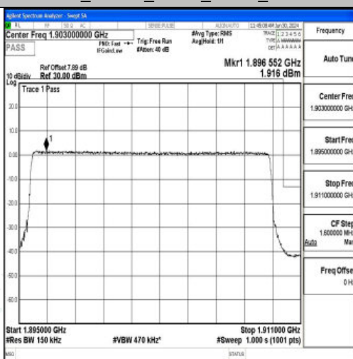
Band2_15MHz_16QAM_19125_75RB#0
