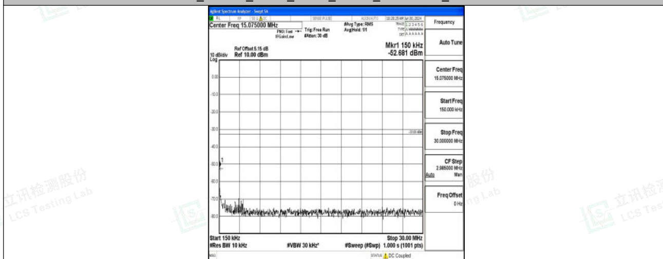
Band2_1.4MHz_QPSK_19193_1RB#0_0.15~30_0.15~30
