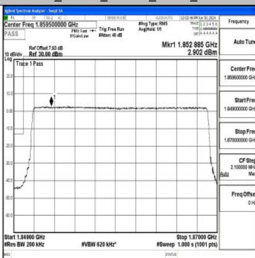
Band2_20MHz_QPSK_18700_100RB#0
