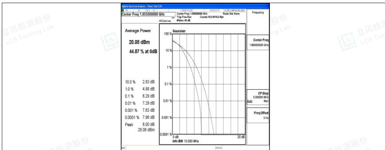
Band2-10MHz-16QAM-18650-50RB#0-PASS
