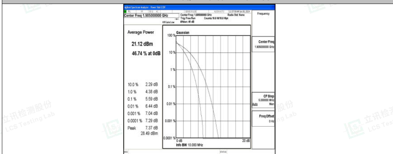
Band2-10MHz-QPSK-19150-50RB#0-PASS
