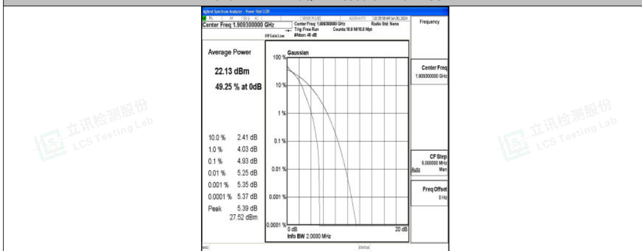
Band2-1.4MHz-QPSK-19193-1RB#0-PASS
