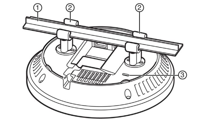
Figure 4 WS-AP3805 Mounted on Drop Ceiling T-bar Rail
