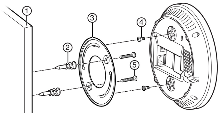
Figure 5 Mounting the WS-AP3805 to a Flat Wall or Solid Ceiling
