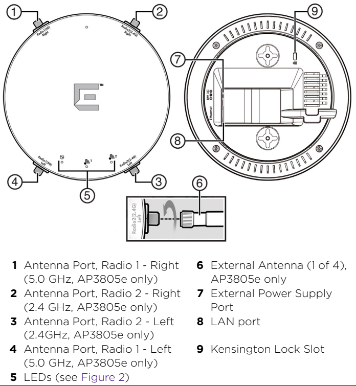
Figure 1 Front & Back Views of the WS-AP3805
