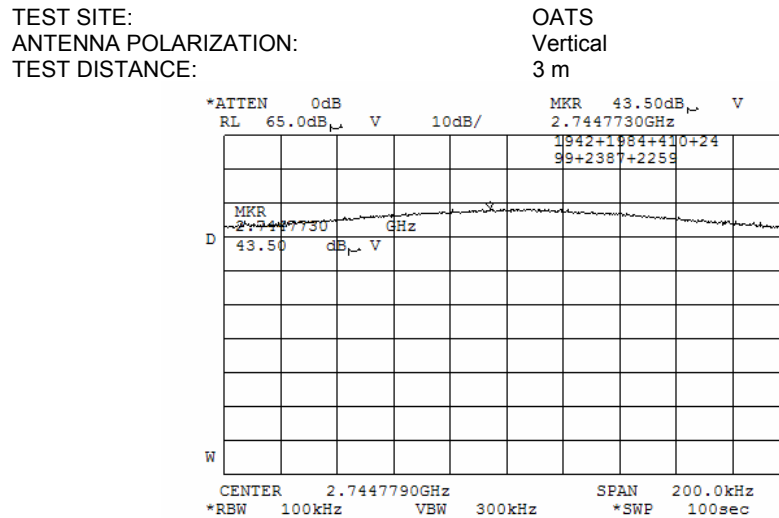
Plot 4.3.14 Radiated emission measurements at the 3 rd harmonic
