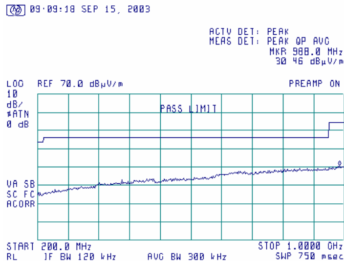
Plot 4.4.2 Radiated emission measurements in the anechoic chamber from 200 MHz to 1 GHz, vertical & horizontal antenna polarization
