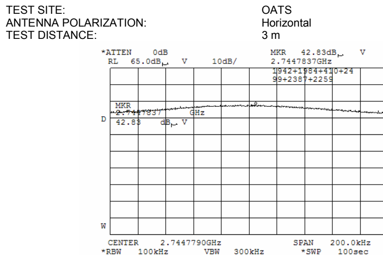
Plot 4.3.15 Radiated emission measurements at the 3 rd harmonic
