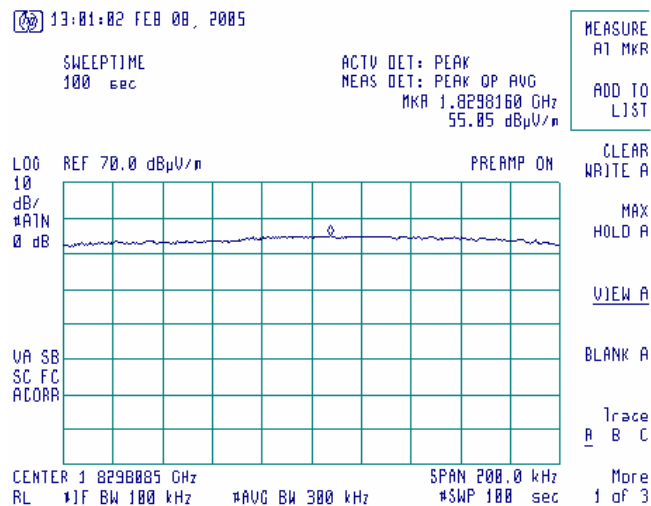
Plot 4.3.13 Radiated emission measurements at the 2 nd harmonic
