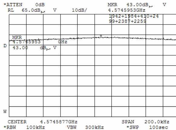
Plot 4.3.19 Radiated emission measurements at the 5 th harmonic
