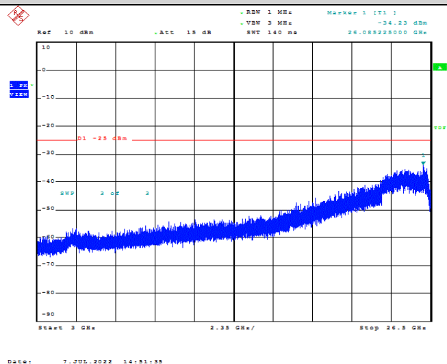
Band7-15MHz-16QAM-21375-1RB#0-Range1:3000~26500MHz
