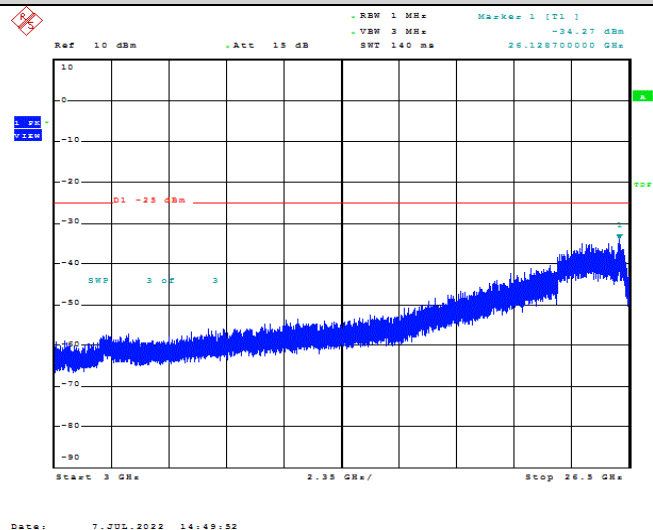
Band7-10MHz-16QAM-21400-1RB#0-Range1:3000~26500MHz
