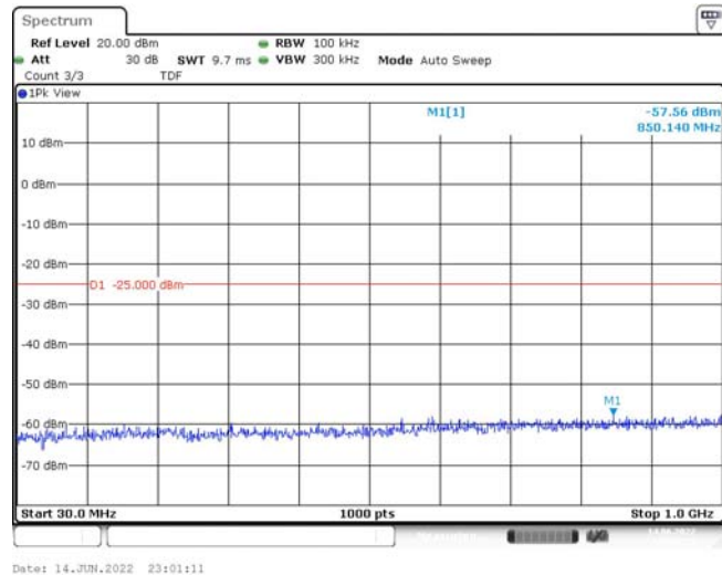
Band7-15MHz-16QAM-21375-1RB#0-Range1:30~1000MHz
