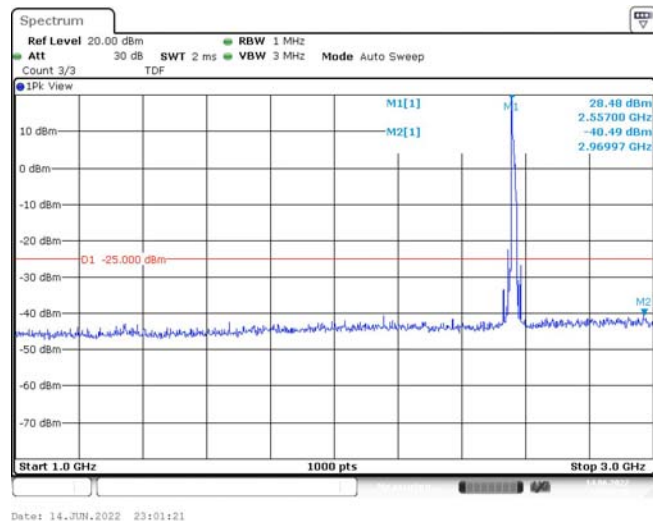
Band7-15MHz-16QAM-21375-1RB#0-Range2:1000~3000MHz
