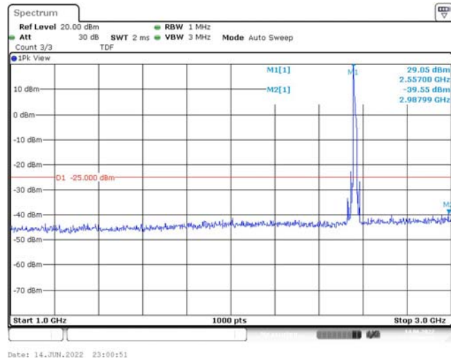
Band7-15MHz-QPSK-21375-1RB#0-Range2:1000~3000MHz
