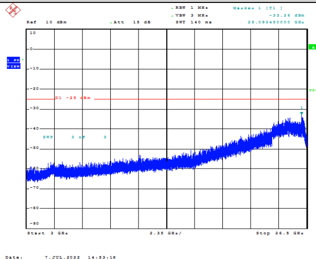
Band7-20MHz-16QAM-21350-1RB#0-Range1:3000~26500MHz
