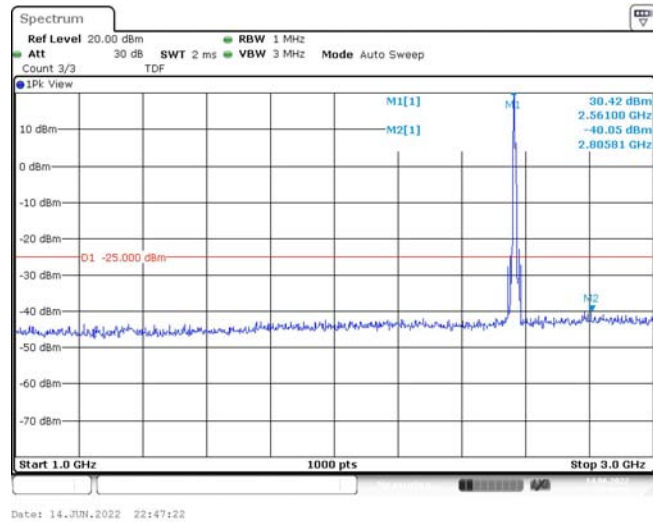
Band7-10MHz-16QAM-21400-1RB#0-Range2:1000~3000MHz
