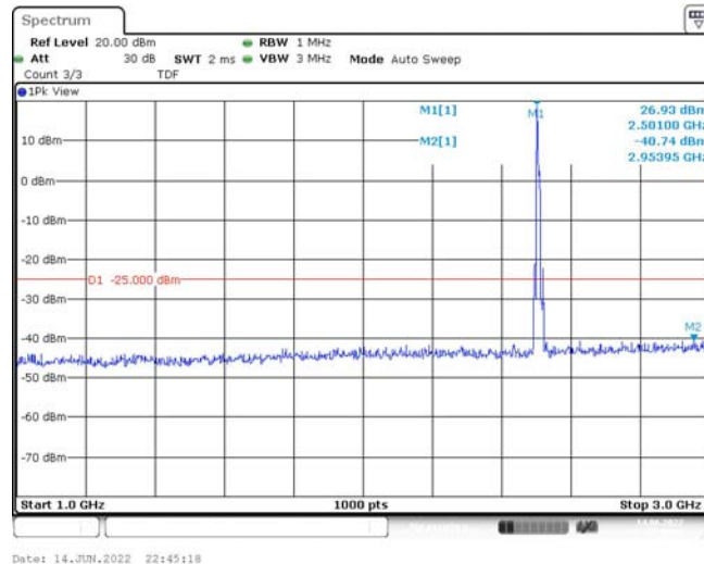
Band7-10MHz-16QAM-20800-1RB#0-Range2:1000~3000MHz
