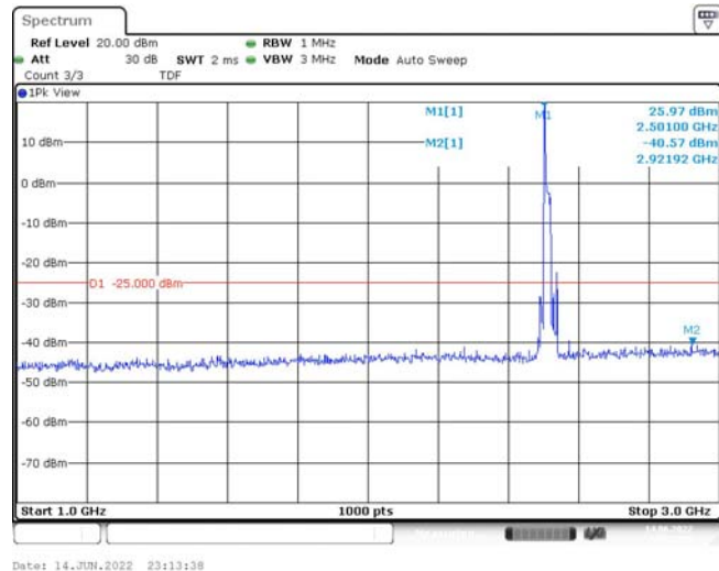
Band7-20MHz-16QAM-20850-1RB#0-Range2:1000~3000MHz
