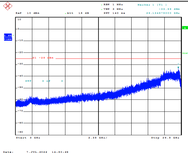
Band7-15MHz-16QAM-20825-1RB#0-Range1:3000~26500MHz
