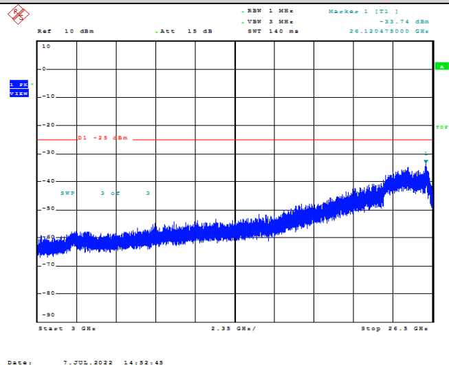
Band7-20MHz-16QAM-21100-1RB#0-Range1:3000~26500MHz
