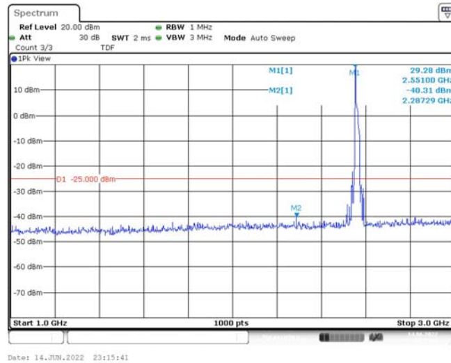
Band7-20MHz-16QAM-21350-1RB#0-Range2:1000~3000MHz
