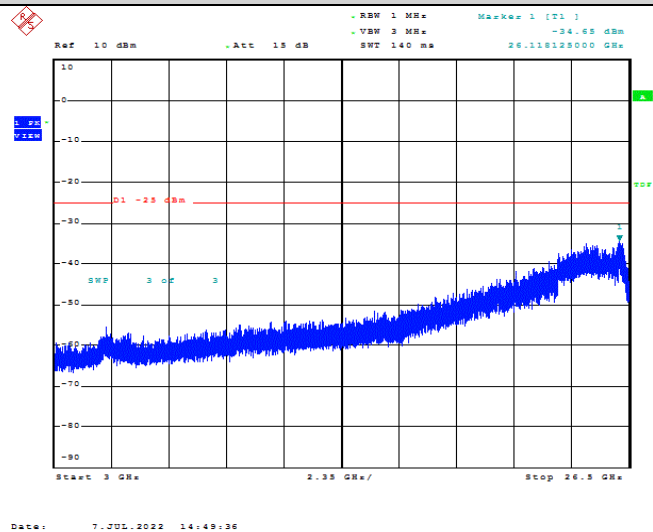
Band7-10MHz-QPSK-21400-1RB#0-Range1:3000~26500MHz
