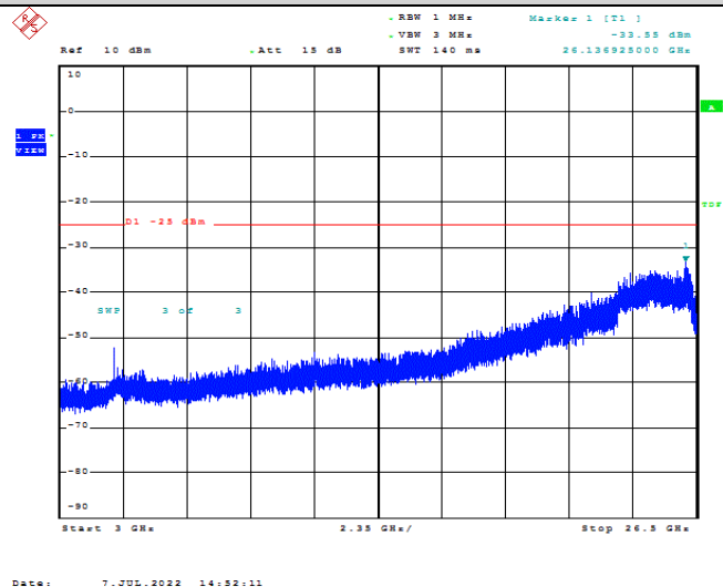
Band7-20MHz-16QAM-20850-1RB#0-Range1:3000~26500MHz
