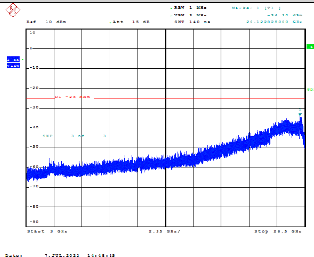
Band7-10MHz-16QAM-20800-1RB#0-Range1:3000~26500MHz
