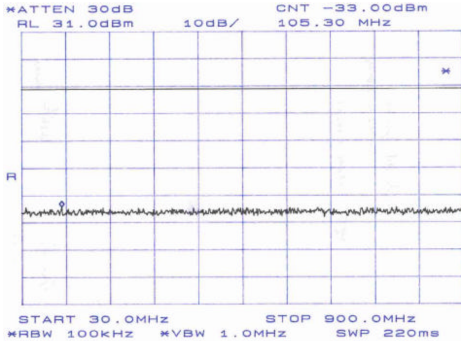
Figure 4-8. Conducted Spurious Emissions, Low Channel 30 - 900MHz
