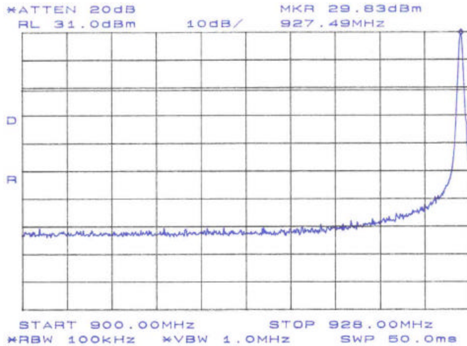
Figure 4-25. Conducted Spurious Emissions, High Channel 900 - 928MHz
