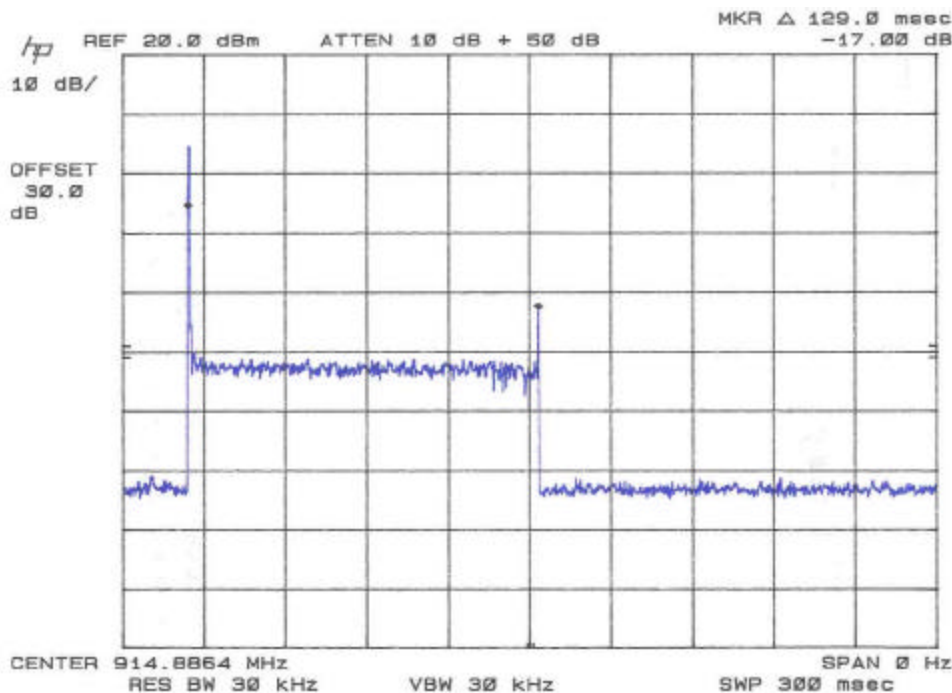
Figure 4-7. Dwell Time
