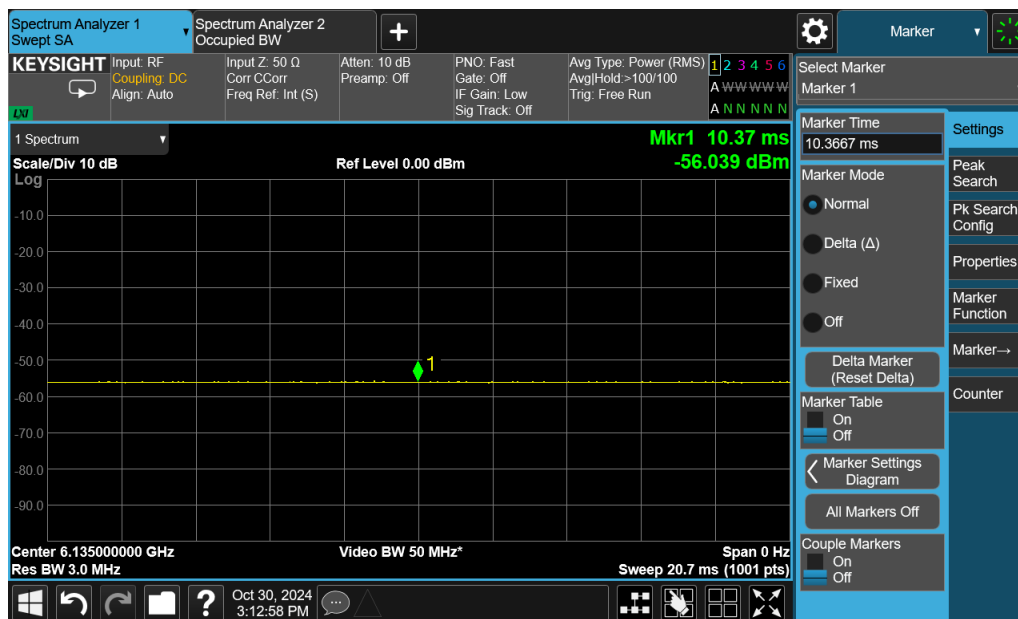
Plot 2: AWGN Signal Level Details
