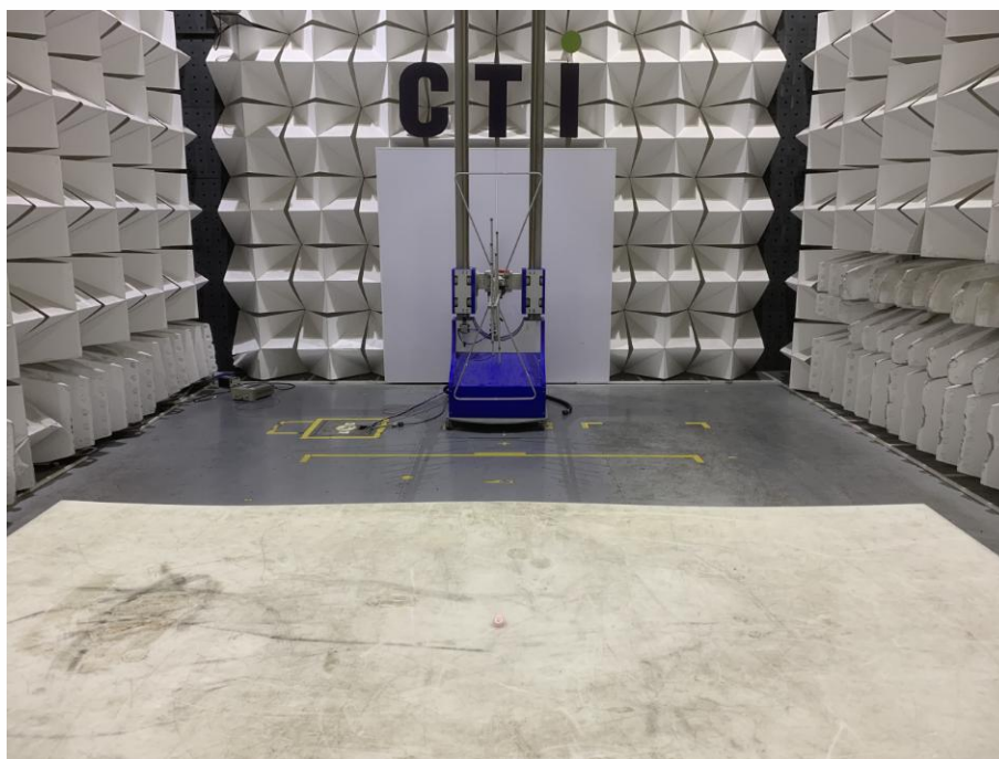
Radiated spurious emission Test Setup-1(Below 1GHz) Ear R
