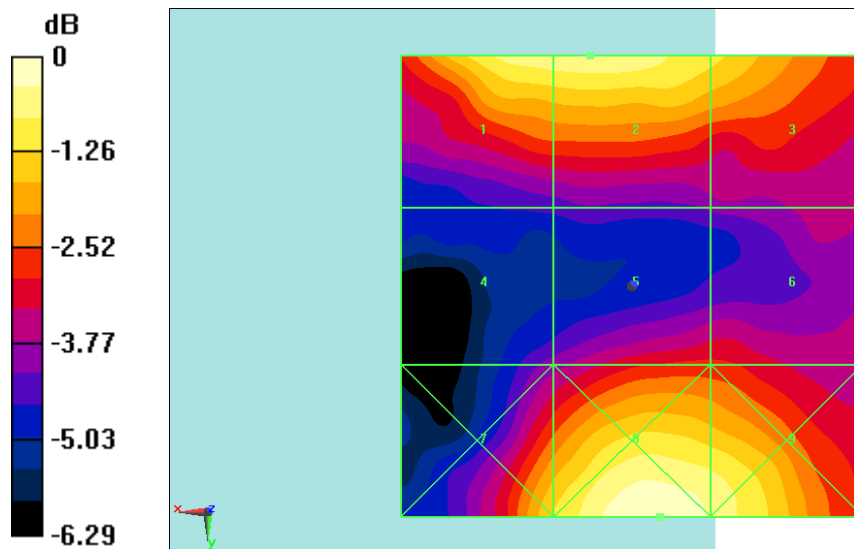
Fig B.3 HAC RF E-Field LTE Band41 QPSK CH39750
