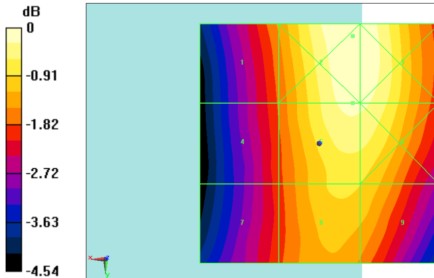
Fig B.1 HAC RF E-Field GSM 850 Middle
