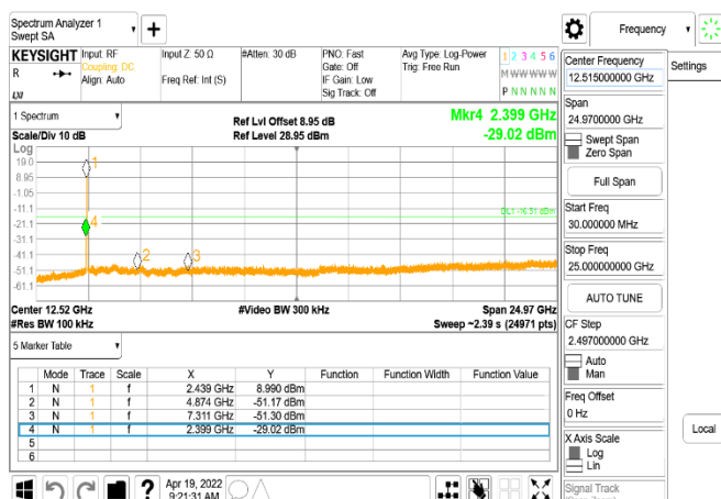
802.11ax_40MHz_Chain0_2437MHz
