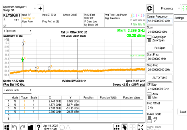
802.11ax_40MHz_Chain1_2437MHz
