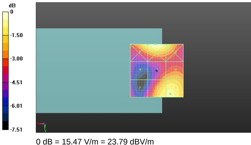
Fig A.7 HAC RF E-Field LTE Band 41
