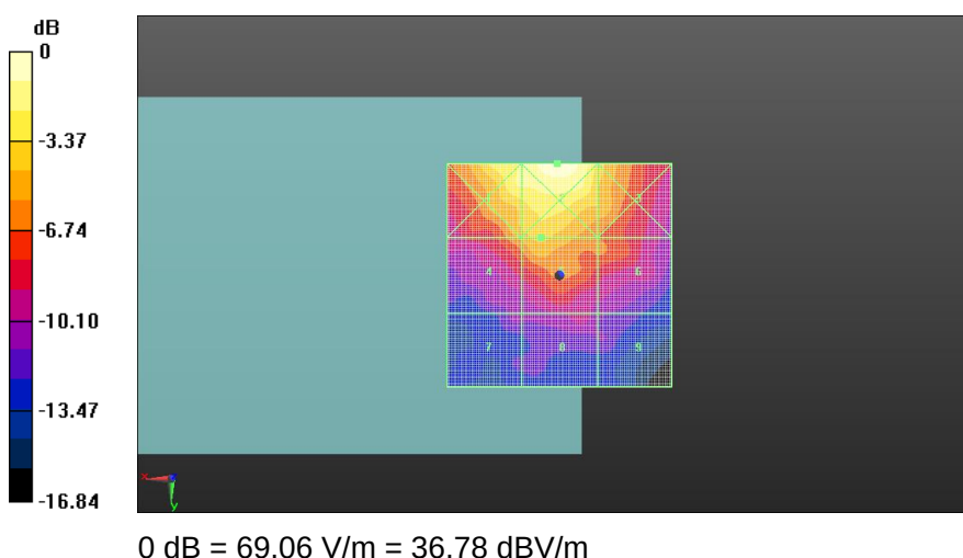
Fig A.1 HAC RF E-Field CDMA BC0
