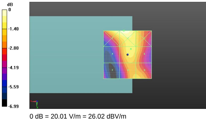
Fig A.9 HAC RF E-Field LTE Band 41
