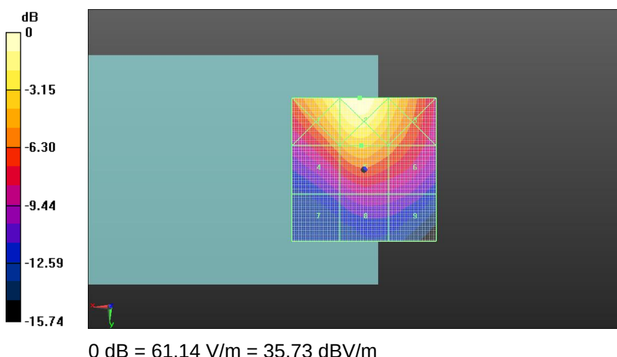
Fig A.2 HAC RF E-Field CDMA BC0
