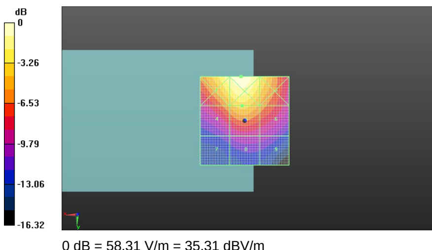
Fig A.3 HAC RF E-Field CDMA BC0
