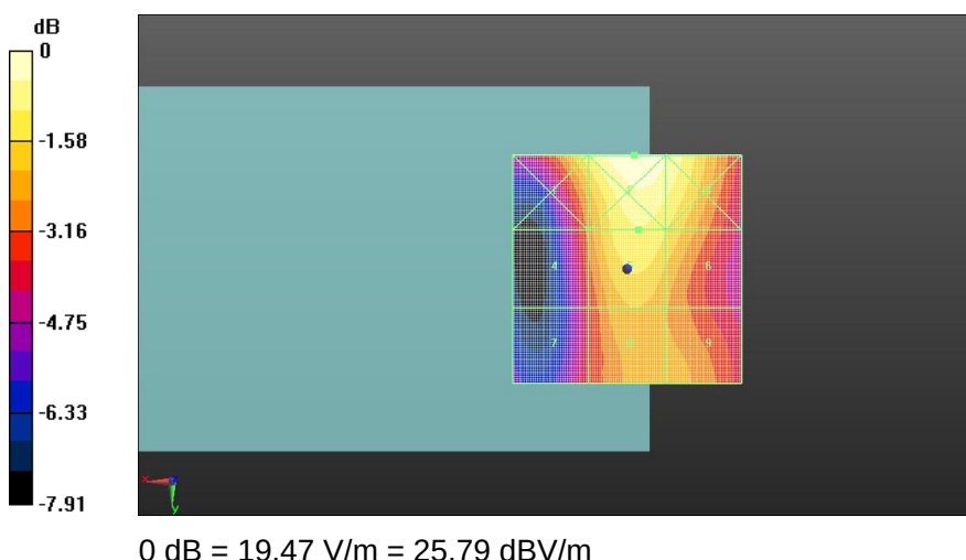
Fig A.8 HAC RF E-Field LTE Band 41
