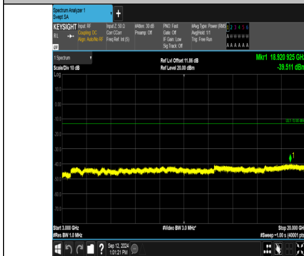
Band2_5MHz_QPSK_18900_1RB#24_3000~20000_3000~20000
