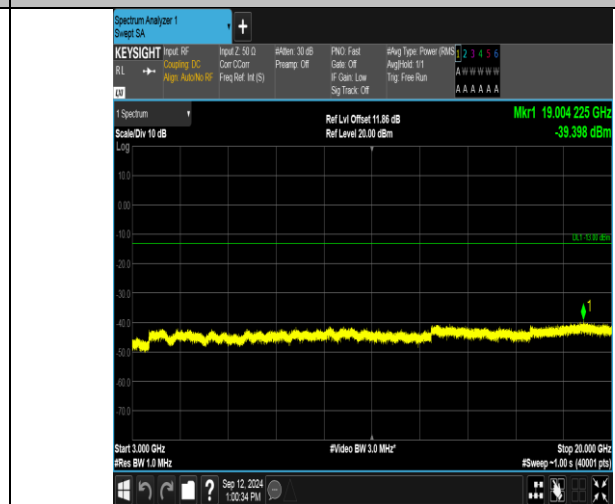
Band2_5MHz_16QAM_18900_1RB#0_3000~20000_3000~20000
