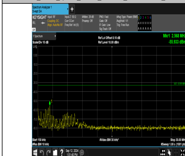
Band2_5MHz_16QAM_18900_1RB#24_0.15~30_0.15~30
