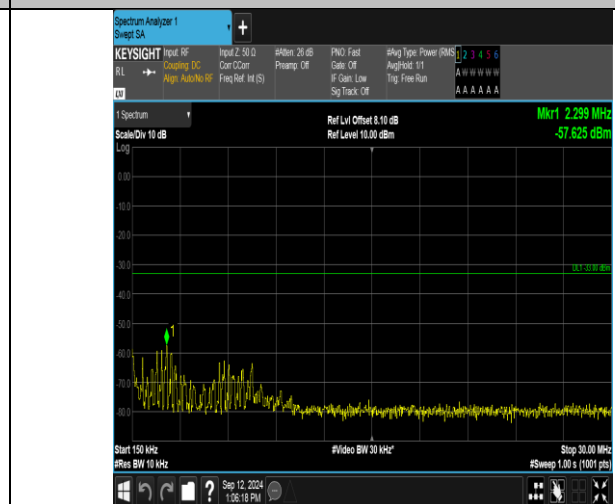
Band2_5MHz_QPSK_19175_1RB#24_0.15~30_0.15~30
