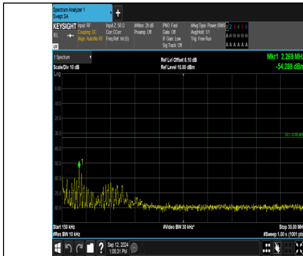
Band2_5MHz_16QAM_19175_1RB#0_0.15~30_0.15~30
