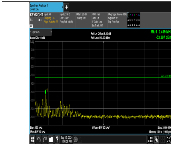
Band2_5MHz_16QAM_18900_1RB#0_0.15~30_0.15~30
