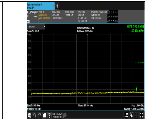
Band2_5MHz_16QAM_19175_1RB#0_30~1000_30~1000
