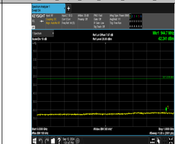
Band2_5MHz_16QAM_18900_1RB#24_30~1000_30~1000
