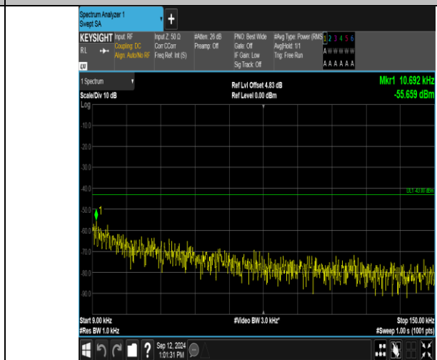
Band2_5MHz_16QAM_18900_1RB#24_0.009~0.15_0.009~0.15
