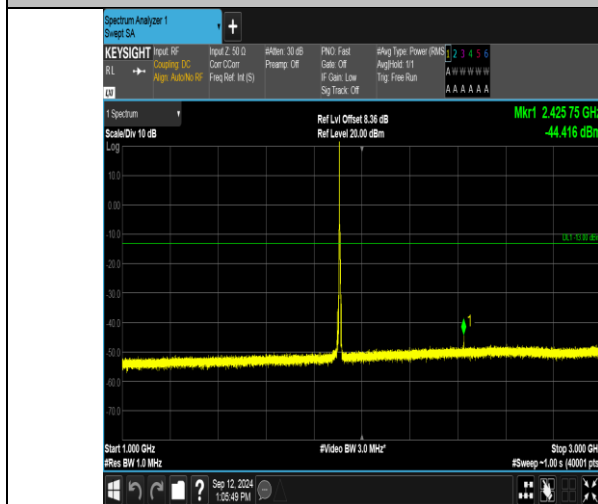
Band2_5MHz_16QAM_19175_1RB#0_1000~3000_1000~3000
