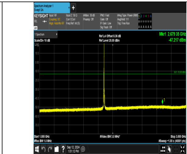
Band2_5MHz_QPSK_18900_1RB#24_1000~3000_1000~3000
