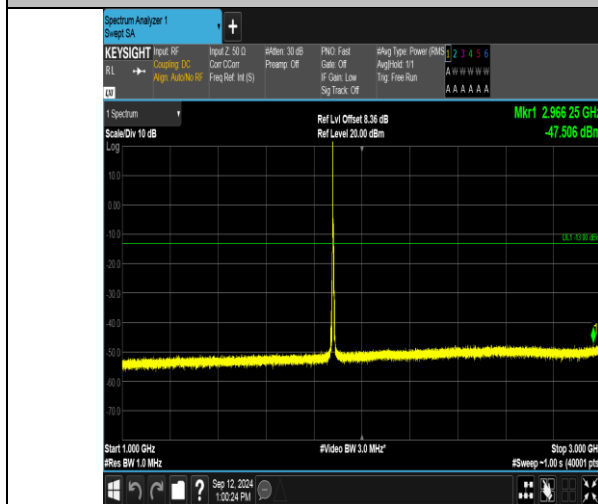
Band2_5MHz_16QAM_18900_1RB#0_1000~3000_1000~3000
