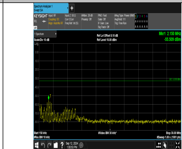
Band2_5MHz_QPSK_18900_1RB#24_0.15~30_0.15~30
