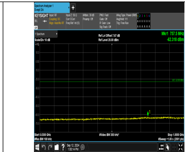
Band2_5MHz_16QAM_18900_1RB#0_30~1000_30~1000
