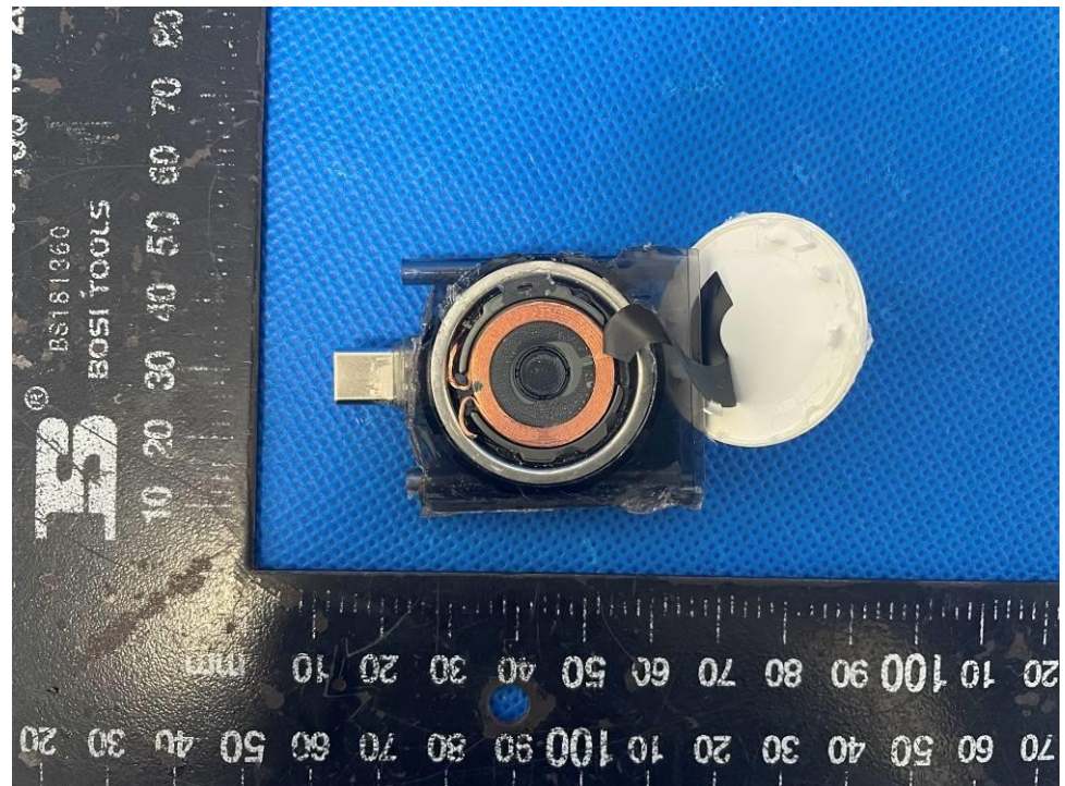
Figure 6: Internal view
