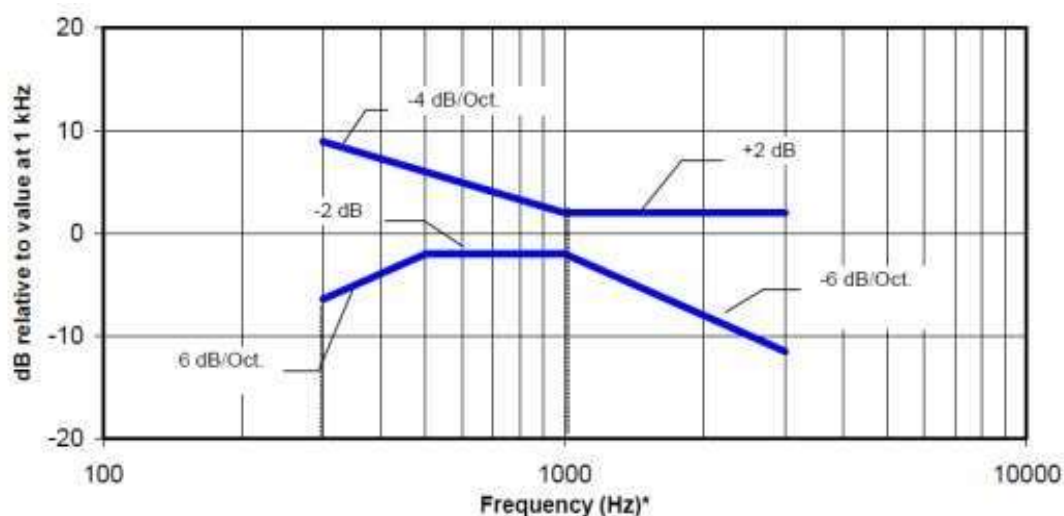
Figure 8.1—Magnetic field frequency response for WDs with field strength \leq -15 dB (A/m) at 1 kHz
