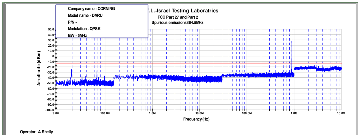
Figure 472: Spurious Emissions at Antenna Terminal QPSK, 864.5MHz, B.W. 5MHz
