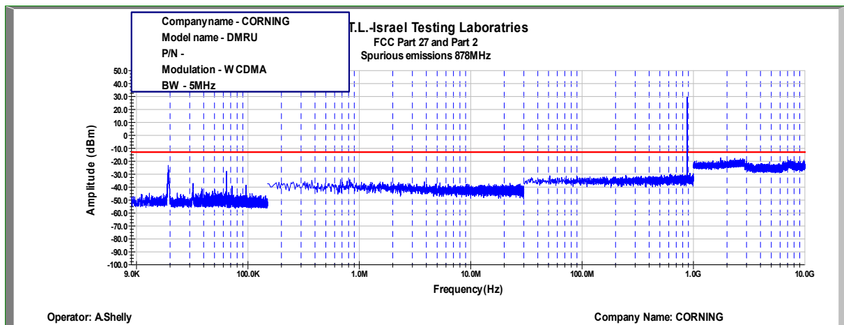
Figure 482: Spurious Emissions at Antenna Terminal WCDMA, 878.0MHz, B.W. 5MHz
