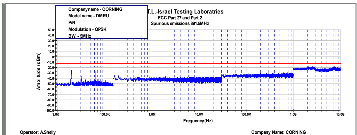
Figure 474: Spurious Emissions at Antenna Terminal QPSK, 891.5MHz, B.W. 5MHz
