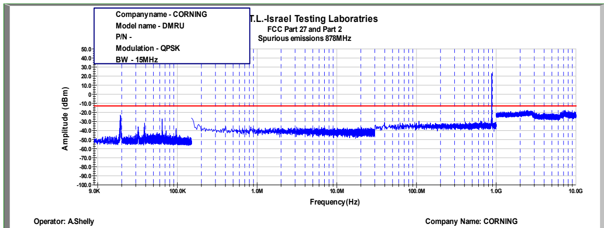
Figure 479: Spurious Emissions at Antenna Terminal QPSK, 878.0MHz, B.W. 15MHz
