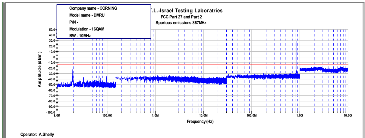
Figure 457: Spurious Emissions at Antenna Terminal 16QAM, 867.0MHz, B.W. 10MHz
