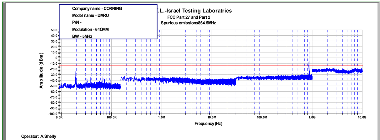
Figure 463: Spurious Emissions at Antenna Terminal 64QAM, 864.5MHz, B.W. 5MHz
