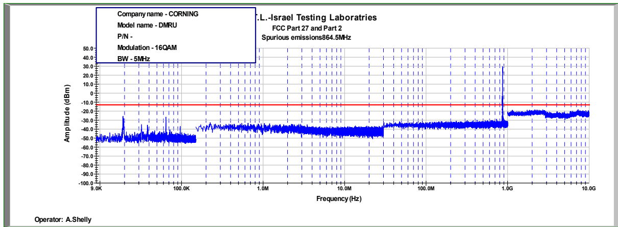
Figure 454: Spurious Emissions at Antenna Terminal 16QAM, 864.5MHz, B.W. 5MHz
