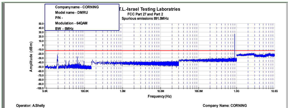
Figure 465: Spurious Emissions at Antenna Terminal 64QAM, 891.5MHz, B.W. 5MHz
