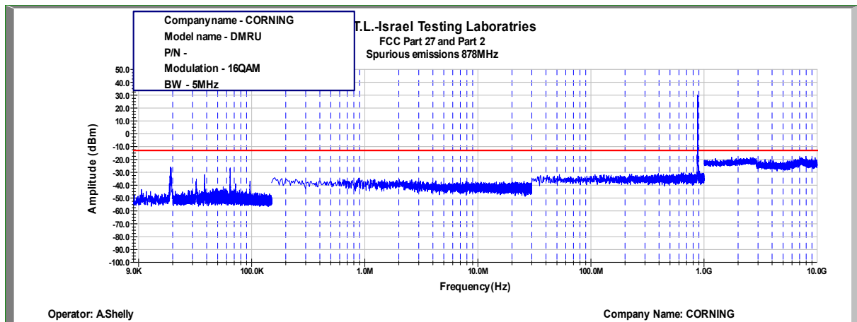
Figure 455: Spurious Emissions at Antenna Terminal 16QAM, 878.0MHz, B.W. 5MHz
