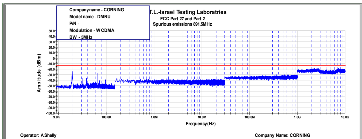
Figure 483: Spurious Emissions at Antenna Terminal WCDMA, 891.5MHz, B.W. 5MHz
