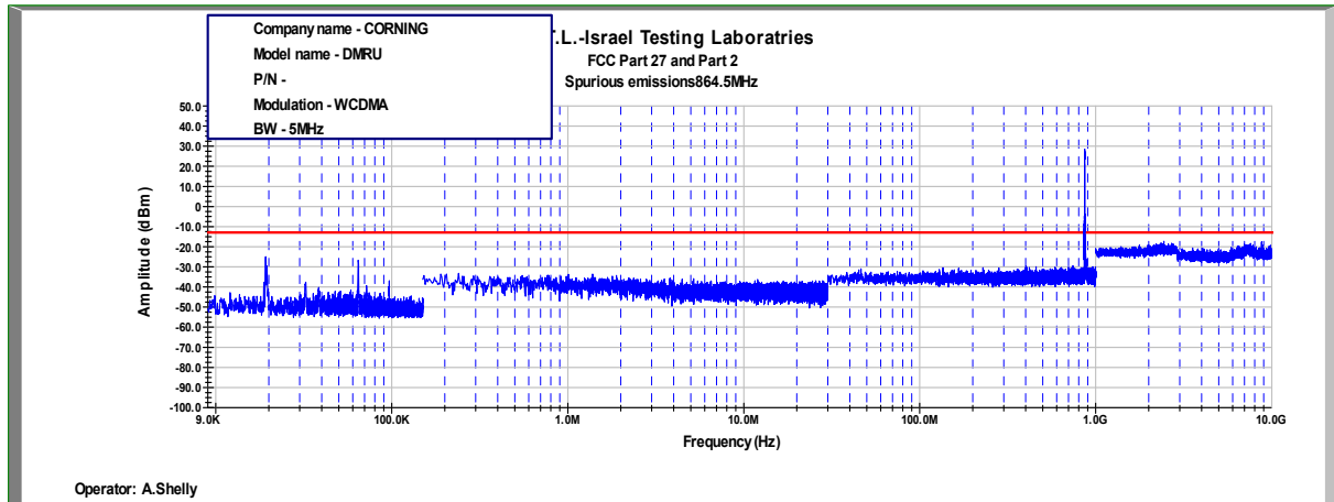
Figure 481: Spurious Emissions at Antenna Terminal WCDMA, 864.5MHz, B.W. 5MHz
