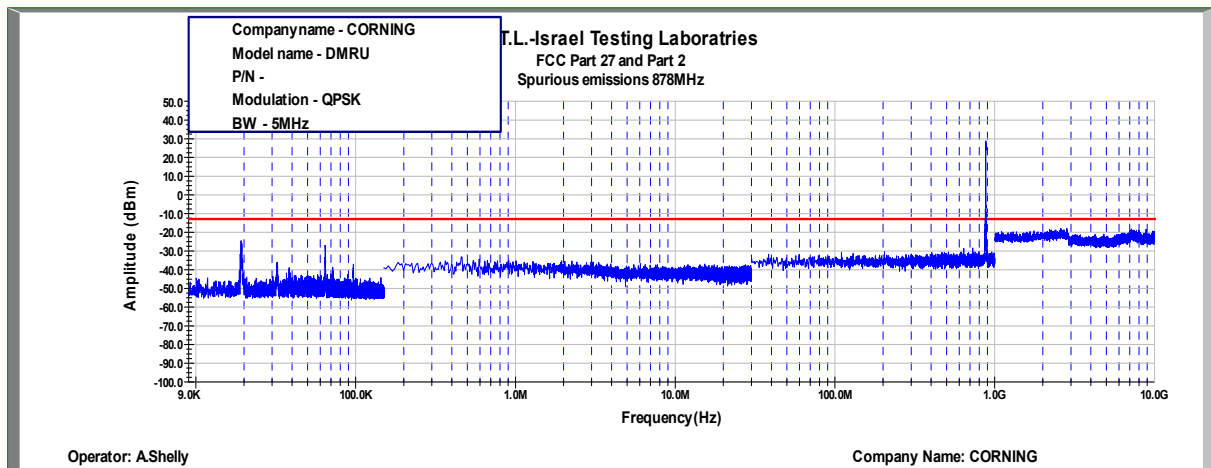
Figure 473: Spurious Emissions at Antenna Terminal QPSK, 878.0MHz, B.W. 5MHz
