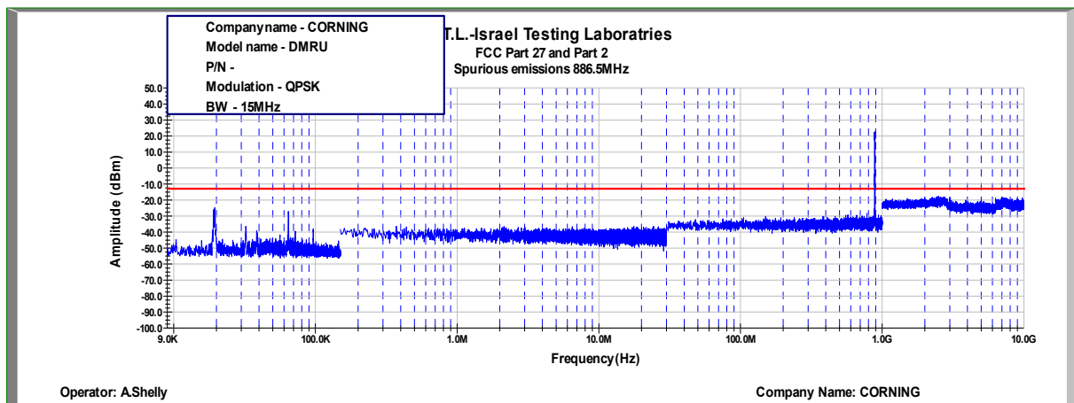
Figure 480: Spurious Emissions at Antenna Terminal QPSK, 886.5MHz, B.W. 15MHz
