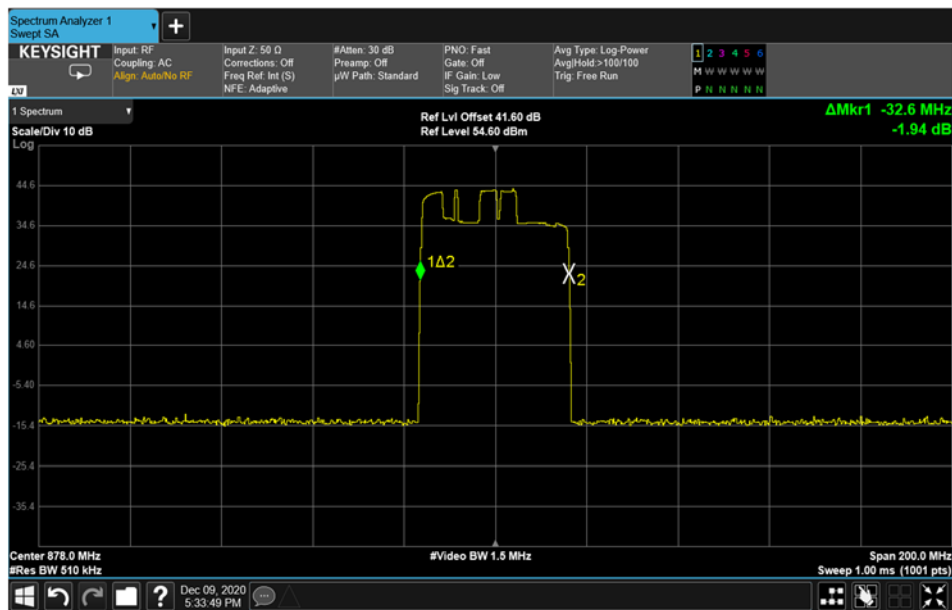
Figure 484. — Out-of-Band Rejection Plot
