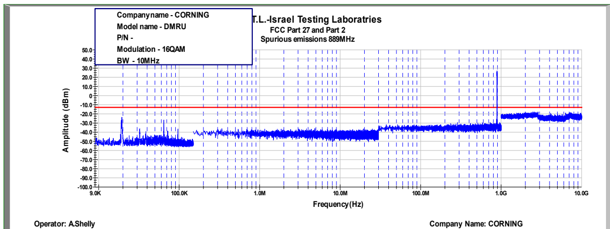
Figure 459: Spurious Emissions at Antenna Terminal 16QAM, 889.0MHz, B.W. 10MHz
