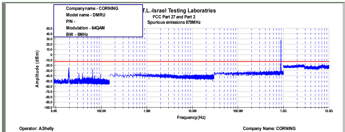
Figure 464: Spurious Emissions at Antenna Terminal 64QAM, 878.0MHz, B.W. 5MHz
