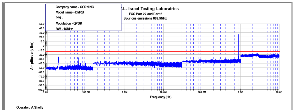
Figure 478: Spurious Emissions at Antenna Terminal QPSK, 869.5MHz, B.W. 15MHz
