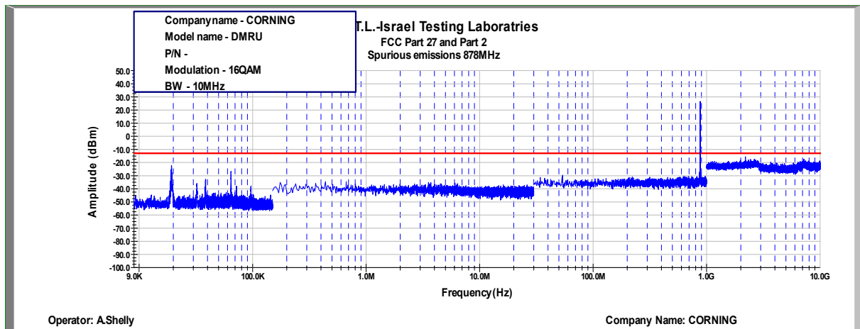
Figure 458: Spurious Emissions at Antenna Terminal 16QAM, 878.0MHz, B.W. 10MHz
