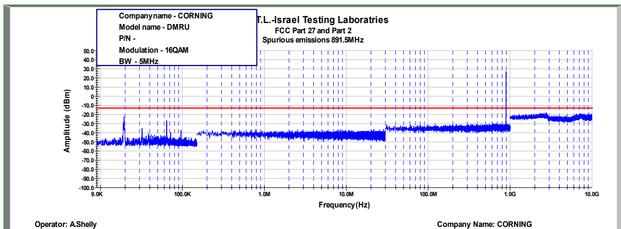
Figure 456: Spurious Emissions at Antenna Terminal 16QAM, 891.5MHz, B.W. 5MHz
