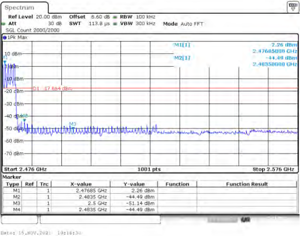
Hopping mode
