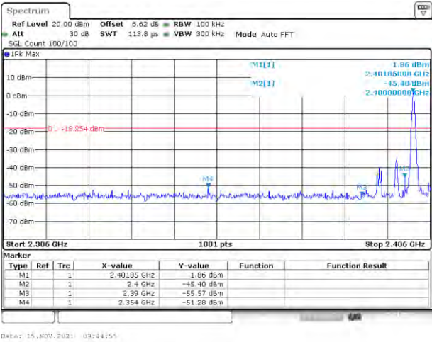
No-hopping mode
