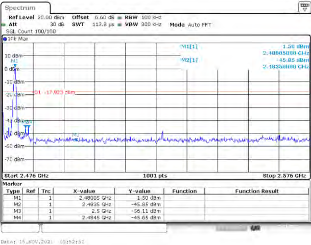
No-hopping mode
