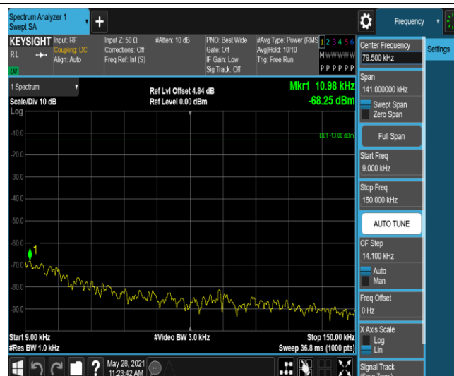
Band7-10MHz-16QAM-21100-1RB#0-Range2:0.15~30MHz
