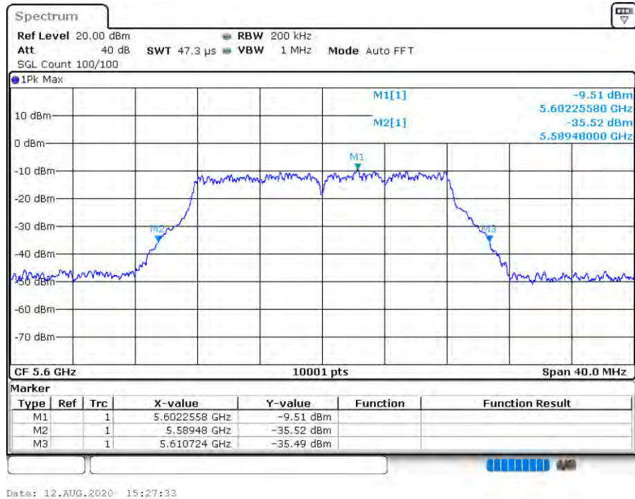
-26 dB BW NVNT 802.11a 5600MHz Ant 1
