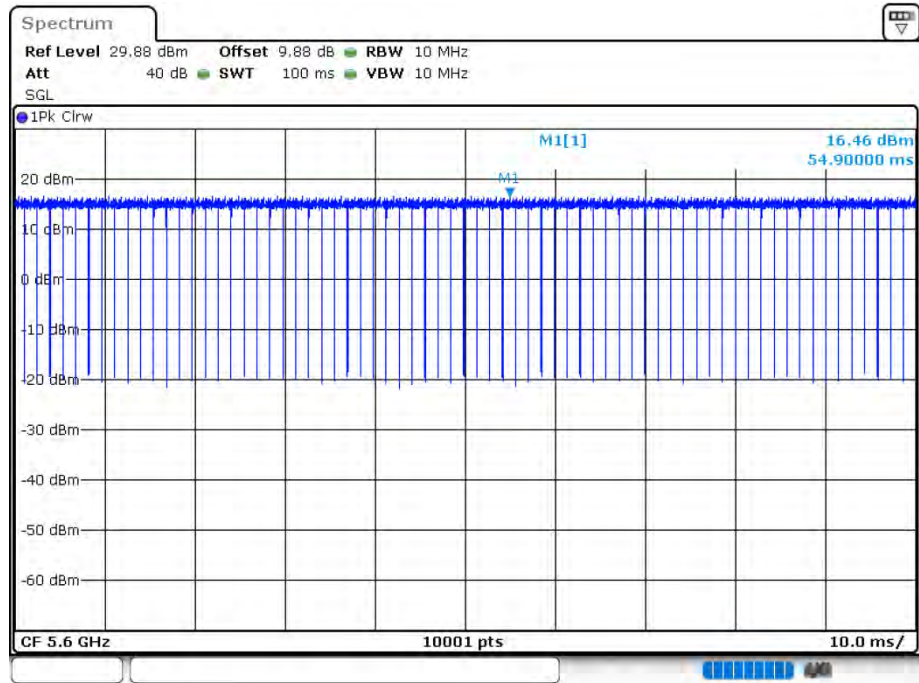
Duty Cycle NVNT 802.11a 5600MHz Ant 2
