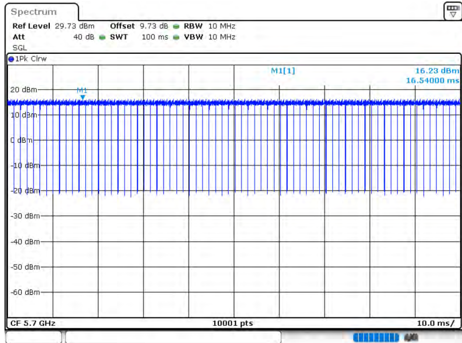
Duty Cycle NVNT 802.11a 5700MHz Ant 2
