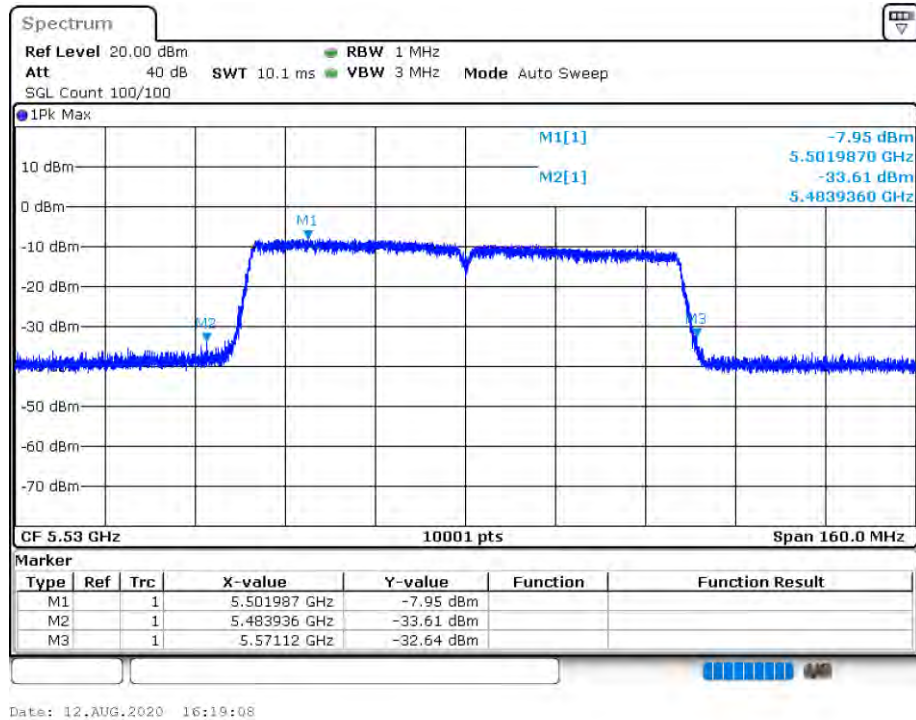
-26 dB BW NVNT 802.11ac80 5530MHz Ant 2
