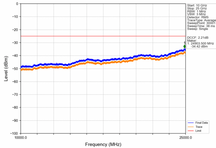
Band38_5MHz_QPSK_HCH_2617.5MHz_RB_1_0_NTNV
