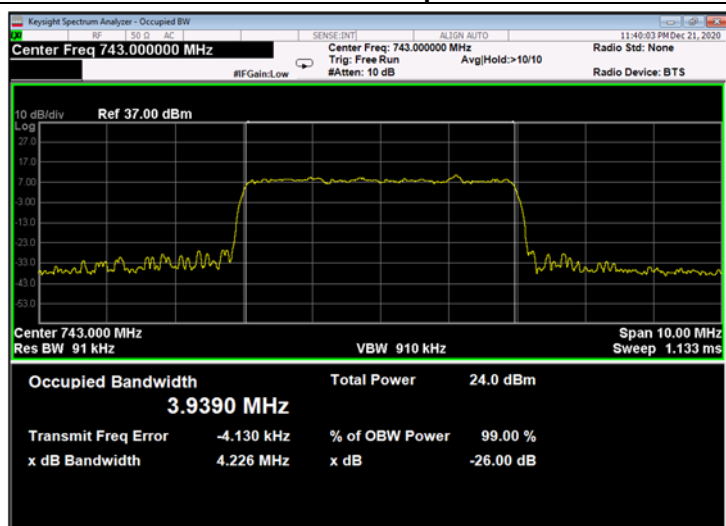
Figure 309: 64QAM 5MHz B.W.; 743.0MHz, 30kHz - Output
