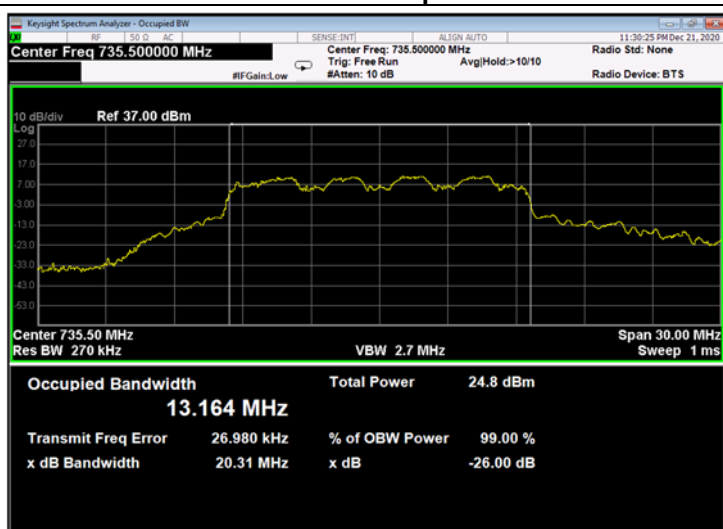
Figure 290: 16QAM 15MHz B.W.; 735.5MHz, 60kHz - Output
