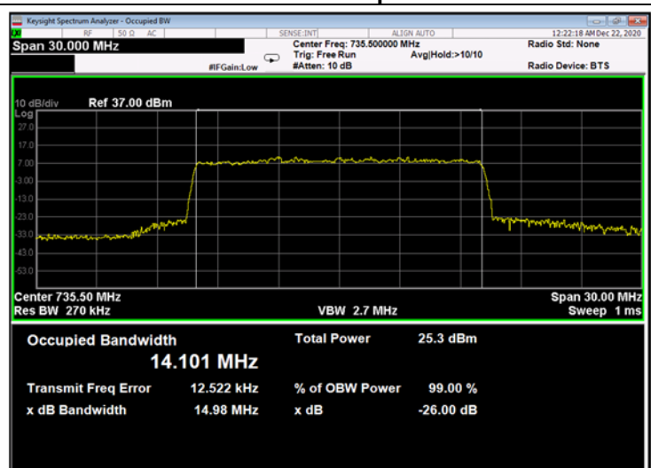
Figure 321: 64QAM 15MHz B.W.; 735.5MHz, 15kHz - Output
