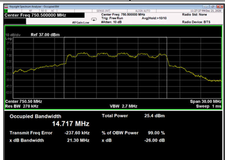
Figure 294: 16QAM 15MHz B.W.; 750.5MHz, 15kHz - Output
