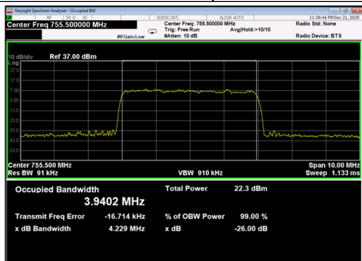
Figure 311: 64QAM 5MHz B.W.; 755.5MHz, 30kHz - Output
