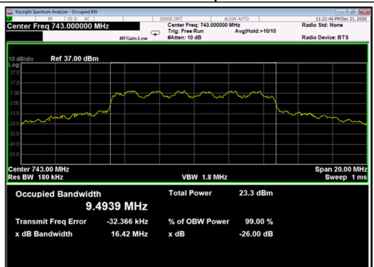
Figure 282: 16QAM 10MHz B.W.; 743.0MHz, 15kHz- Output
