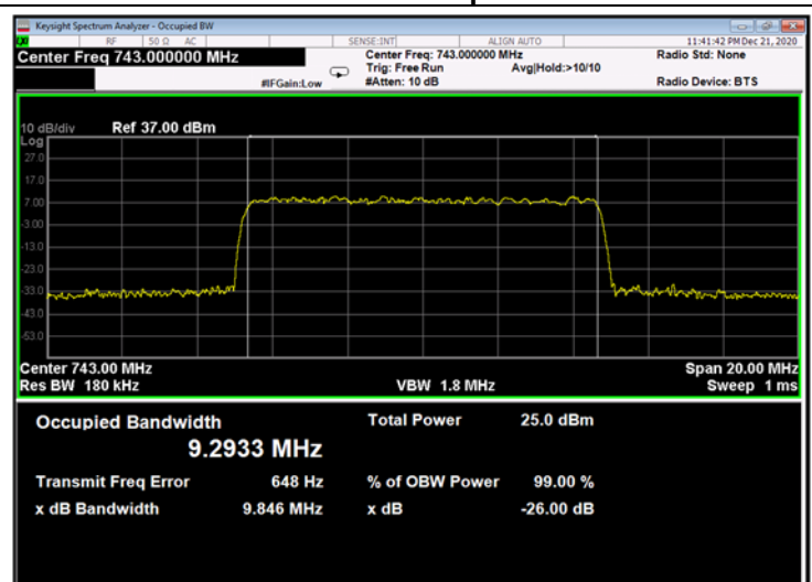
Figure 315: 64QAM 10MHz B.W.; 743.0MHz, 15kHz - Output
