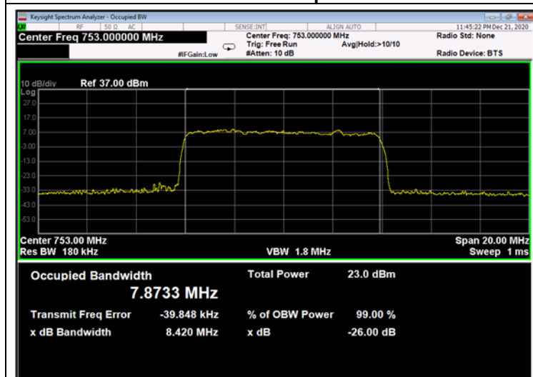
Figure 320: 64QAM 10MHz B.W.; 753.0MHz, 60kHz - Output
