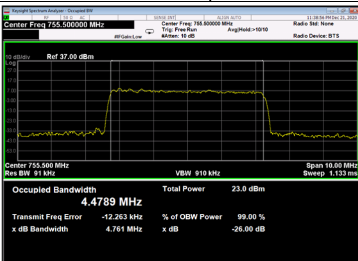
Figure 310: 64QAM 5MHz B.W.; 755.5MHz, 15kHz - Output
