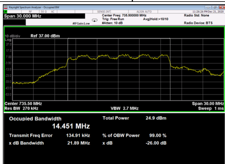
Figure 288: 16QAM 15MHz B.W.; 735.5MHz, 15kHz - Output
