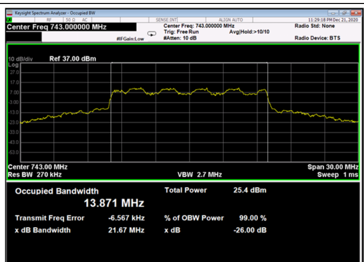
Figure 292: 16QAM 15MHz B.W.; 743.0MHz, 30kHz- Output
