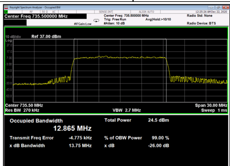
Figure 323: 64QAM 15MHz B.W.; 735.5MHz, 60kHz - Output
