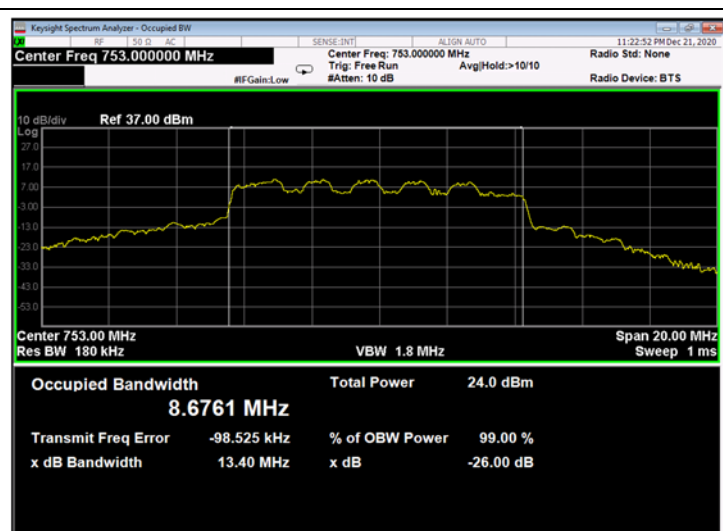
Figure 286: 16QAM 10MHz B.W.; 753.MHz, 30kHz - Output
