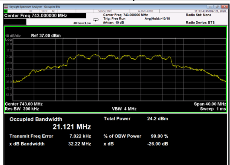
Figure 300: 16QAM 20MHz B.W.; 743.0MHz, 15kHz - Output
