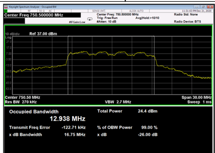
Figure 296: 16QAM 15MHz B.W.; 750.5MHz, 60kHz - Output
