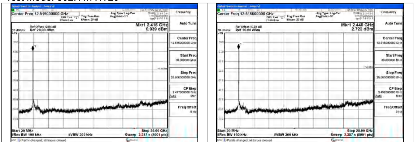
Test Mode:802.11n HT20 2412MHz Chain0
