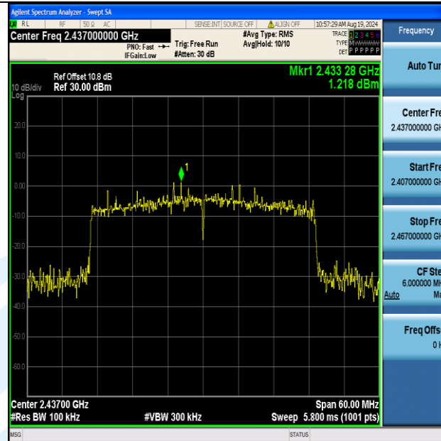
11AX40MIMO-Ant2-2437-0-Reference-PASS
