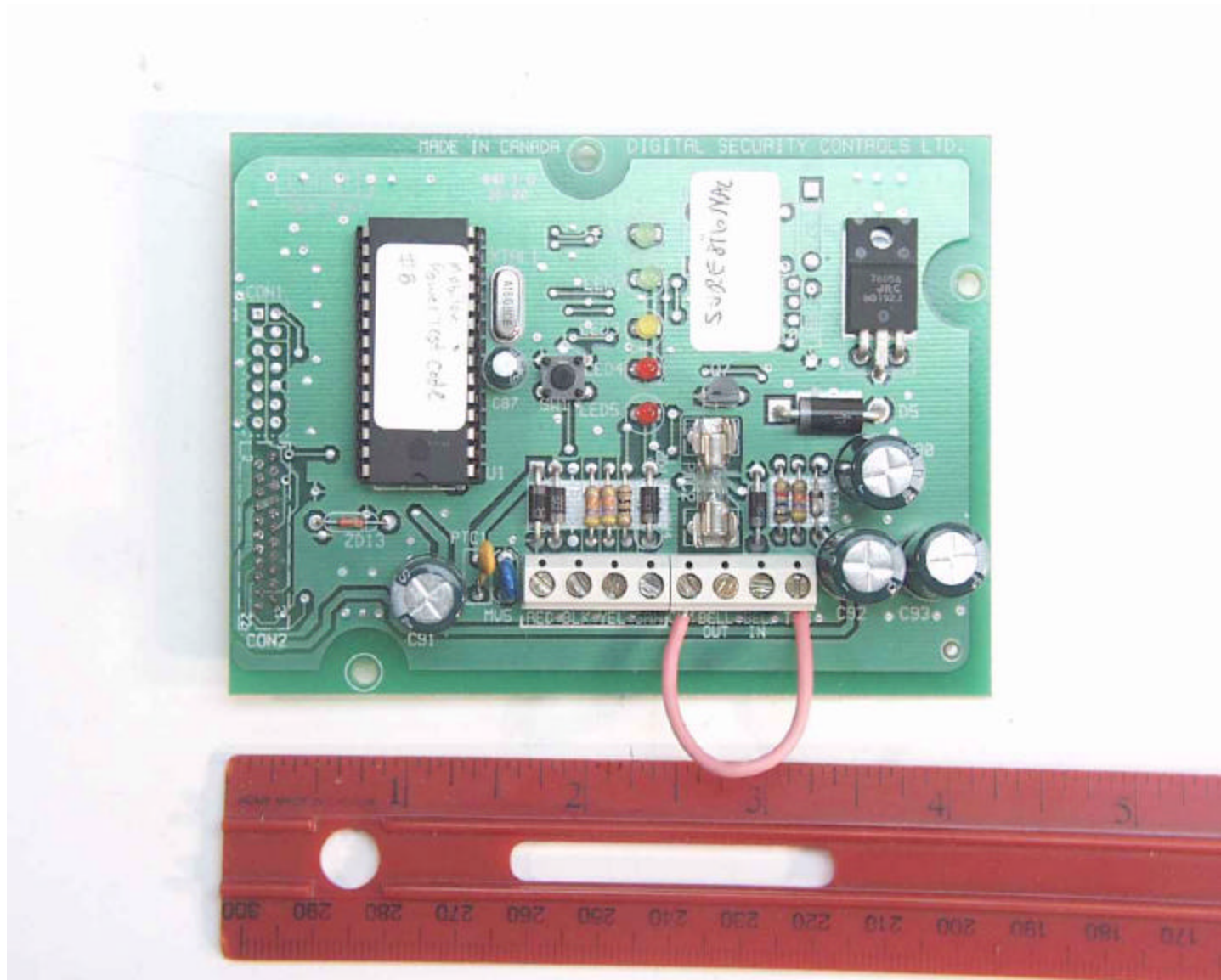
S-G I/O Communication Board (Top View)
