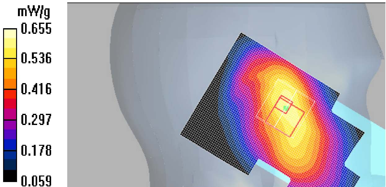
Fig.5 WCDMA 850 CH4132
