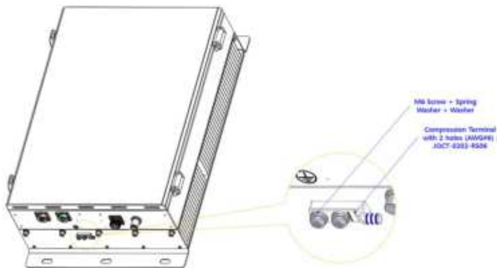
Figure 24. Location of Ground Terminal
