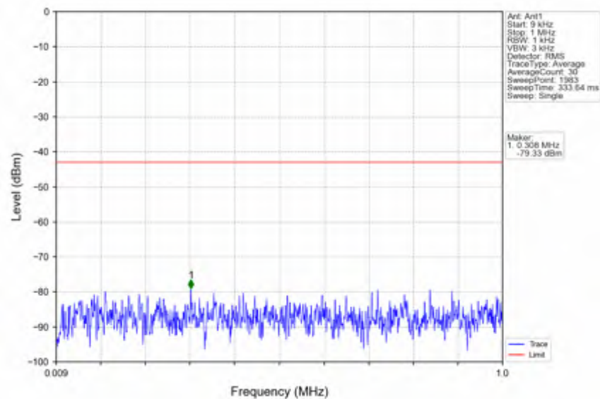
n66_30kHz_SISO_NTNV_25MHz_CP-OFDM_QPSK_1767.5MHz_Outer_Full
