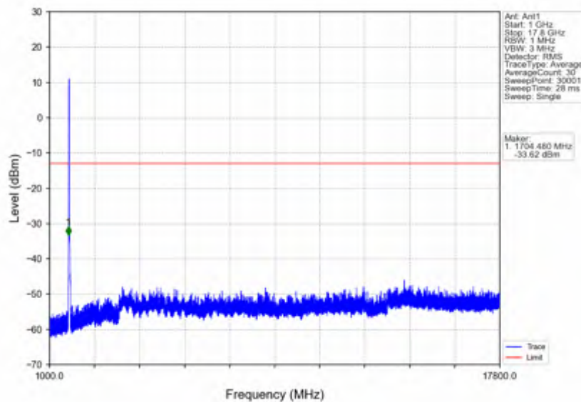
n66_30kHz_SISO_NTNV_25MHz_DFT-s-OFDM_QPSK_1722.5MHz_Inner_1RB_Left
