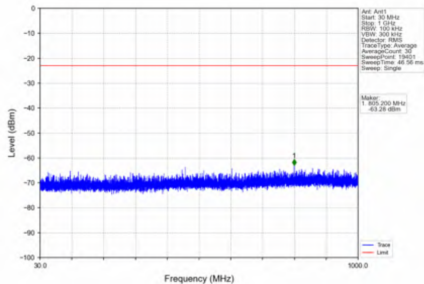
n66_30kHz_SISO_NTNV_30MHz_DFT-s-OFDM QPSK_1765MHz_Edge_1RB_Right
