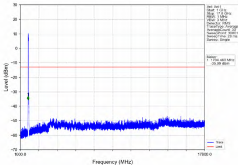
n66_30kHz_SISO_NTNV_40MHz_DFT-s-OFDM_PI/2_BPSK_1730MHz_Outer_Full
