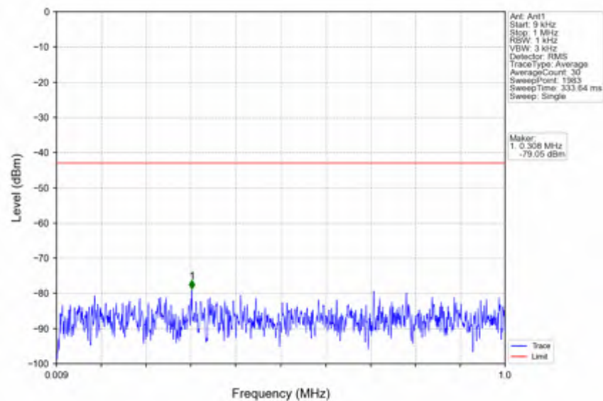
n66_30kHz_SISO_NTNV_25MHz_CP-OFDM_QPSK_1722.5MHz_Outer_Full
