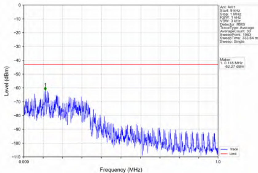
n66_30kHz_SISO_NTNV_30MHz_DFT-s-OFDM_PI/2_BPSK_1765MHz_Edge_1RB_Right
