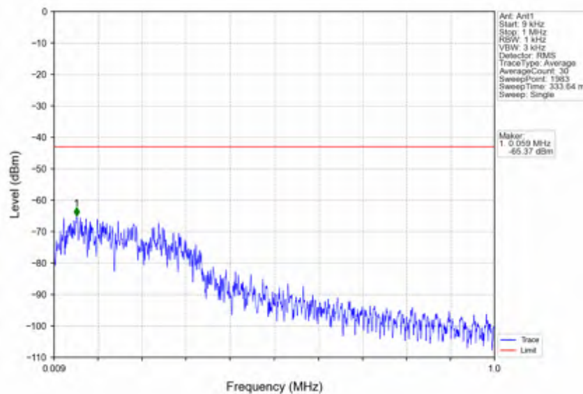
n66_30kHz_SISO_NTNV_30MHz_CP-OFDM QPSK_1765MHz_Edge_1RB_Right
