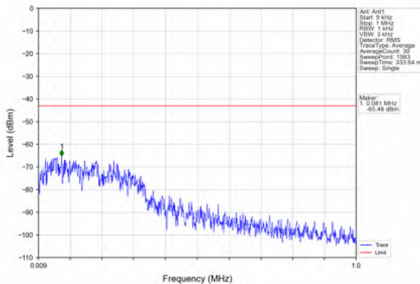
n66_30kHz_SISO_NTNV_25MHz_CP-OFDM QPSK_1767.5MHz_Edge_1RB_Right
