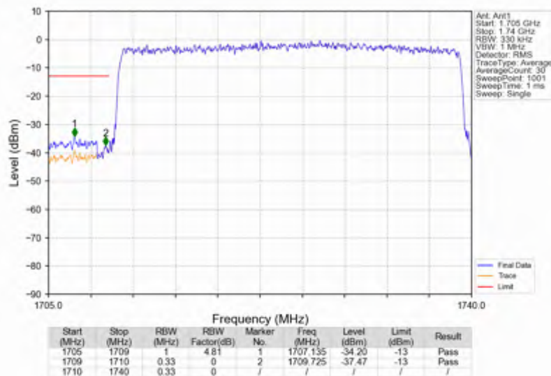
n66_30kHz_SISO_NTNV_30MHz_CP-OFDM QPSK_1725MHz_Outer_Full
