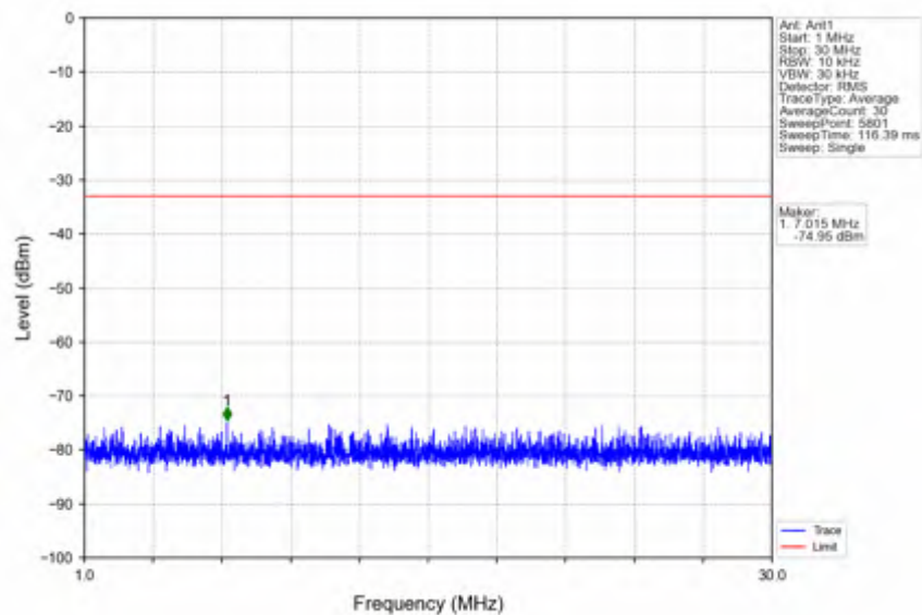
n66_30kHz_SISO_NTNV_40MHz_DFT-s-OFDM PI/2 BPSK_1730MHz_Edge_1RB_Left
