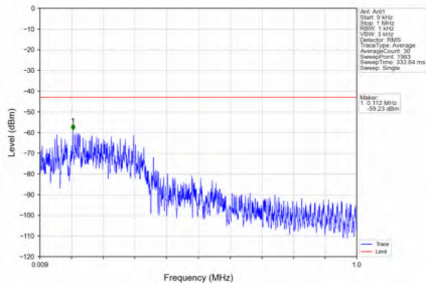
n66_30kHz_SISO_NTNV_30MHz_DFT-s-OFDM_QPSK_1725MHz_Inner_1RB_Left
