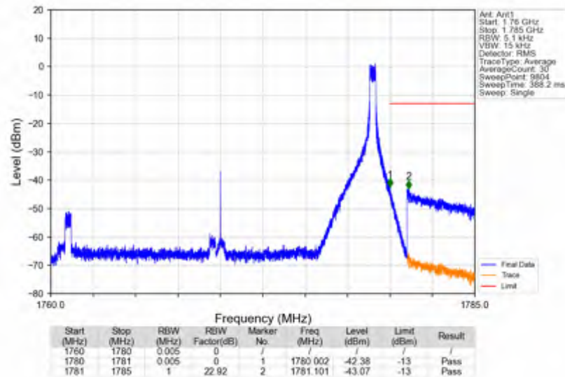
n66_30kHz_SISO_NTNV_20MHz_CP-OFDM QPSK_1770MHz_Edge_1RB_Right
