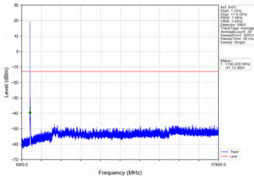
n66_30kHz_SISO_NTNV_25MHz_CP-OFDM QPSK_1745MHz_Edge_1RB_Left
