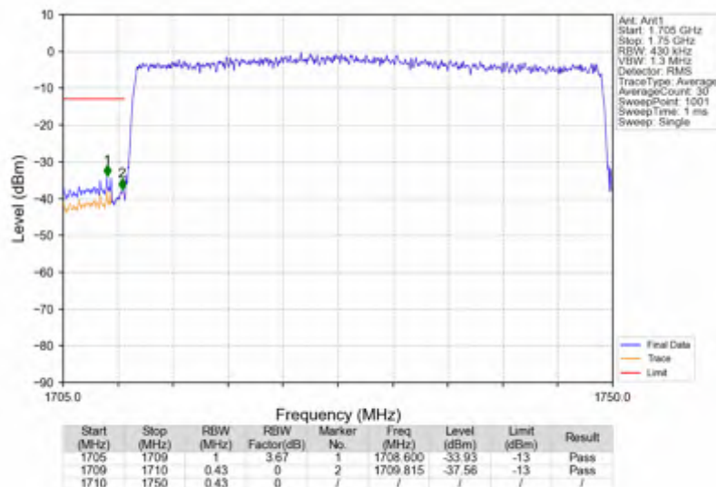
n66_30kHz_SISO_NTNV_40MHz_CP-OFDM QPSK_1730MHz_Outer_Full
