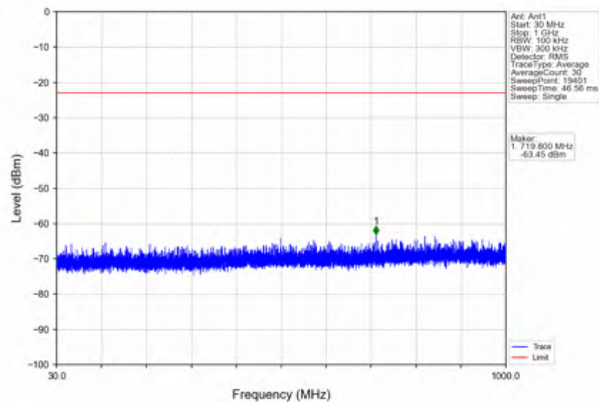
n66_30kHz_SISO_NTV_30MHz_CP-OFDM_QPSK_1765MHz_Outer_Full
