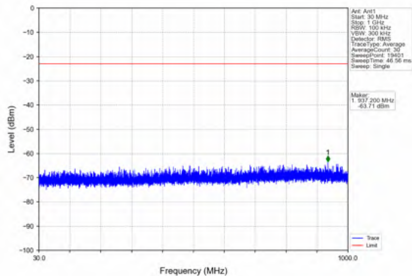
n66_30kHz_SISO_NTNV_30MHz_DFT-s-OFDM_QPSK_1725MHz_Inner_1RB_Left
