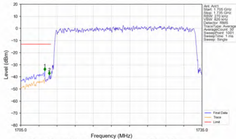
n66_30kHz_SISO_NTNV_25MHz_DFT-s-OFDM PI/2 BPSK_1722.5MHz_Outer_Full
