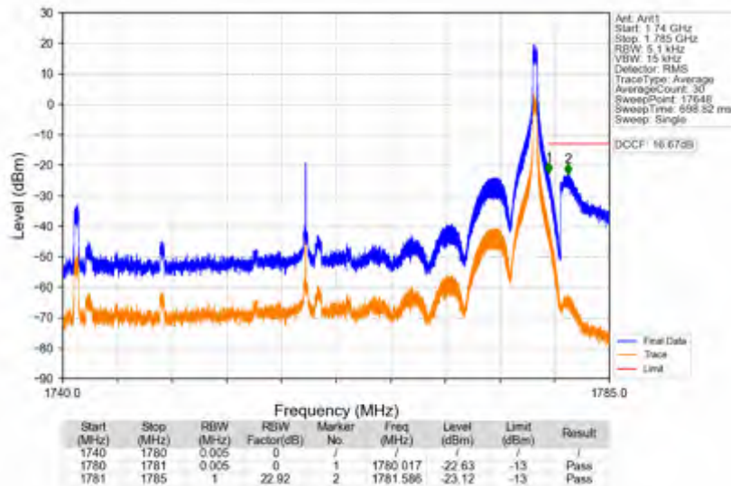
n66_30kHz_SISO_NTNV_40MHz_DFT-s-OFDM QPSK_1760MHz_Edge_1RB_Right
