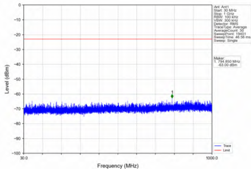
n66_30kHz_SISO_NTNV_30MHz_DFT-s-OFDM QPSK_1745MHz_Edge_1RB_Left
