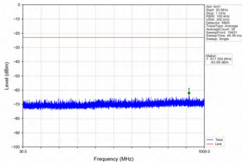
n66_30kHz_SISO_NTNV_25MHz_CP-OFDM QPSK_1767.5MHz_Outer_Full
