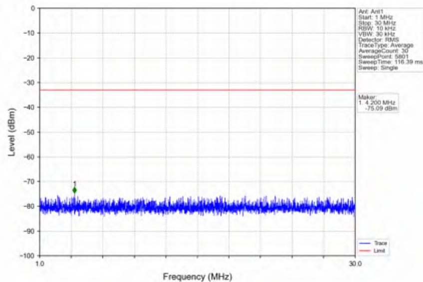
n66_30kHz_SISO_NTNV_40MHz_DFT-s-OFDM QPSK_1745MHz_Edge_1RB_Left
