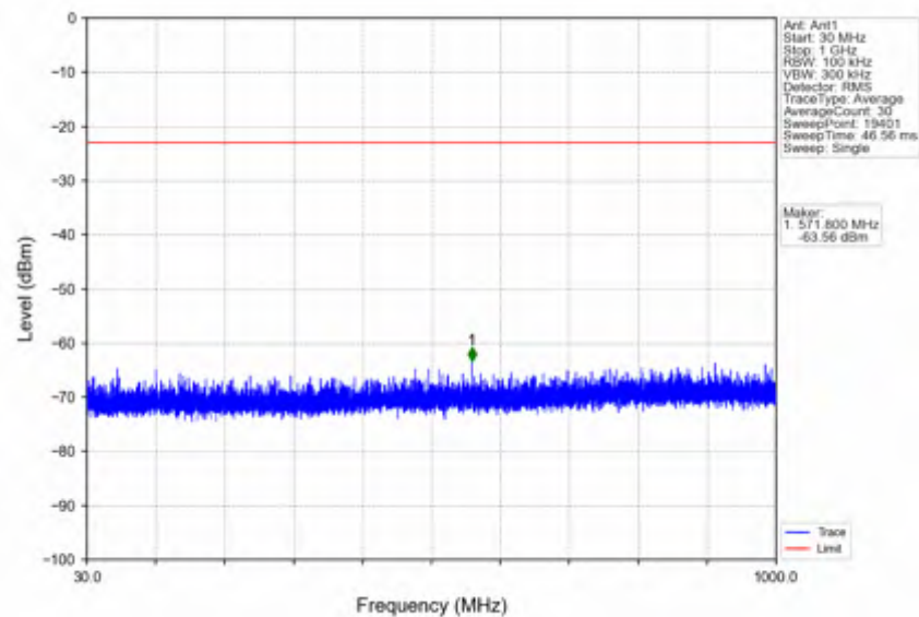
n66_30kHz_SISO_NTNV_40MHz_DFT-s-OFDM_QPSK_1730MHz_Edge_1RB_Left
