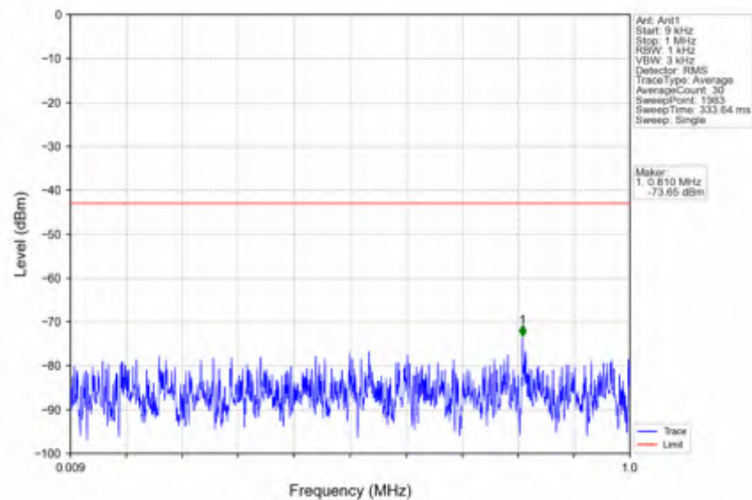
n66_30kHz_SISO_NTNV_20MHz_CP-OFDM QPSK_1720MHz_Outer_Full
