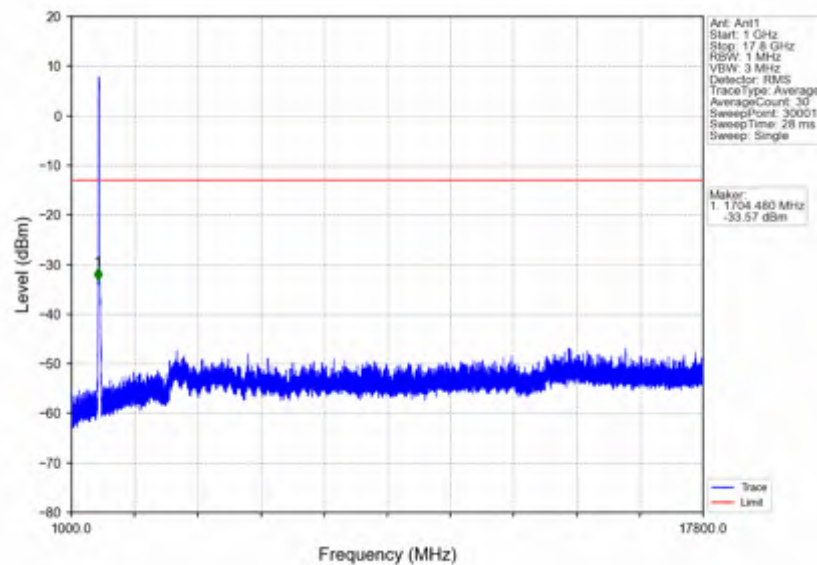
n66_30kHz_SISO_NTV_30MHz_CP-OFDM_QPSK_1725MHz_Outer_Full
