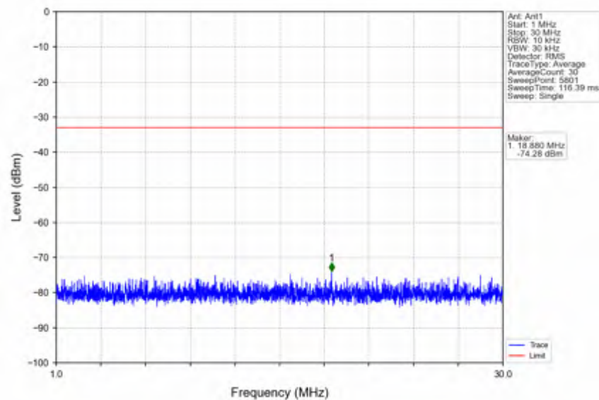
n66_30kHz_SISO_NTNV_30MHz_DFT-s-OFDM QPSK_1745MHz_Edge_1RB_Left
