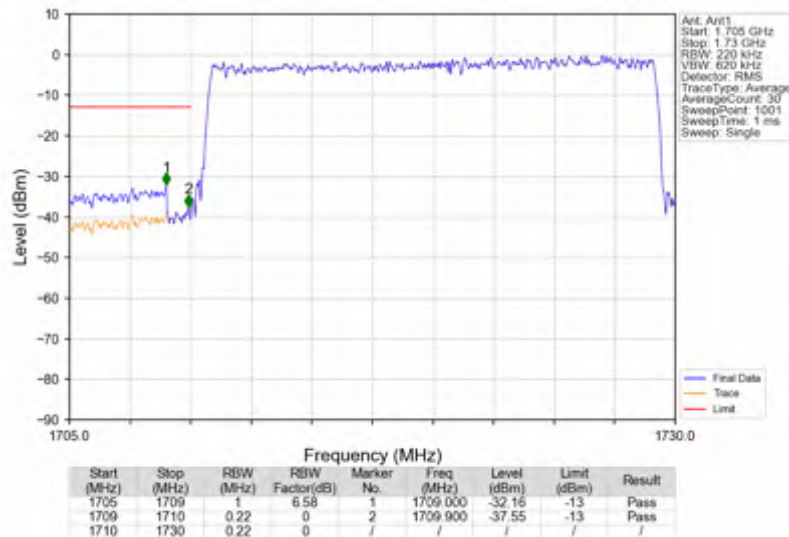
n66_30kHz_SISO_NTNV_20MHz_CP-OFDM QPSK_1720MHz_Outer_Full
