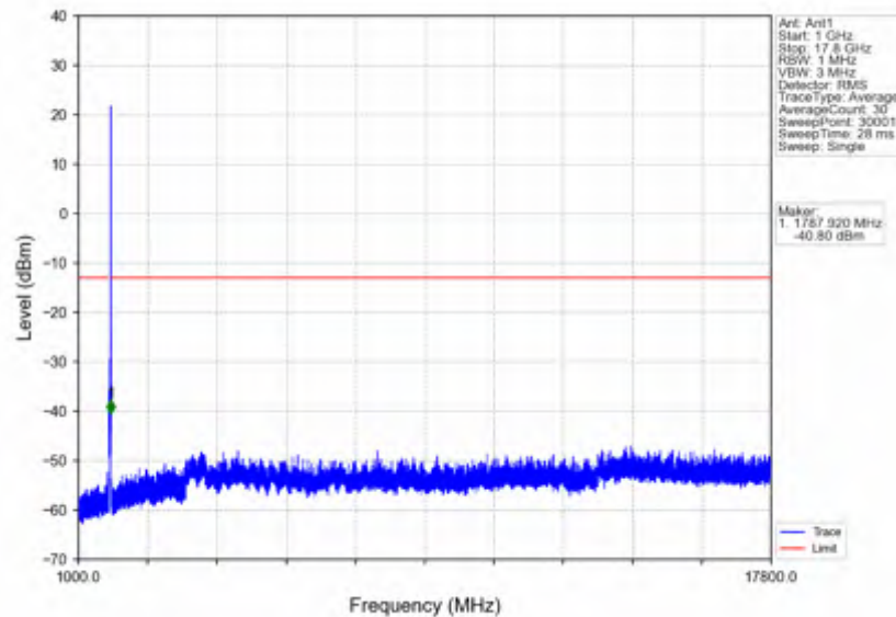
n66_30kHz_SISO_NTNV_20MHz_DFT-s-OFDM_QPSK_1770MHz_Edge_1RB_Right
