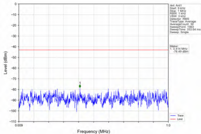
n66_30kHz_SISO_NTNV_30MHz_CP-OFDM QPSK_1765MHz_Outer_Full
