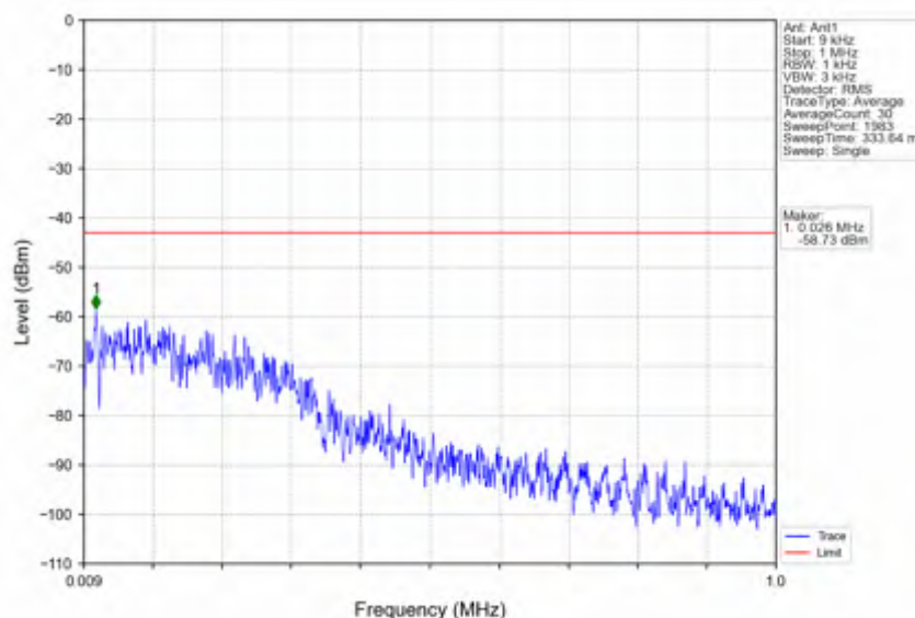
n66_30kHz_SISO_NTNV_25MHz_CP-OFDM QPSK_1767.5MHz_Inner_1RB_Right
