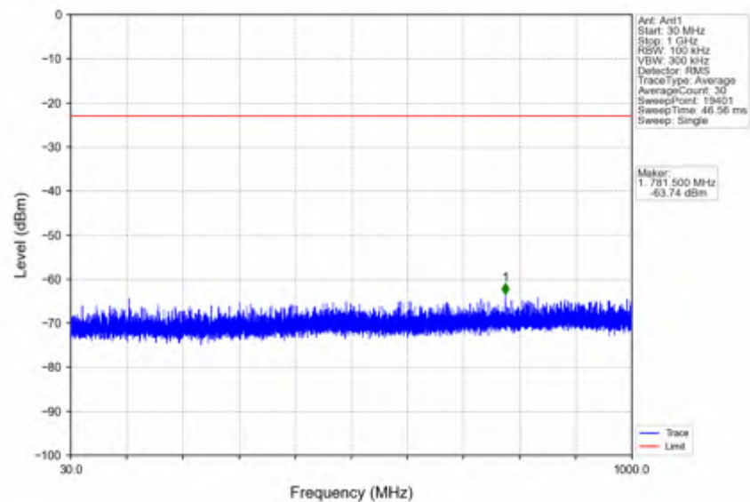
n66_30kHz_SISO_NTNV_25MHz_DFT-s-OFDM QPSK_1745MHz_Edge_1RB_Left
