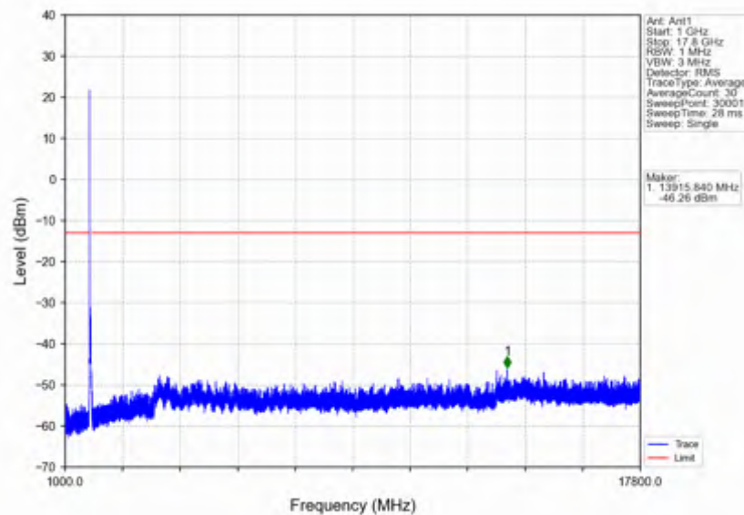
n66_30kHz_SISO_NTNV_40MHz_DFT-s-OFDM_QPSK_1730MHz_Edge_1RB_Left
