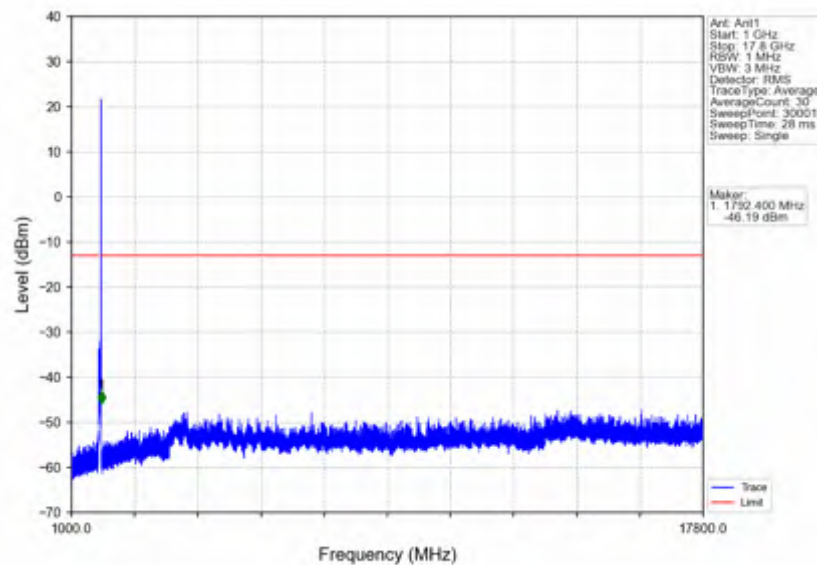
n66_30kHz_SISO_NTNV_30MHz_DFT-s-OFDM QPSK_1765MHz_Edge_1RB_Right
