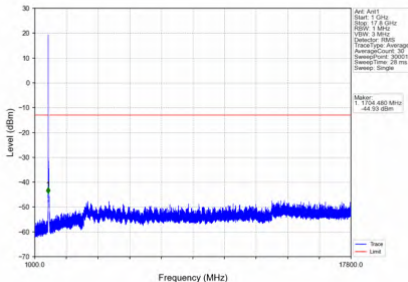
n66_30kHz_SISO_NTNV_40MHz_CP-OFDM QPSK_1730MHz_Outer_Full
