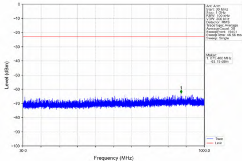
n66_30kHz_SISO_NTNV_20MHz_CP-OFDM QPSK_1720MHz_Outer_Full
