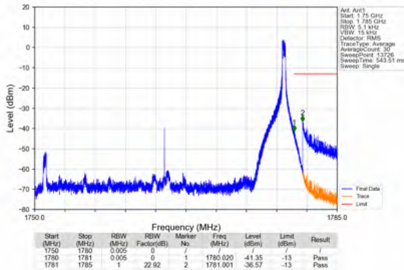
n66_30kHz_SISO_NTNV_30MHz_DFT-s-OFDM_PI/2_BPSK_1765MHz_Edge_1RB_Right
