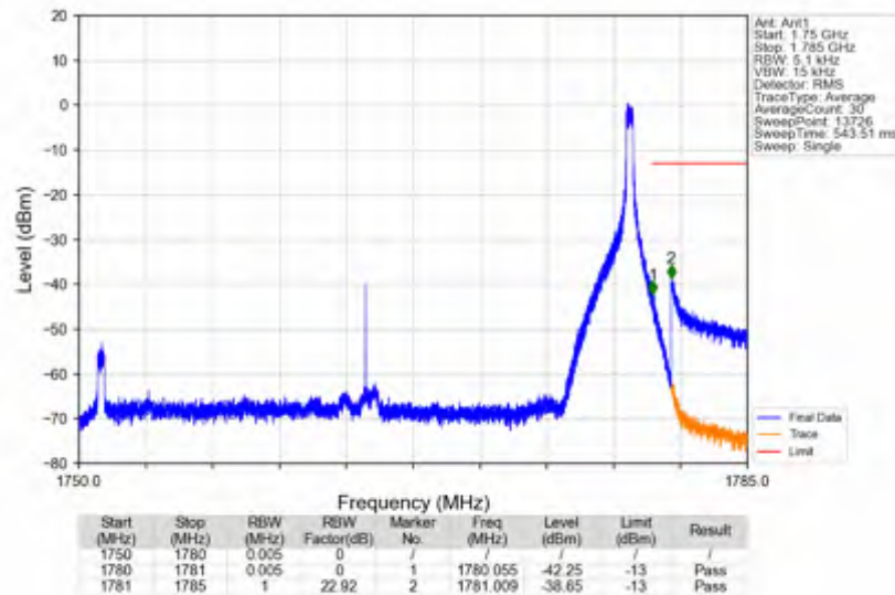
n66_30kHz_SISO_NTNV_30MHz_CP-OFDM QPSK_1765MHz_Edge_1RB_Right
