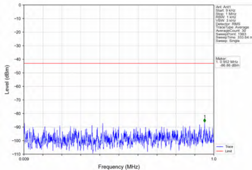
n66_30kHz_SISO_NTNV_30MHz_DFT-s-OFDM_QPSK_1725MHz_Outer_Full
