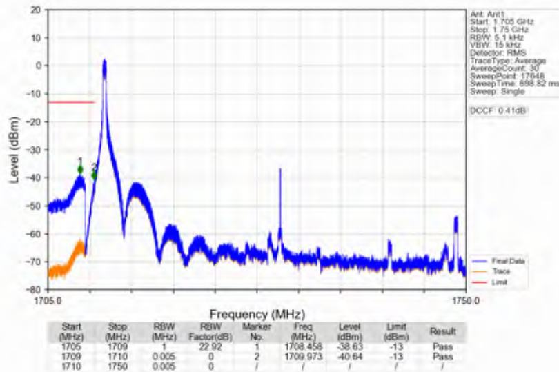
n66_30kHz_SISO_NTNV_40MHz_DFT-s-OFDM QPSK_1730MHz_Edge_1RB_Left
