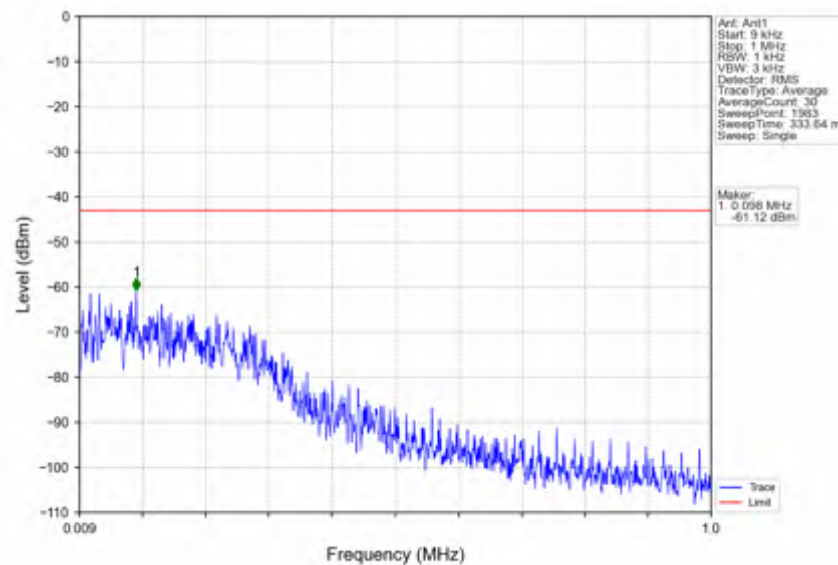
n66_30kHz_SISO_NTNV_20MHz_CP-OFDM QPSK_1770MHz_Edge_1RB_Right
