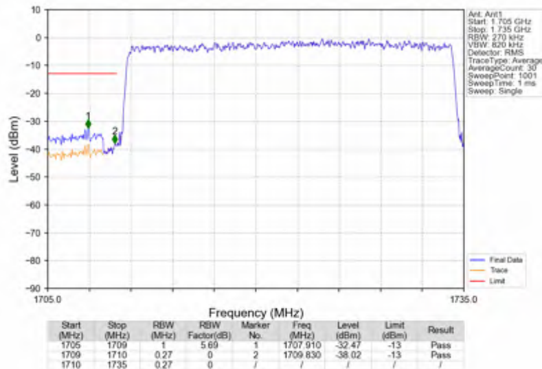
n66_30kHz_SISO_NTV_25MHz_CP-OFDM QPSK_1722.5MHz_Outer_Full
