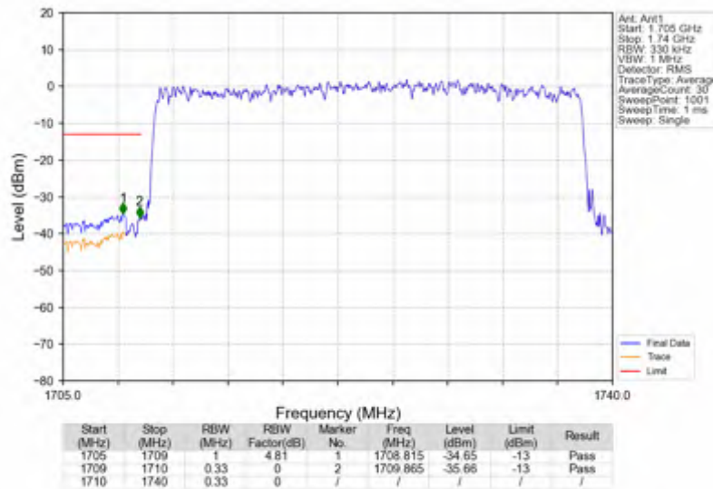
n66_30kHz_SISO_NTNV_30MHz_DFT-s-OFDM_QPSK_1725MHz_Outer_Full
