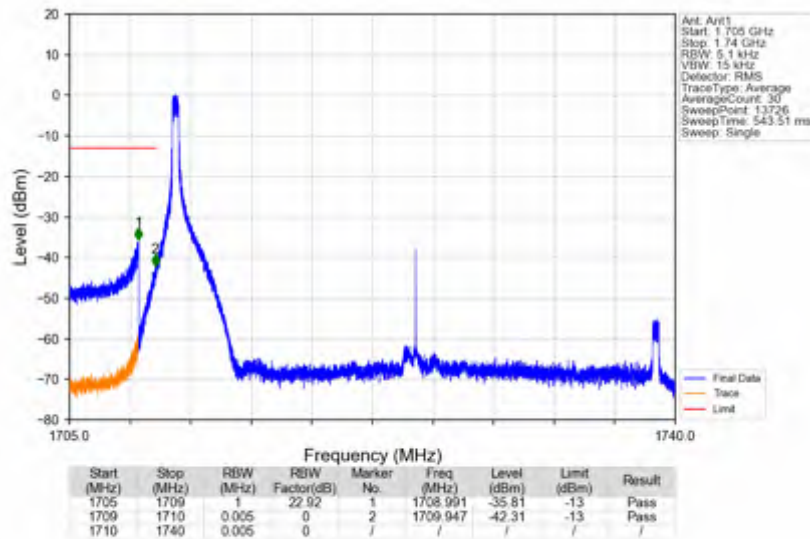
n66_30kHz_SISO_NTNV_30MHz_CP-OFDM_QPSK_1725MHz_Edge_1RB_Left
