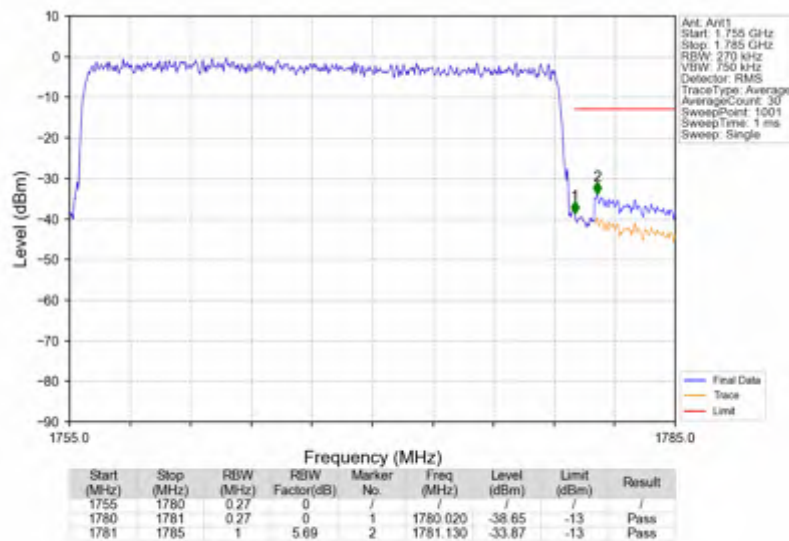
n66_30kHz_SISO_NTNV_25MHz_CP-OFDM QPSK_1767.5MHz_Outer_Full
