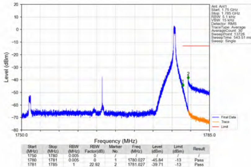
n66_30kHz_SISO_NTNV_30MHz_CP-OFDM_QPSK_1765MHz_Inner_1RB_Right
