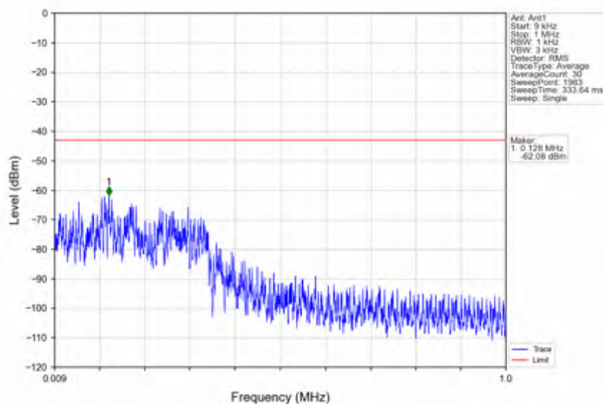
n66_30kHz_SISO_NTNV_30MHz_DFT-s-OFDM_PI/2_BPSK_1725MHz_Edge_1RB_Left
