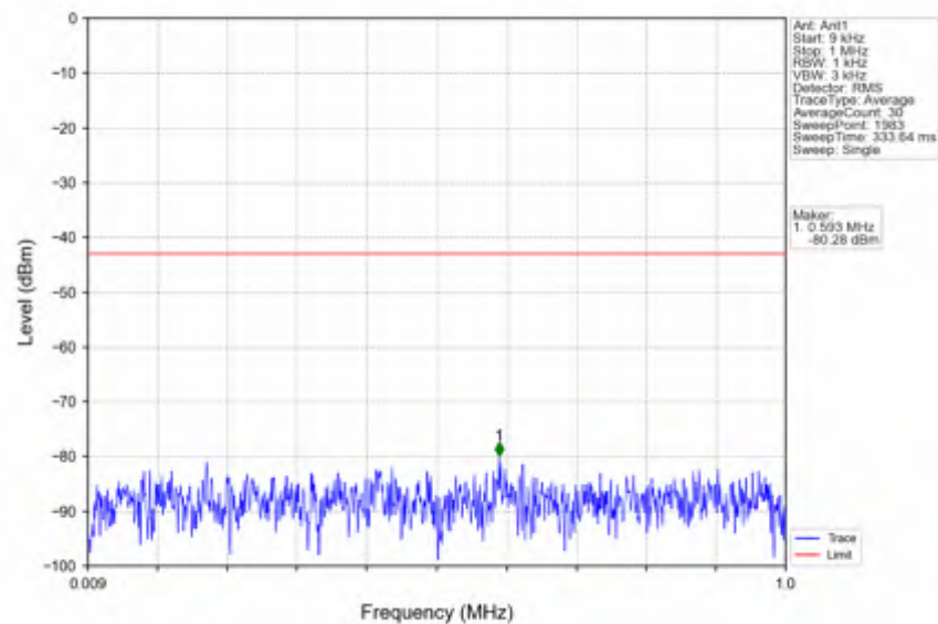
n66_30kHz_SISO_NTNV_30MHz_CP-OFDM QPSK_1725MHz_Outer_Full
