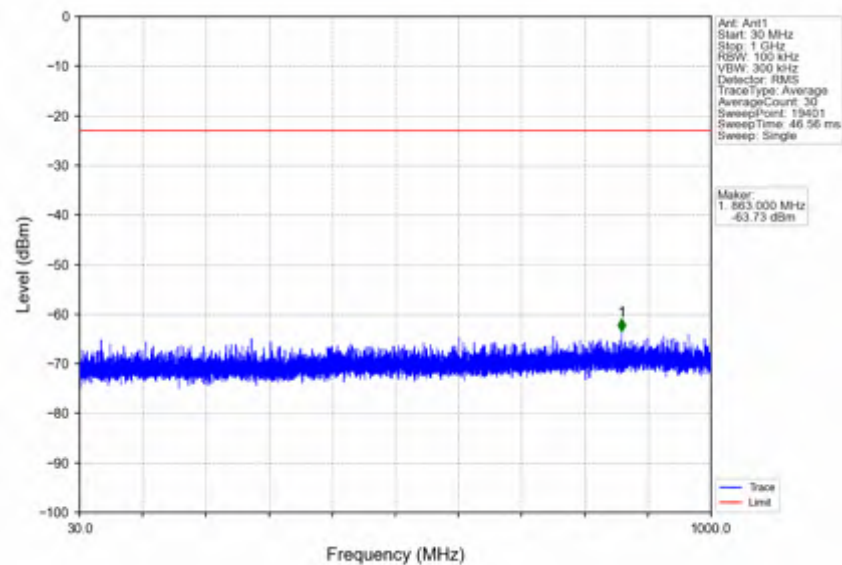
n66_30kHz_SISO_NTNV_40MHz_DFT-s-OFDM_PI/2_BPSK_1745MHz_Edge_1RB_Left
