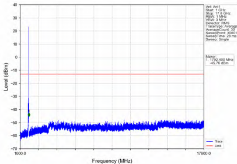
n66_30kHz_SISO_NTNV_30MHz_DFT-s-OFDM QPSK_1725MHz_Edge_1RB_Left
