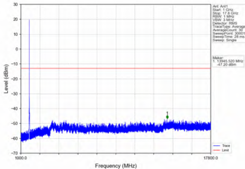
n66_30kHz_SISO_NTNV_20MHz_CP-OFDM_QPSK_1745MHz_Edge_1RB_Left
