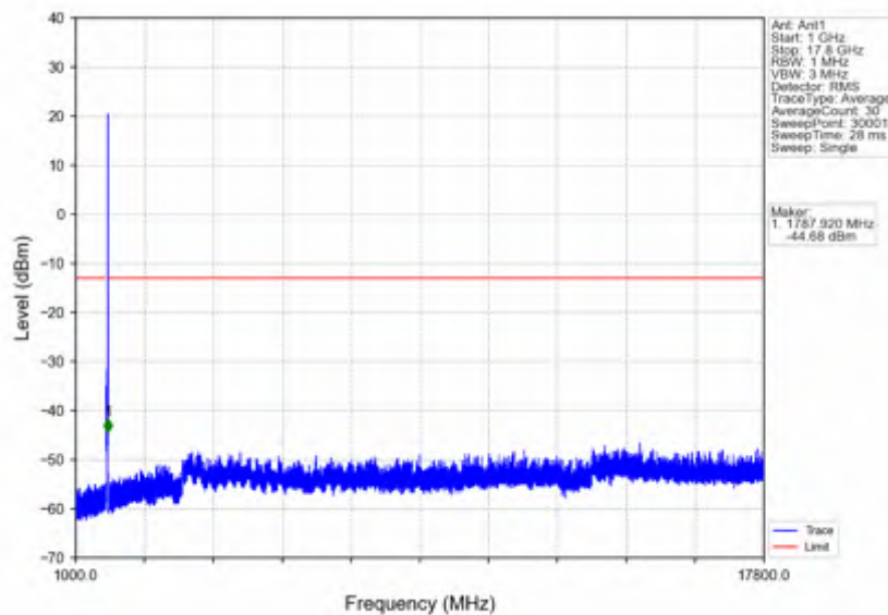
n66_30kHz_SISO_NTNV_20MHz_CP-OFDM QPSK_1770MHz_Outer_Full
