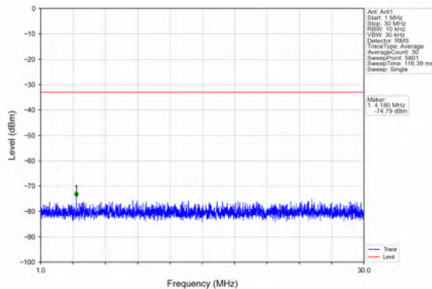
n66_30kHz_SISO_NTNV_20MHz_DFT-s-OFDM QPSK_1745MHz_Edge_1RB_Left
