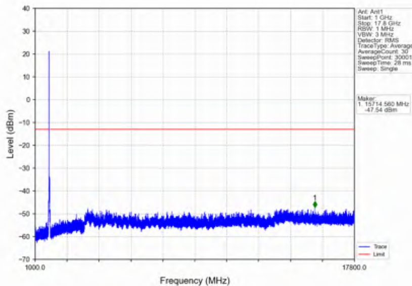
n66_30kHz_SISO_NTNV_40MHz_DFT-s-OFDM QPSK_1760MHz_Edge_1RB_Right
