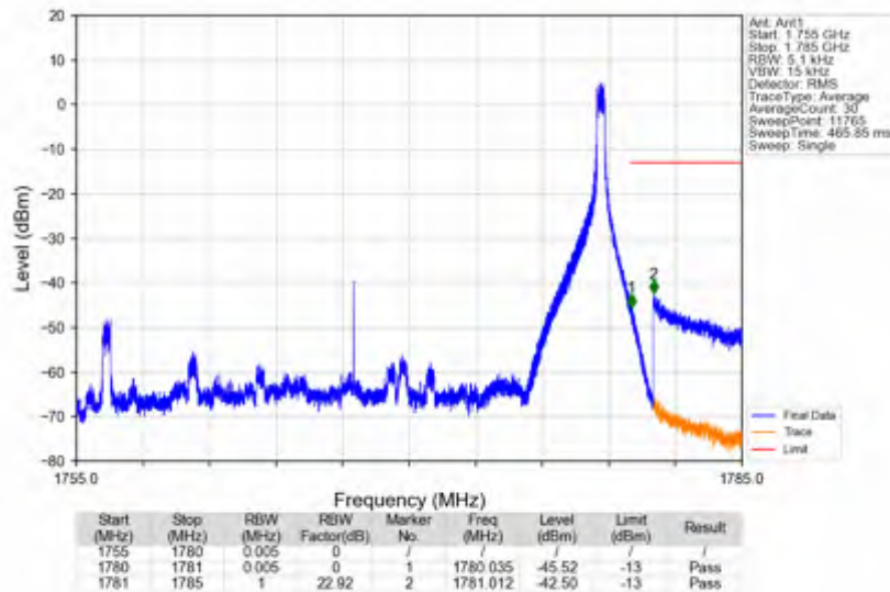
n66_30kHz_SISO_NTNV_25MHz_DFT-s-OFDM QPSK_1767.5MHz_Inner_1RB_Right
