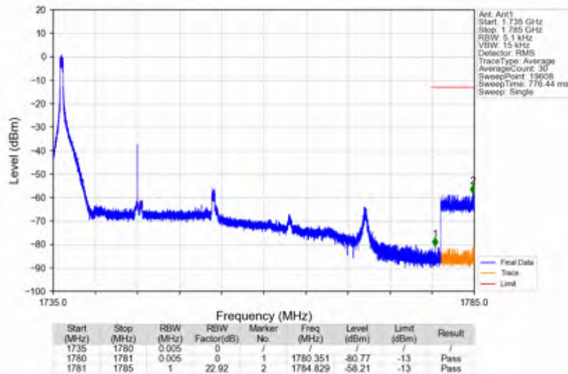
n66_30kHz_SISO_NTNV_20MHz_CP-OFDM_QPSK_1745MHz_Edge_1RB_Left
