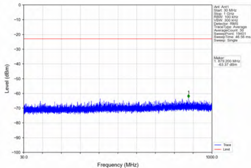
n66_30kHz_SISO_NTNV_30MHz_CP-OFDM QPSK_1765MHz_Edge_1RB_Right
