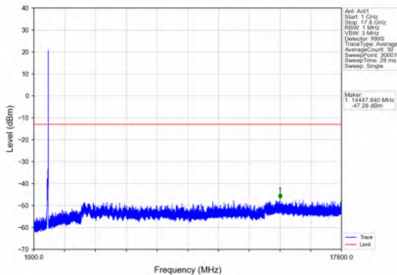
n66_30kHz_SISO_NTNV_30MHz_CP-OFDM QPSK_1765MHz_Outer_Full
