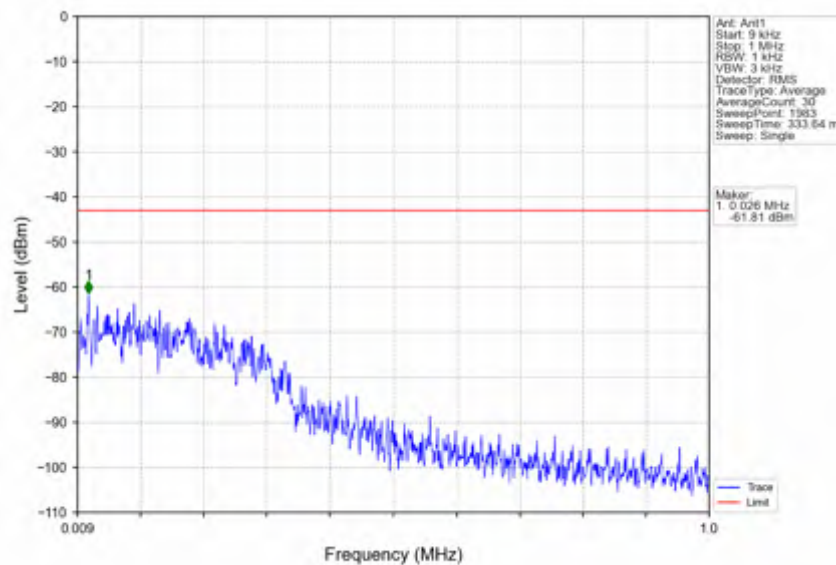
n66_30kHz_SISO_NTNV_30MHz_CP-OFDM_QPSK_1725MHz_Edge_1RB_Left
