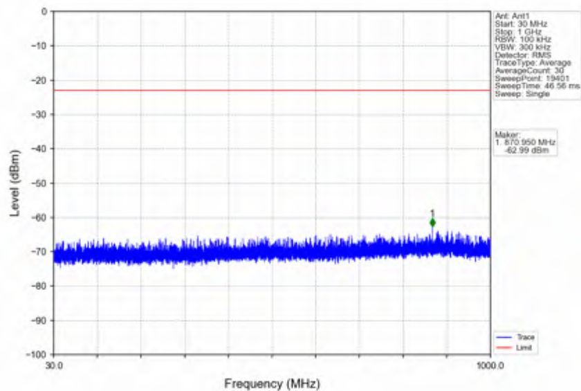
n66_30kHz_SISO_NTNV_40MHz_DFT-s-OFDM_PI/2_BPSK_1730MHz_Outer_Full
