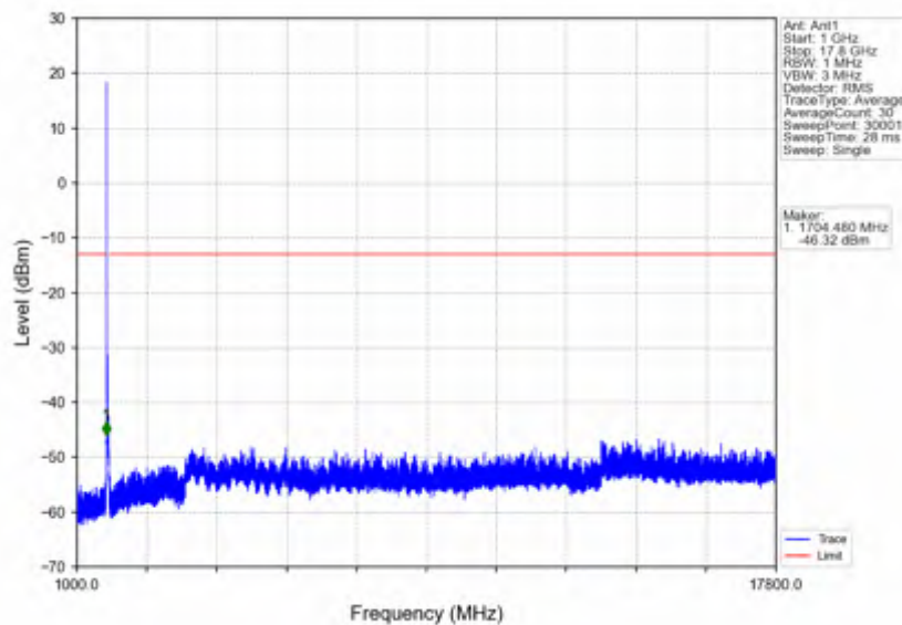
n66_30kHz_SISO_NTV_25MHz_CP-OFDM QPSK_1722.5MHz_Outer_Full
