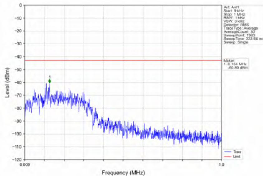
n66_30kHz_SISO_NTNV_30MHz_DFT-s-OFDM QPSK_1725MHz_Edge_1RB_Left
