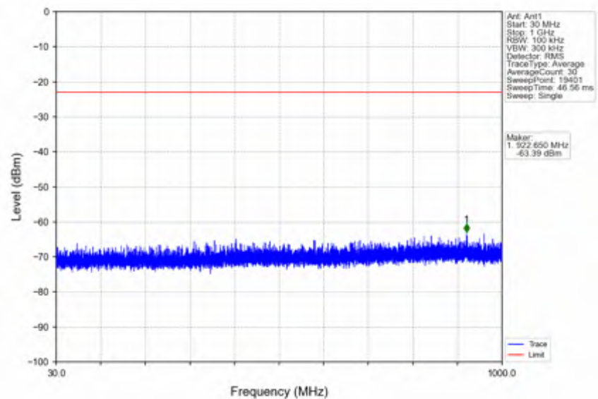
n66_30kHz_SISO_NTNV_20MHz_DFT-s-OFDM QPSK_1770MHz_Outer_Full
