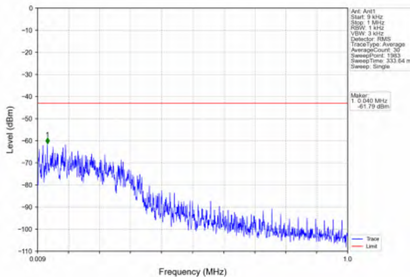
n66_30kHz_SISO_NTV_25MHz_CP-OFDM_QPSK_1722.5MHz_Edge_1RB_Left
