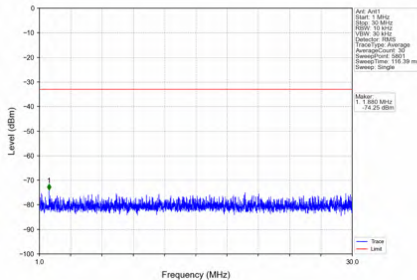
n66_30kHz_SISO_NTNV_25MHz_CP-OFDM QPSK_1767.5MHz_Inner_1RB_Right
