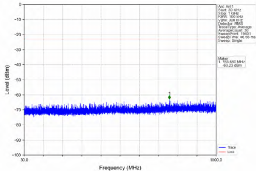
n66_30kHz_SISO_NTNV_20MHz_CP-OFDM QPSK_1770MHz_Edge_1RB_Right
