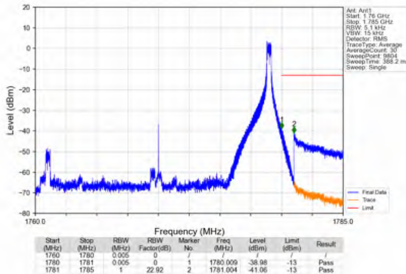
n66_30kHz_SISO_NTNV_20MHz_DFT-s-OFDM QPSK_1770MHz_Edge_1RB_Right
