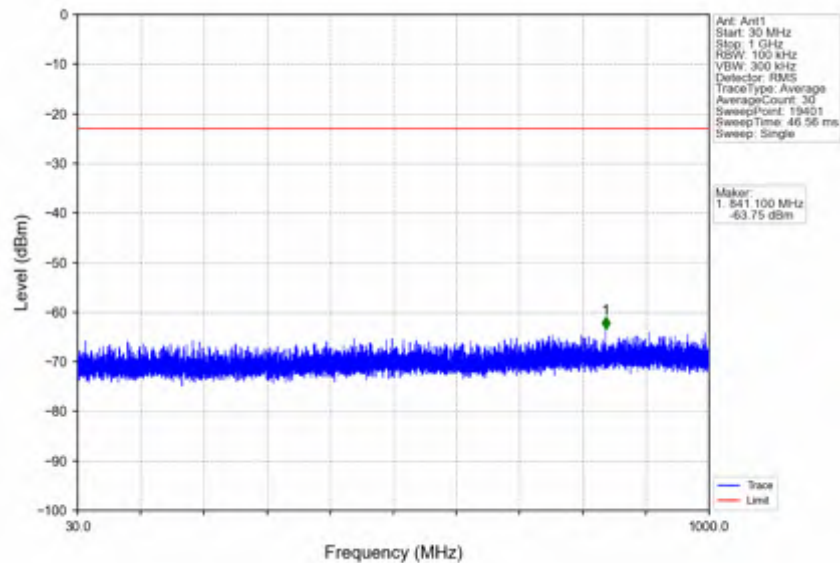
n66_30kHz_SISO_NTNV_20MHz_CP-OFDM_QPSK_1745MHz_Edge_1RB_Left
