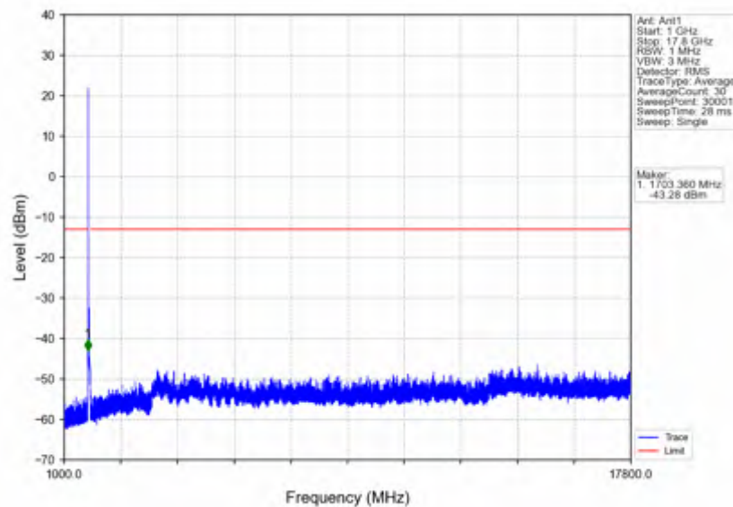
n66_30kHz_SISO_NTNV_30MHz_DFT-s-OFDM_QPSK_1725MHz_Inner_1RB_Left
