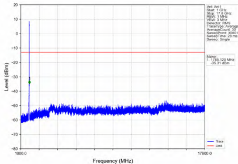
n66_30kHz_SISO_NTV_30MHz_CP-OFDM_QPSK_1765MHz_Outer_Full
