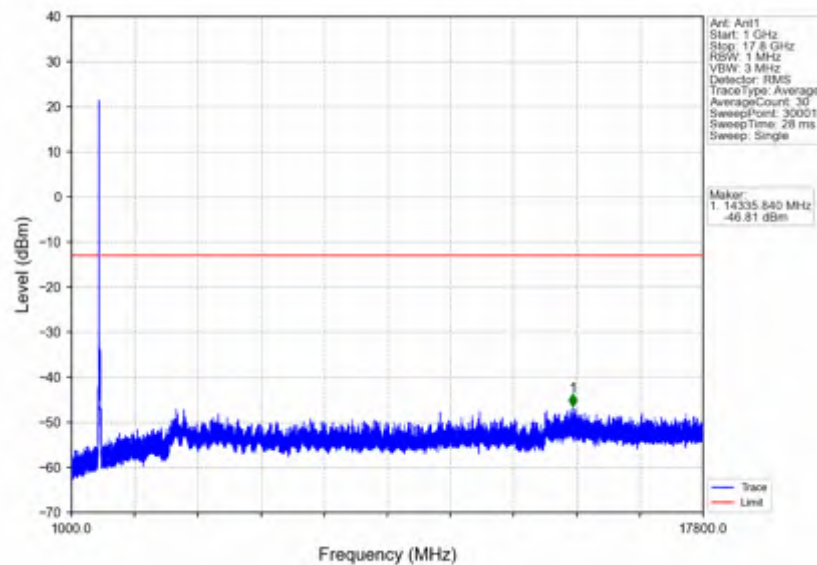
n66_30kHz_SISO_NTNV_40MHz_DFT-s-OFDM_PI/2_BPSK_1745MHz_Edge_1RB_Left
