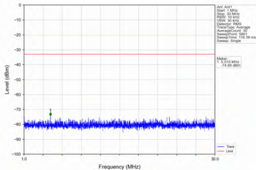
n66_30kHz_SISO_NTNV_30MHz_DFT-s-OFDM_PI/2_BPSK_1725MHz_Outer_Full
