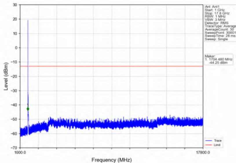
n66_30kHz_SISO_NTNV_30MHz_CP-OFDM QPSK_1725MHz_Outer_Full
