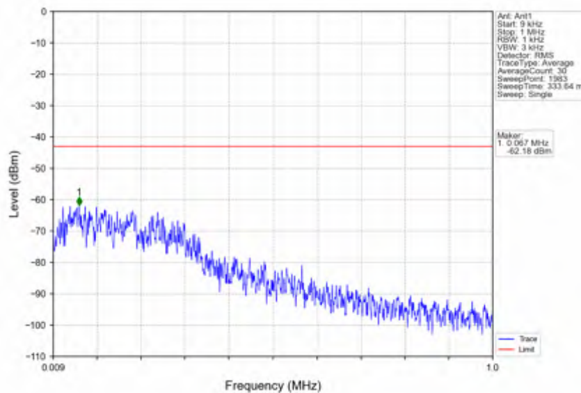
n66_30kHz_SISO_NTNV_30MHz_CP-OFDM_QPSK_1765MHz_Inner_1RB_Right
