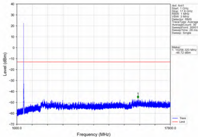
n66_30kHz_SISO_NTNV_25MHz_DFT-s-OFDM PI/2 BPSK_1745MHz_Edge_1RB_Left
