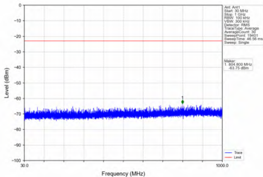
n66_30kHz_SISO_NTNV_30MHz_CP-OFDM_QPSK_1765MHz_Inner_1RB_Right
