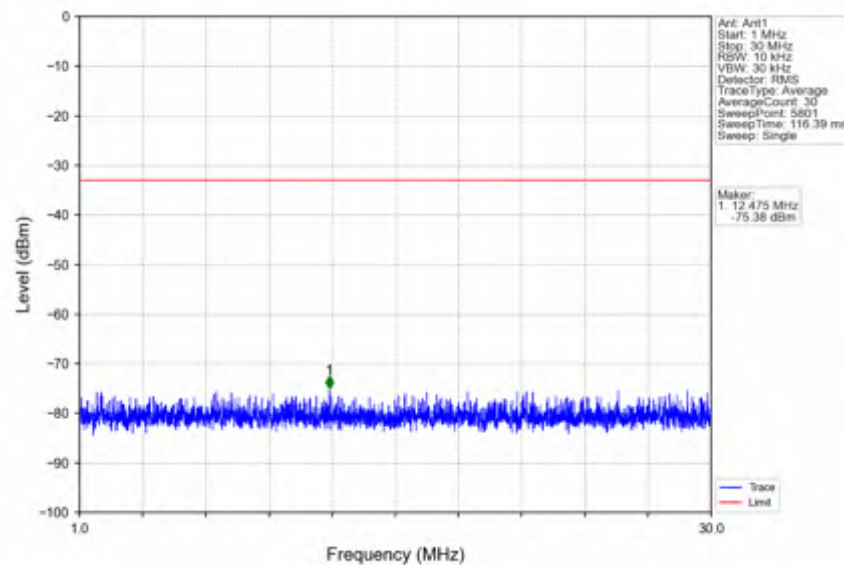
n66_30kHz_SISO_NTNV_40MHz_DFT-s-OFDM PI/2 BPSK_1745MHz_Edge_1RB_Left
