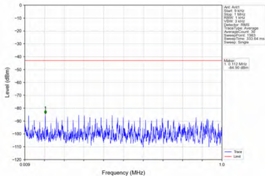
n66_30kHz_SISO_NTNV_40MHz_DFT-s-OFDM_PI/2_BPSK_1730MHz_Outer_Full
