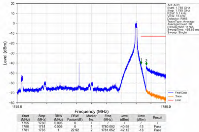
n66_30kHz_SISO_NTNV_25MHz_CP-OFDM QPSK_1767.5MHz_Edge_1RB_Right
