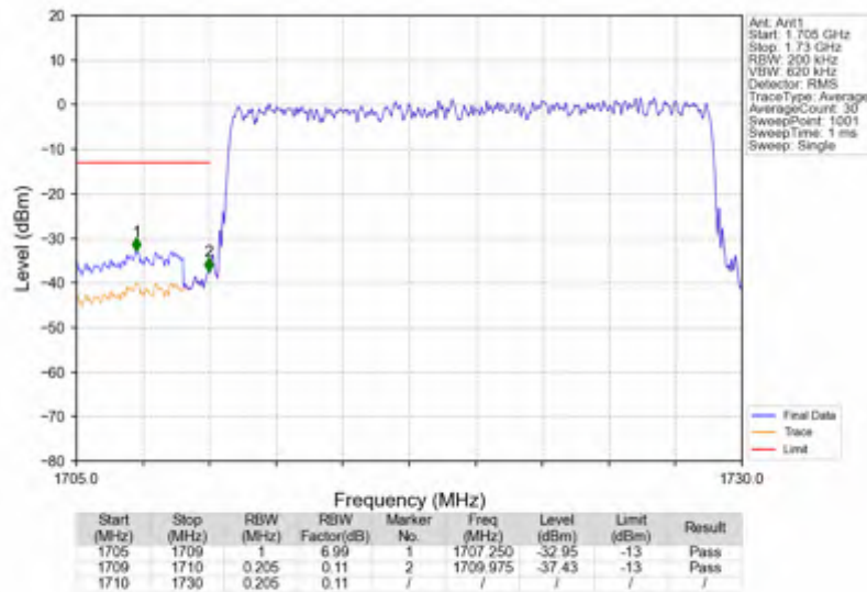
n66_30kHz_SISO_NTNV_20MHz_DFT-s-OFDM QPSK_1720MHz_Outer_Full
