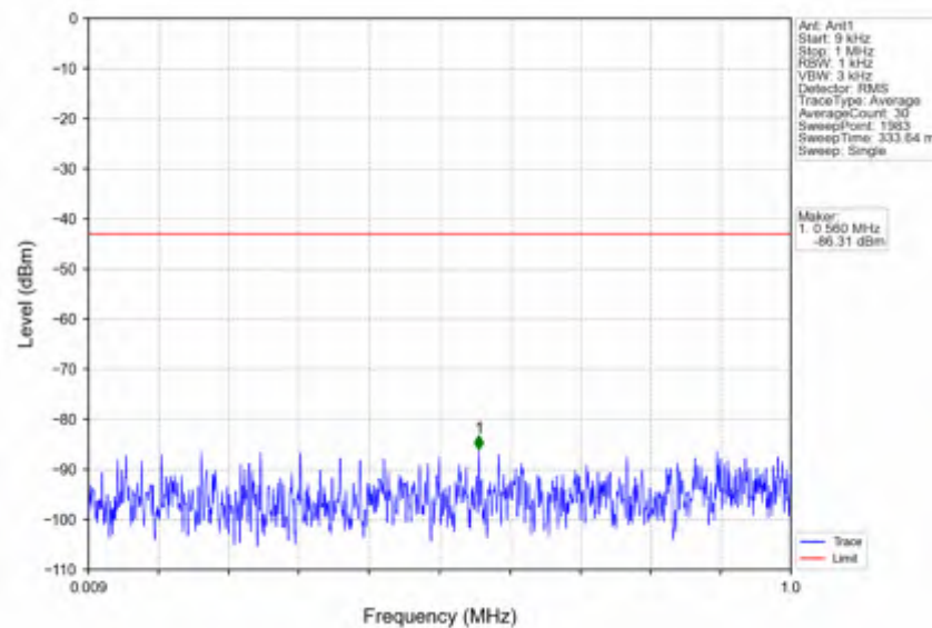
n66_30kHz_SISO_NTNV_20MHz_DFT-s-OFDM QPSK_1720MHz_Outer_Full
