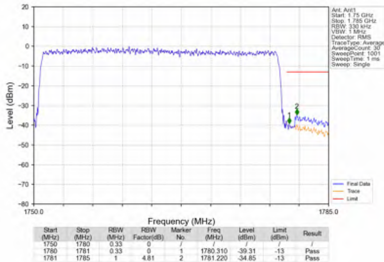
n66_30kHz_SISO_NTNV_30MHz_CP-OFDM QPSK_1765MHz_Outer_Full
