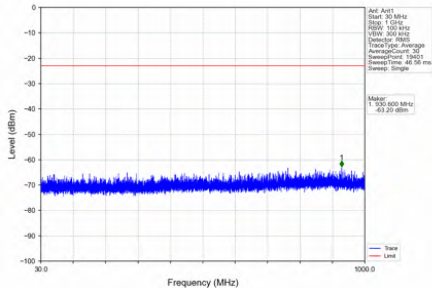
n66_30kHz_SISO_NTNV_20MHz_DFT-s-OFDM_QPSK_1770MHz_Edge_1RB_Right
