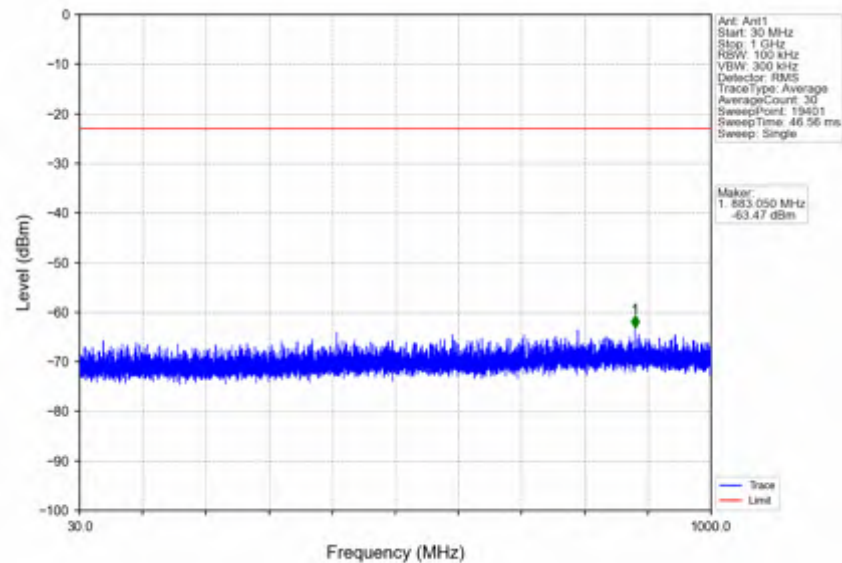
n66_30kHz_SISO_NTNV_25MHz_CP-OFDM_QPSK_1722.5MHz_Outer_Full
