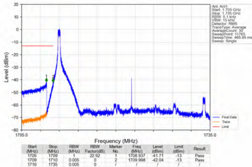
n66_30kHz_SISO_NTV_25MHz_CP-OFDM_QPSK_1722.5MHz_Edge_1RB_Left
