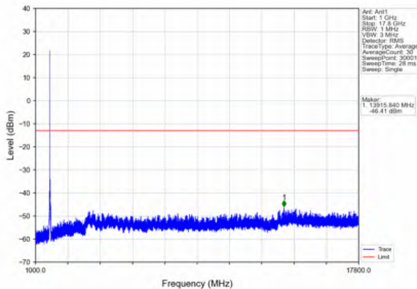
n66_30kHz_SISO_NTNV_25MHz_DFT-s-OFDM QPSK_1767.5MHz_Edge_1RB_Right
