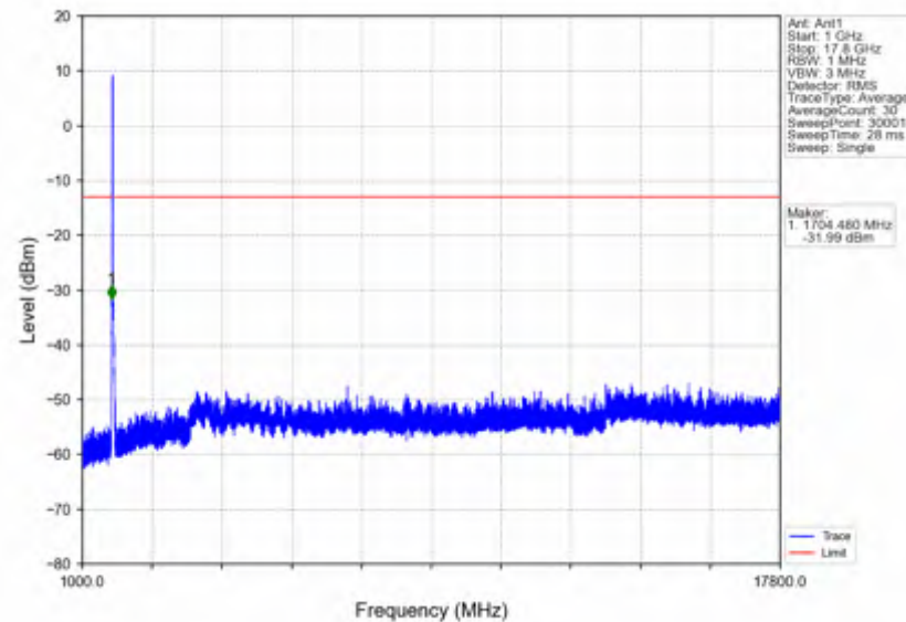
n66_30kHz_SISO_NTNV_25MHz_CP-OFDM_QPSK_1722.5MHz_Outer_Full
