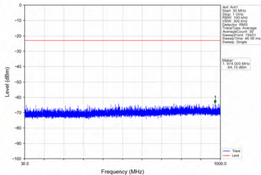
n66_30kHz_SISO_NTNV_40MHz_DFT-s-OFDM QPSK_1745MHz_Edge_1RB_Left
