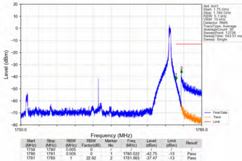
n66_30kHz_SISO_NTNV_30MHz_DFT-s-OFDM QPSK_1765MHz_Edge_1RB_Right
