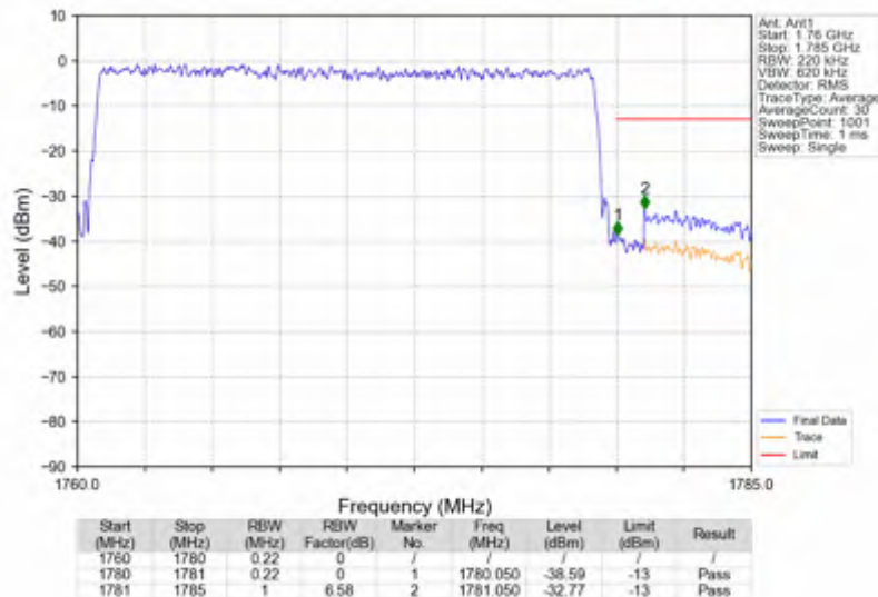
n66_30kHz_SISO_NTNV_20MHz_CP-OFDM QPSK_1770MHz_Outer_Full
