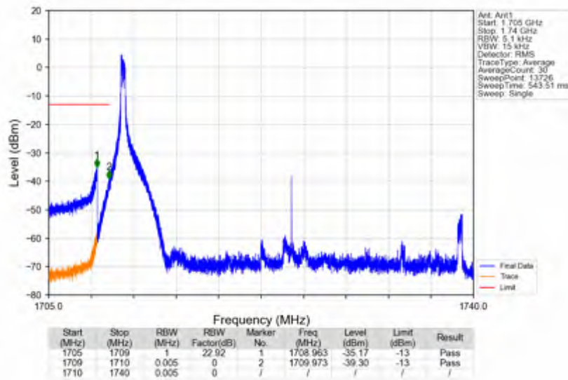
n66_30kHz_SISO_NTNV_30MHz_DFT-s-OFDM_PI/2_BPSK_1725MHz_Edge_1RB_Left
