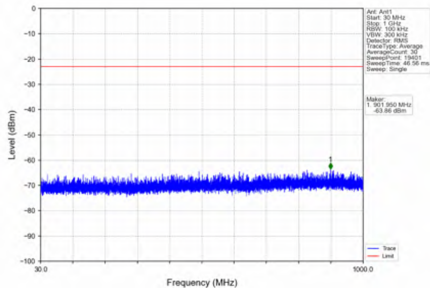
n66_30kHz_SISO_NTNV_30MHz_CP-OFDM_QPSK_1745MHz_Edge_1RB_Left
