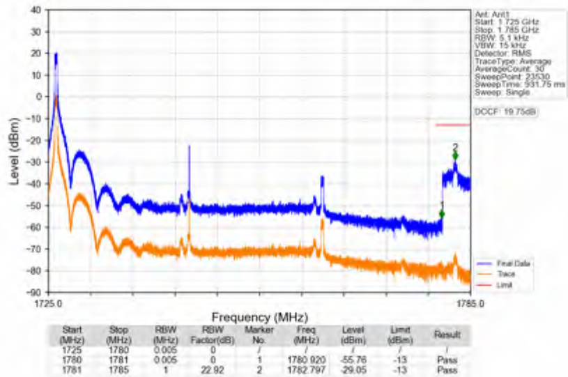
n66_30kHz_SISO_NTNV_40MHz_CP-OFDM QPSK_1745MHz_Edge_1RB_Left
