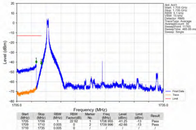
n66_30kHz_SISO_NTNV_25MHz_DFT-s-OFDM_QPSK_1722.5MHz_Inner_1RB_Left
