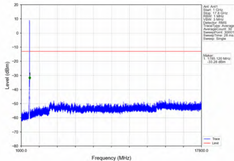
n66_30kHz_SISO_NTNV_25MHz_CP-OFDM QPSK_1767.5MHz_Outer_Full
