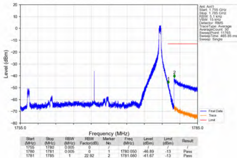
n66_30kHz_SISO_NTNV_25MHz_CP-OFDM QPSK_1767.5MHz_Inner_1RB_Right
