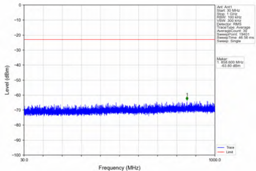
n66_30kHz_SISO_NTNV_30MHz_DFT-s-OFDM_QPSK_1725MHz_Outer_Full
