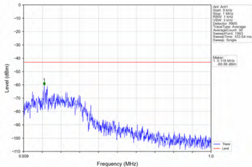
n66_30kHz_SISO_NTNV_25MHz_DFT-s-OFDM QPSK_1767.5MHz_Edge_1RB_Right
