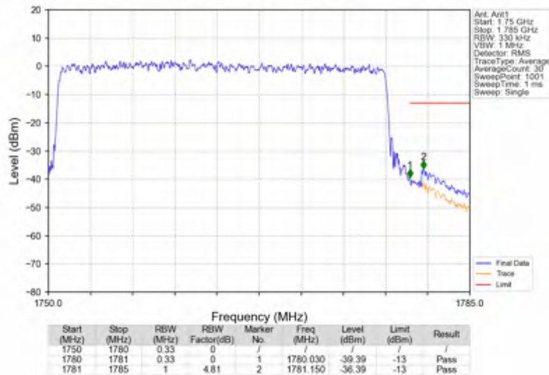
n66_30kHz_SISO_NTNV_30MHz_DFT-s-OFDM PI/2 BPSK_1765MHz_Outer_Full
