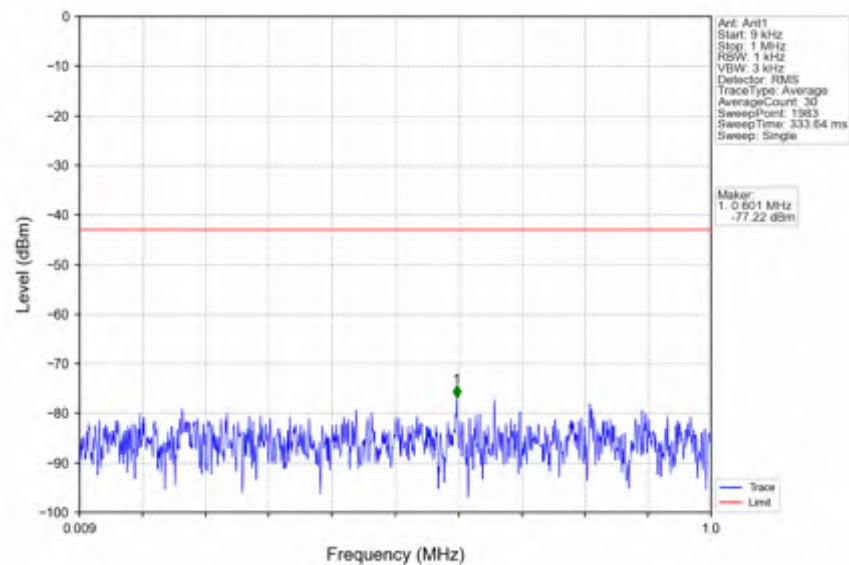
n66_30kHz_SISO_NTNV_20MHz_CP-OFDM_QPSK_1770MHz_Outer_Full
