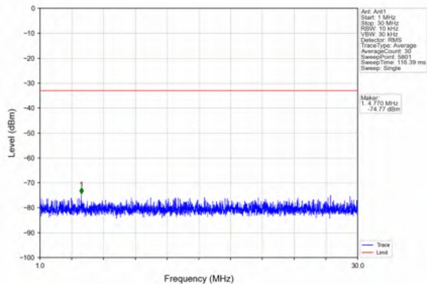
n66_30kHz_SISO_NTNV_40MHz_CP-OFDM_QPSK_1730MHz_Outer_Full
