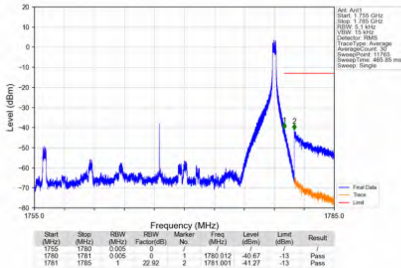
n66_30kHz_SISO_NTNV_25MHz_DFT-s-OFDM QPSK_1767.5MHz_Edge_1RB_Right
