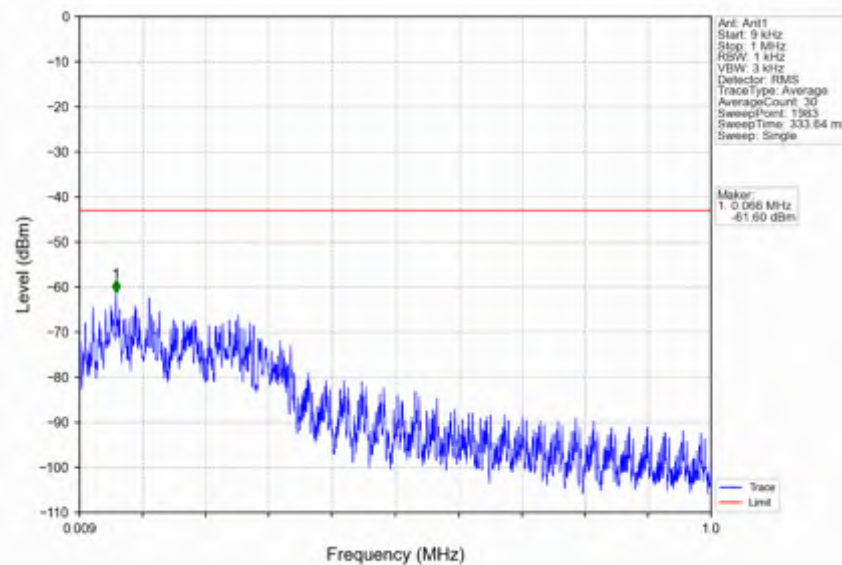
n66_30kHz_SISO_NTNV_25MHz_CP-OFDM QPSK_1745MHz_Edge_1RB_Left
