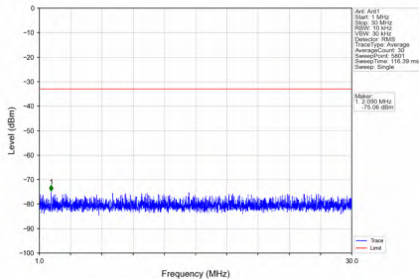
n66_30kHz_SISO_NTNV_25MHz_CP-OFDM QPSK_1767.5MHz_Edge_1RB_Right
