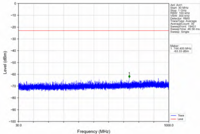
n66_30kHz_SISO_NTNV_30MHz_CP-OFDM QPSK_1725MHz_Edge_1RB_Left
