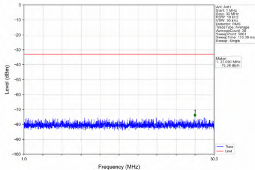
n66_30kHz_SISO_NTNV_30MHz_DFT-s-OFDM QPSK_1765MHz_Outer_Full
