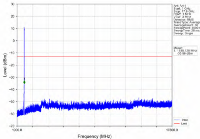
n66_30kHz_SISO_NTNV_25MHz_DFT-s-OFDM QPSK_1767.5MHz_Inner_1RB_Right
