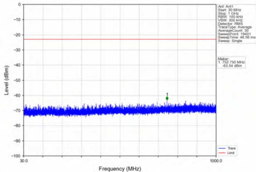
n66_30kHz_SISO_NTNV_40MHz_CP-OFDM_QPSK_1730MHz_Edge_1RB_Left
