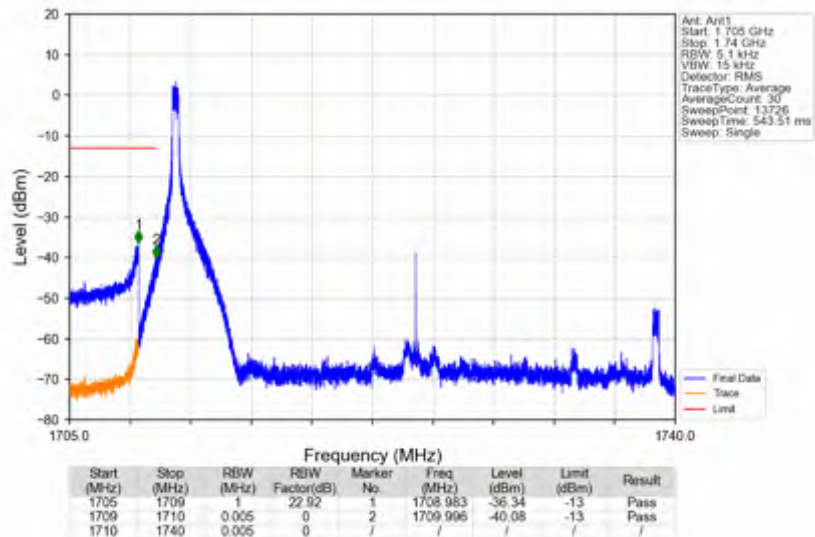
n66_30kHz_SISO_NTNV_30MHz_DFT-s-OFDM QPSK_1725MHz_Edge_1RB_Left
