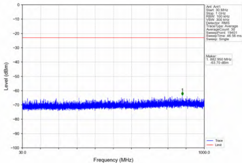
n66_30kHz_SISO_NTV_30MHz_CP-OFDM_QPSK_1725MHz_Outer_Full
