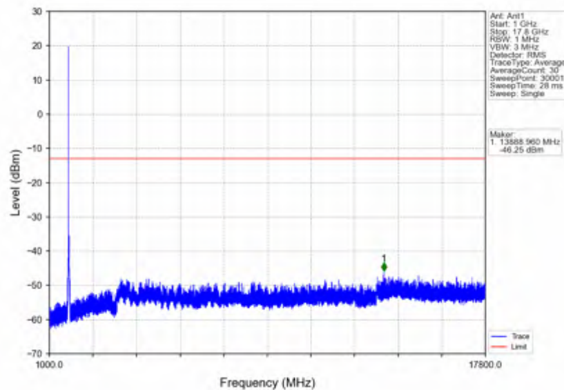
n66_30kHz_SISO_NTNV_30MHz_CP-OFDM_QPSK_1745MHz_Edge_1RB_Left
