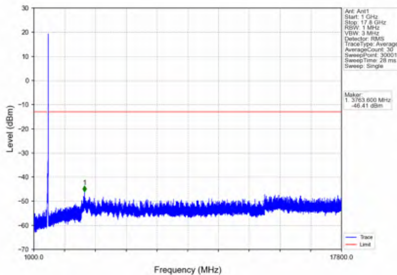
n66_30kHz_SISO_NTNV_25MHz_CP-OFDM QPSK_1767.5MHz_Outer_Full
