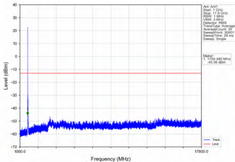
n66_30kHz_SISO_NTNV_40MHz_DFT-s-OFDM PI/2 BPSK_1745MHz_Edge_1RB_Left
