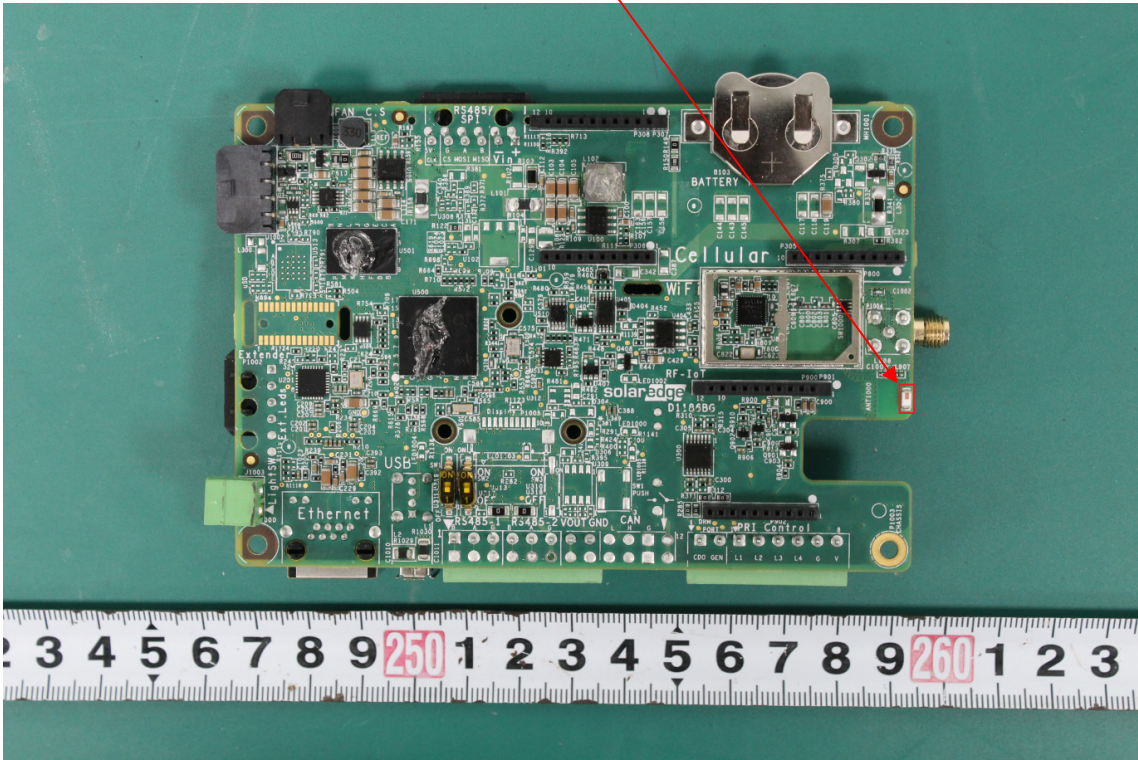
Chip Antenna
