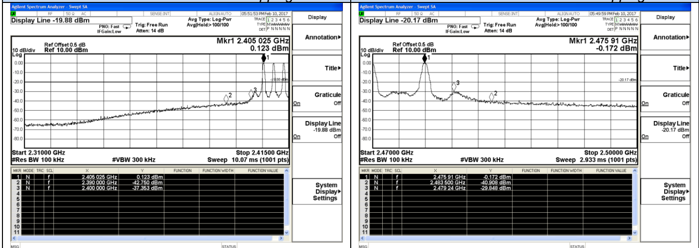
Channel 1 / 2405 MHz – Hopping
